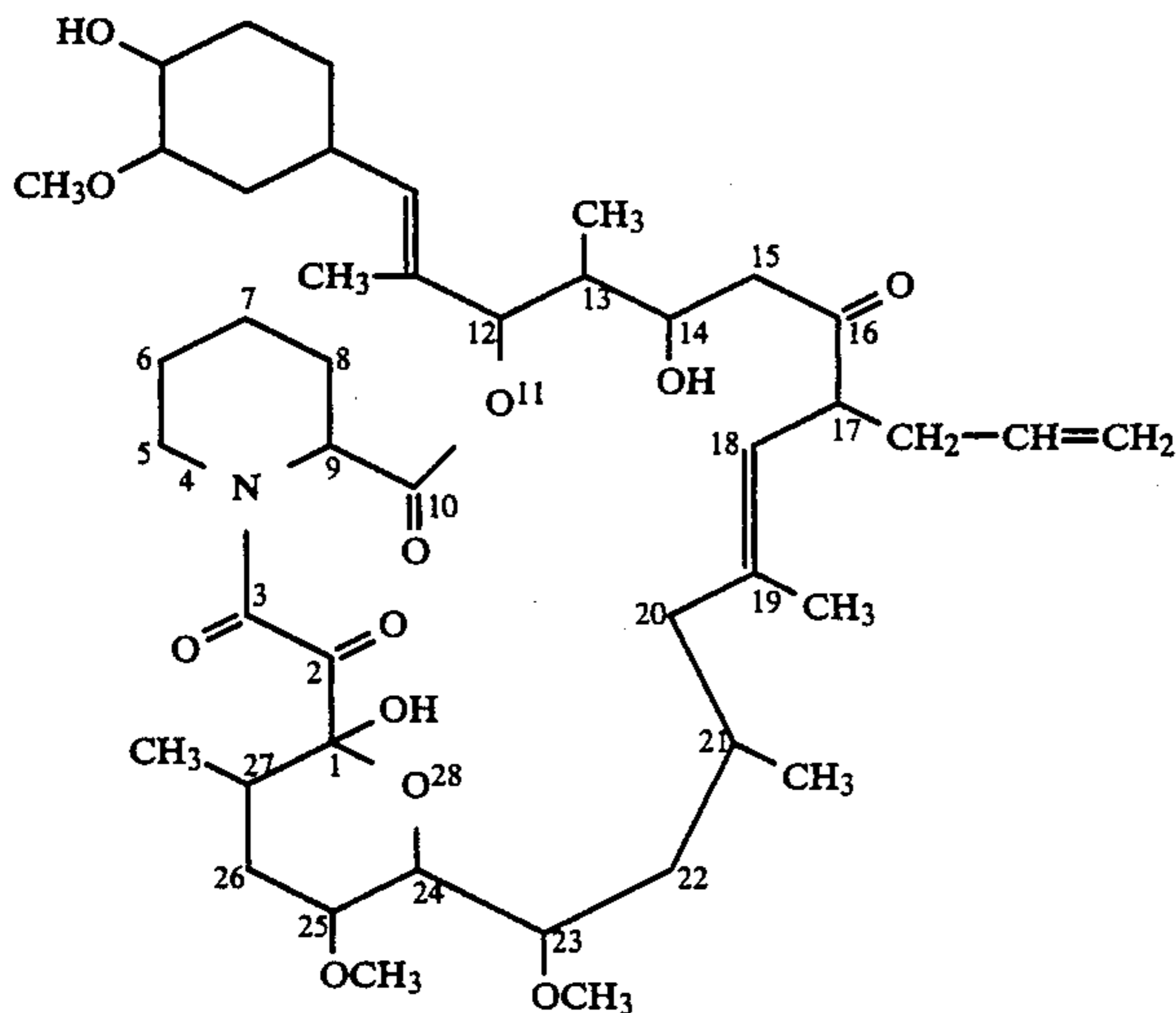
17-Allyl-1,14-dihydroxy-12-[2-(4-hydroxy-3- methoxycyclohexyl)-1-methylvinyl]-23,25- dimethoxy-13,19,21,27-tetramethyl-11,28-dioxa- 4-azatricyclo[22.3.1.0 4,9 ]octacos-18-ene- 2,3,10,16-tetraone
