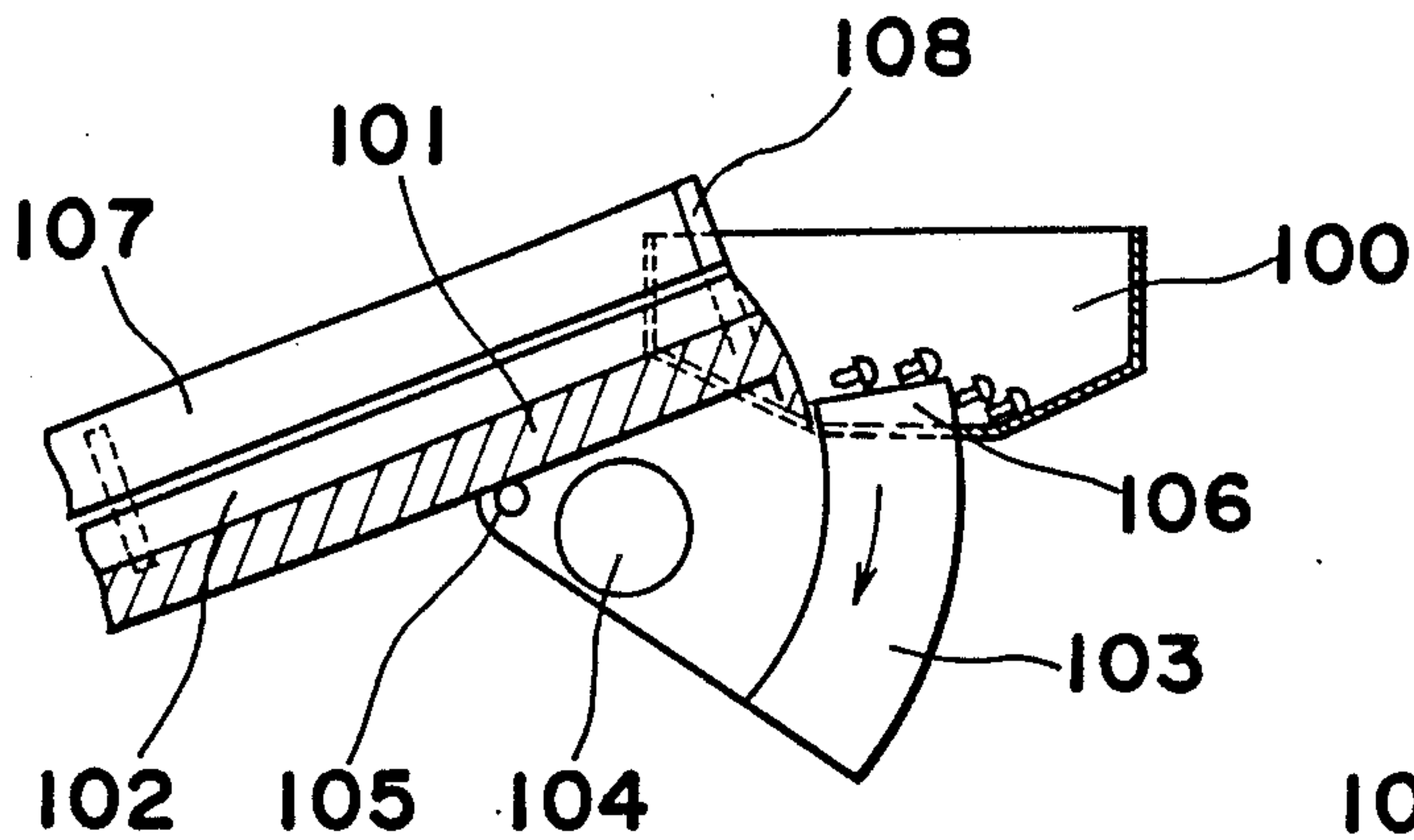
Fig. 15 Prior Art
