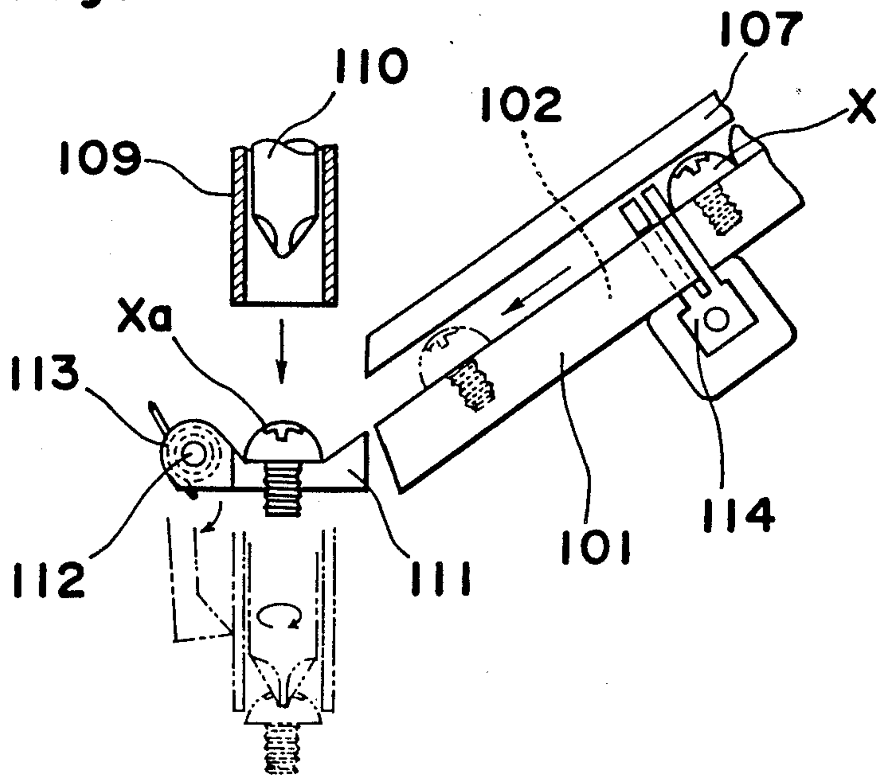
Fig. 17 Prior Art
