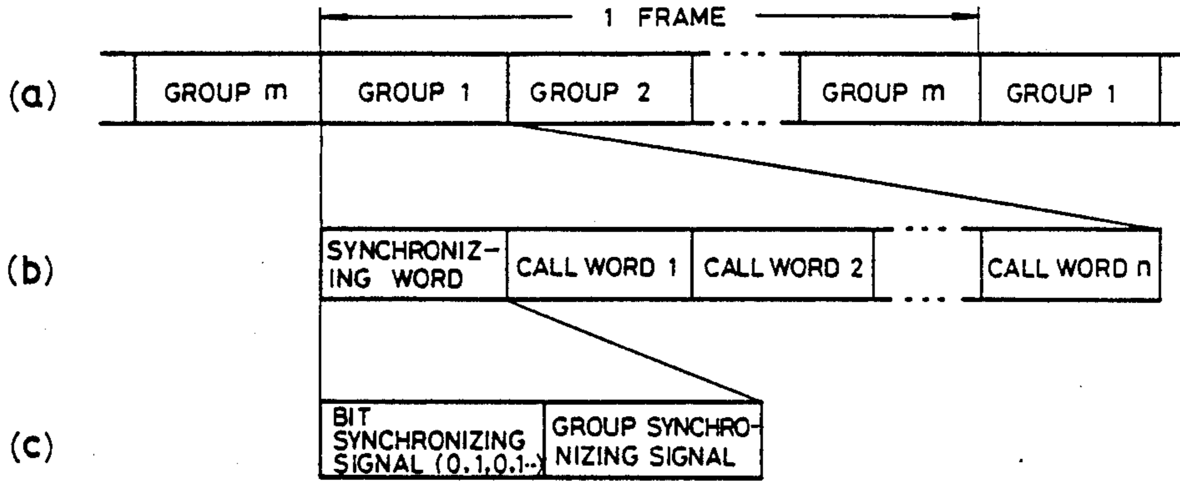
FIG. 1 PRIOR ART
