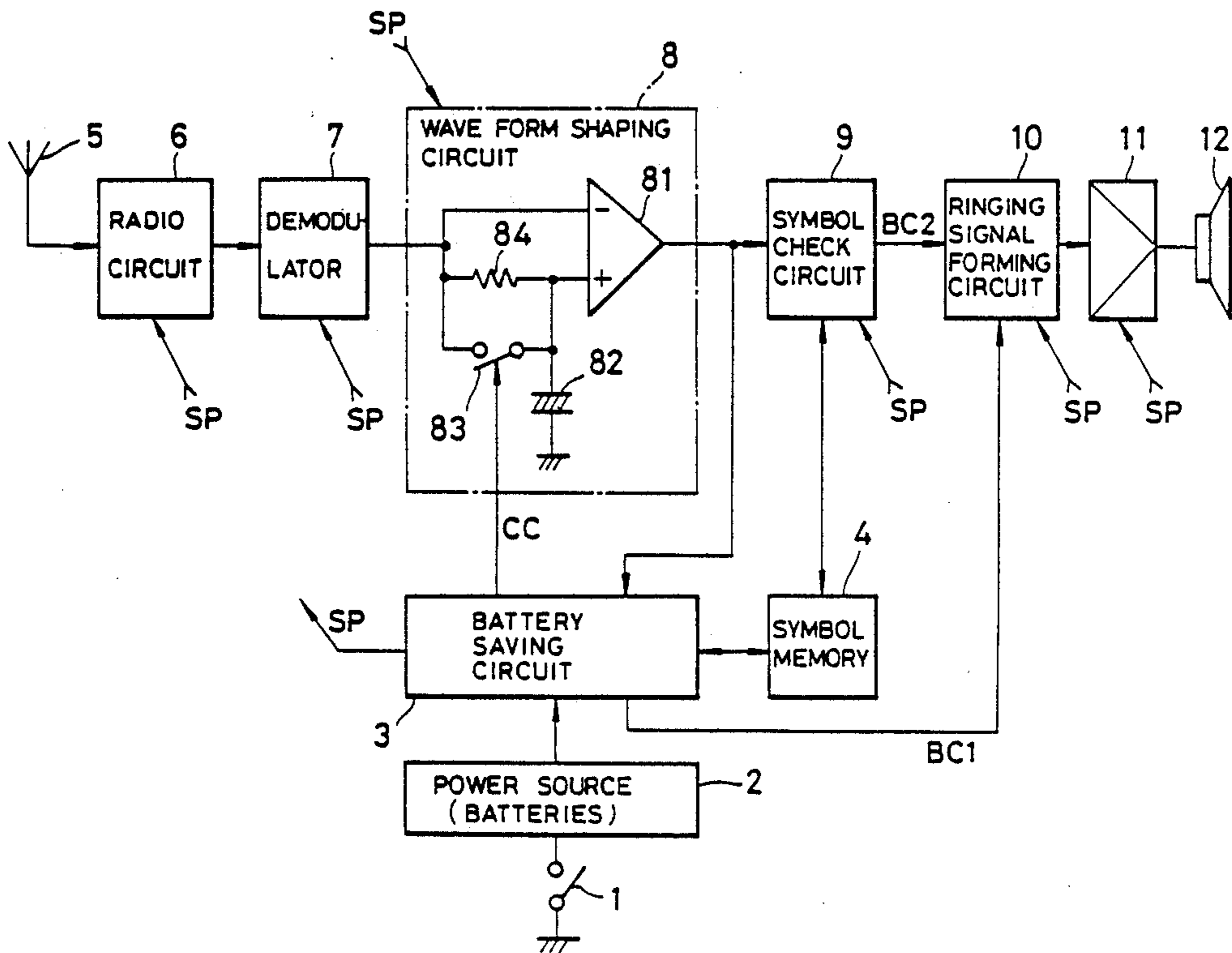
FIG. 2 PRIOR ART
