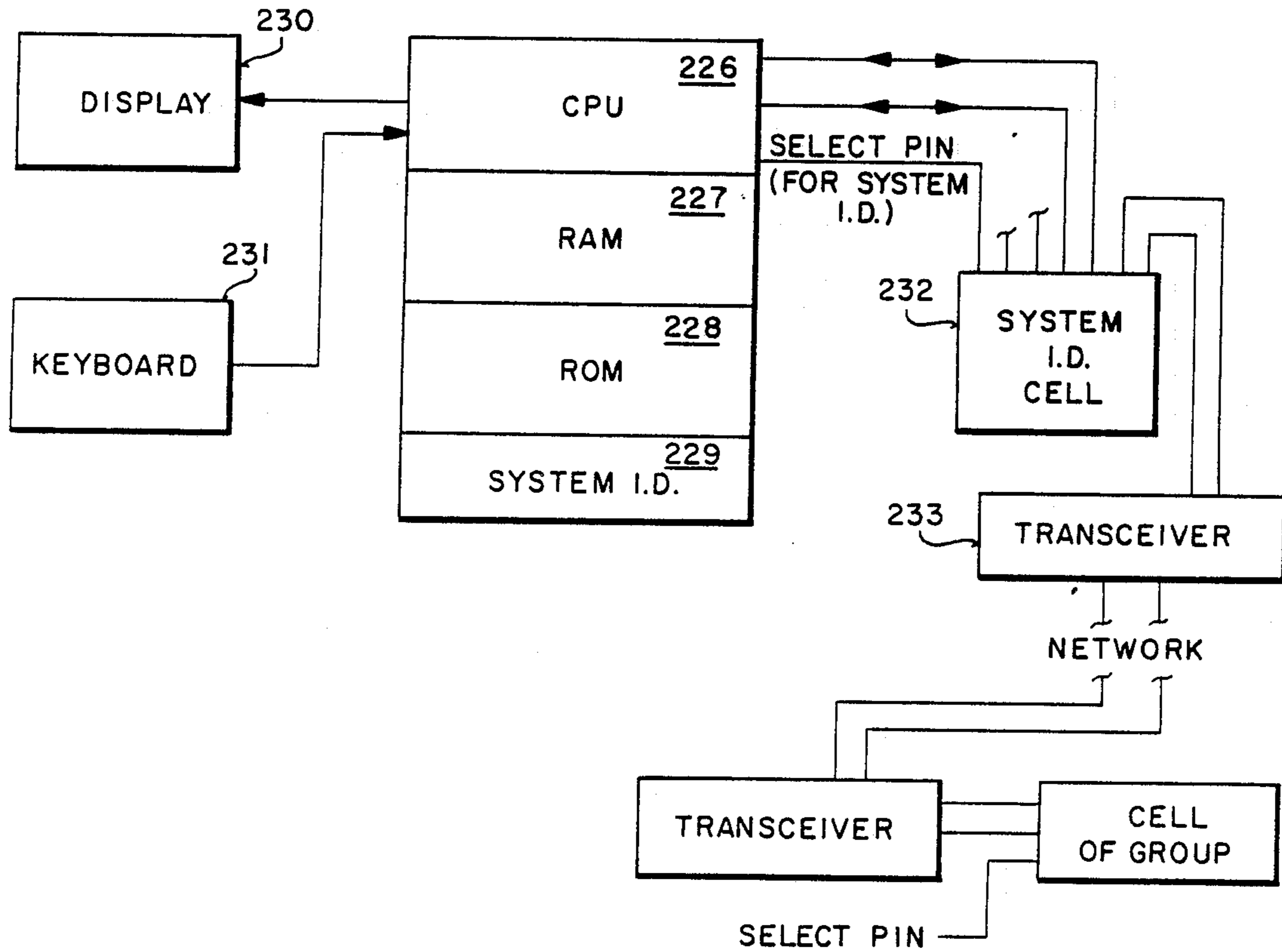
FIG 28 GROUPING DEVICE
