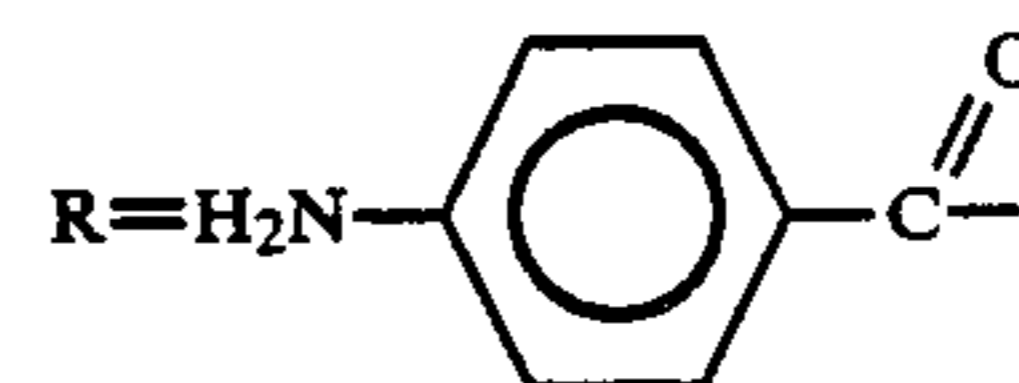
p-amino benzoyl
