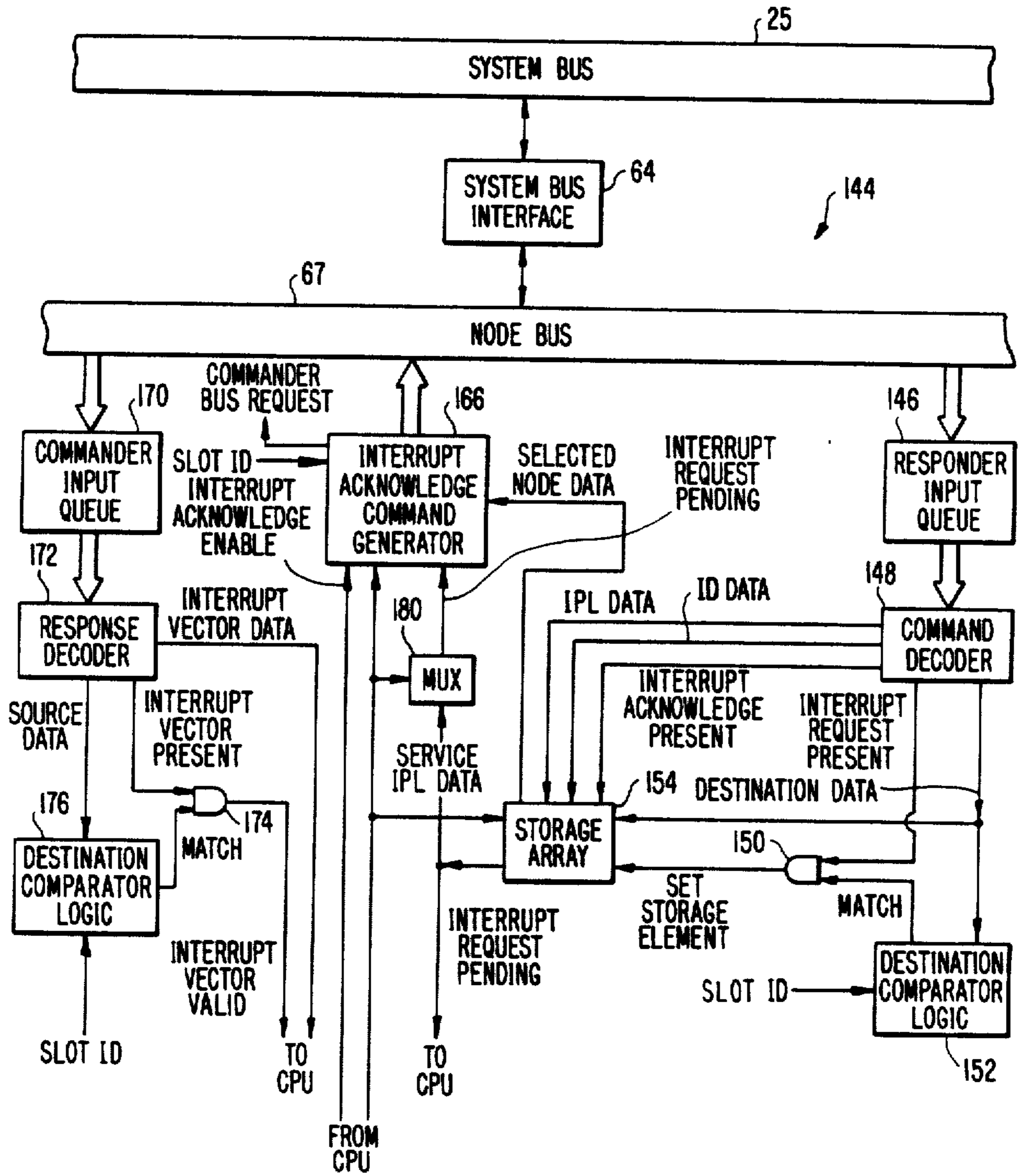
FIG. 7 INTERRUPT SERVICING NODE
