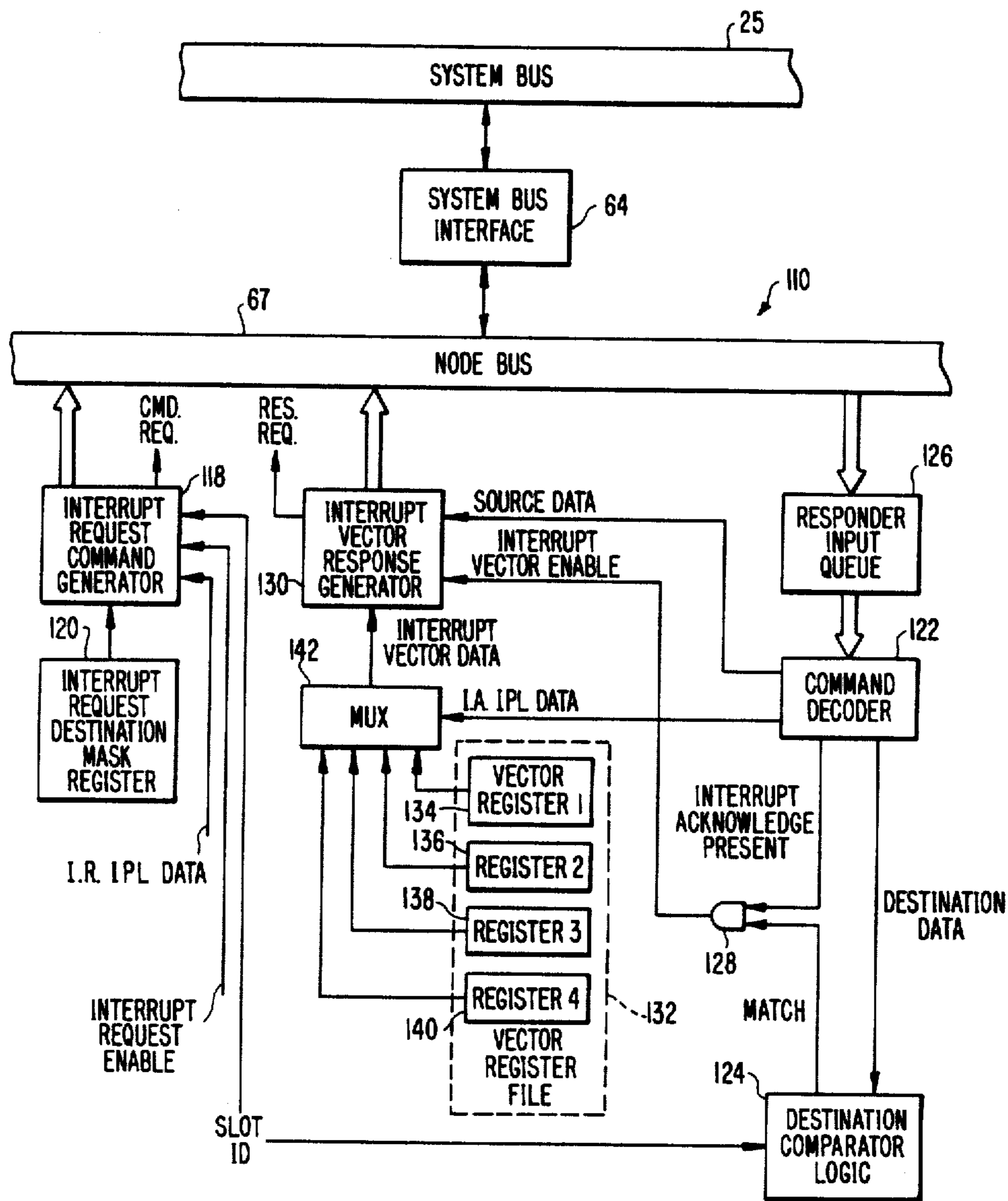
FIG. 6. INTERRUPTING NODE
