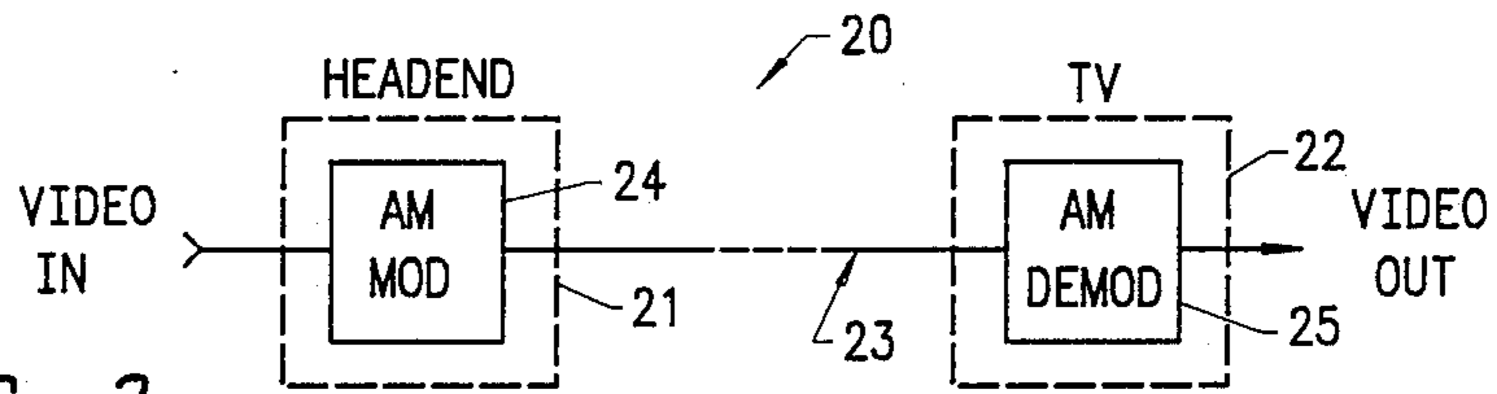
FIG. 3 PRIOR ART
