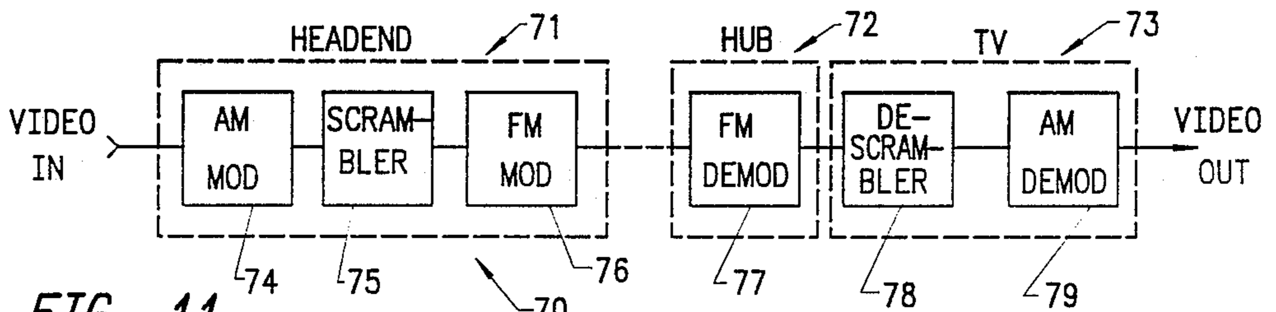
FIG. 10 PRIOR ART
