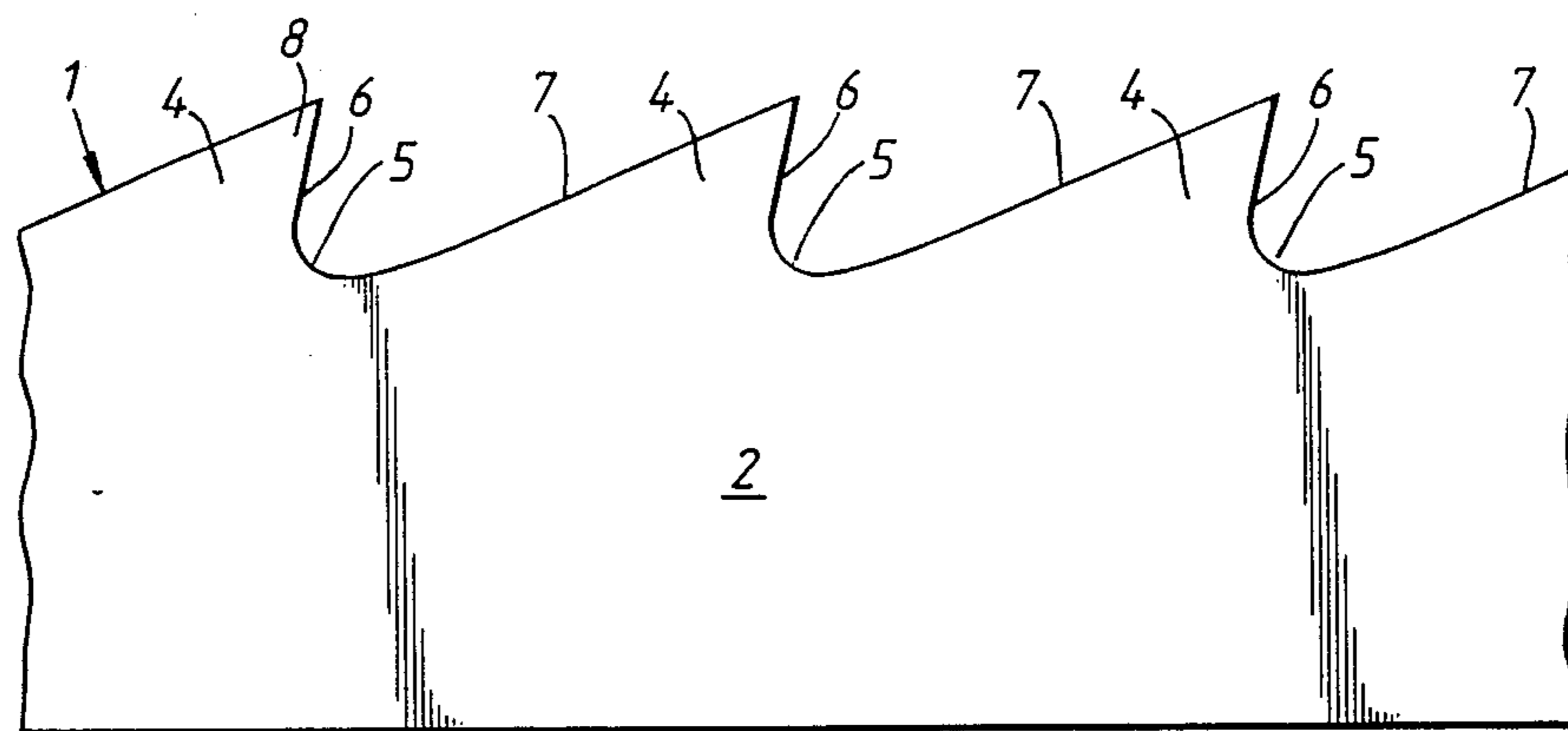
Fig. 1. PRIOR ART
