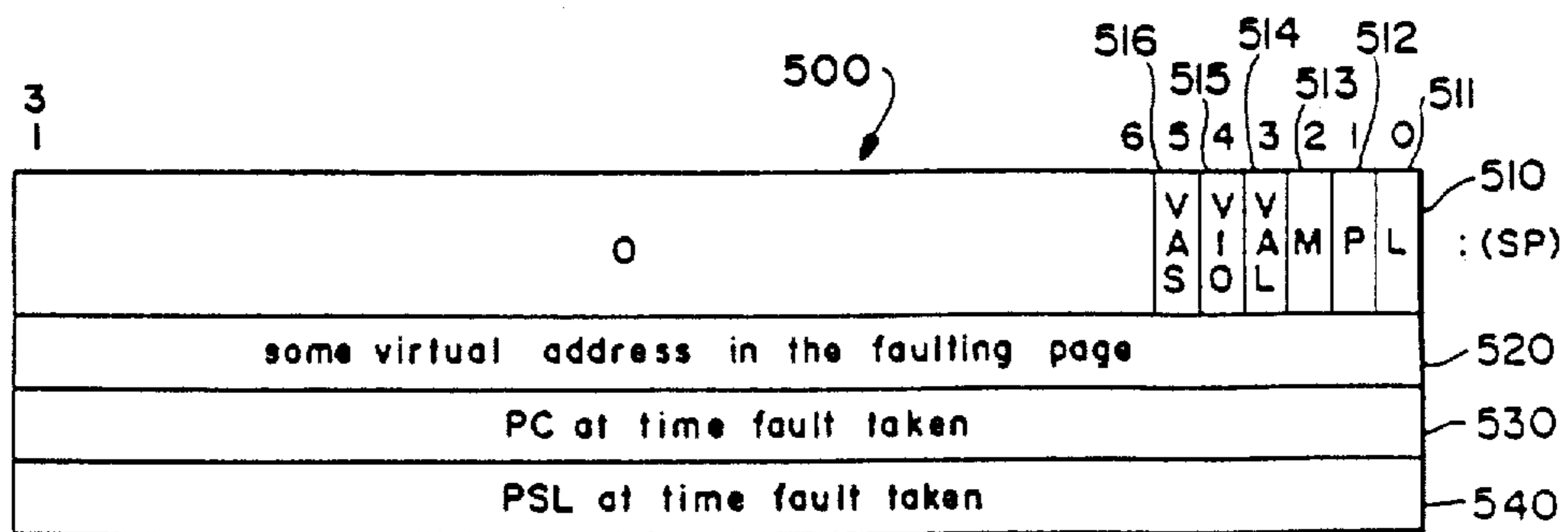
Memory Management Fault Stack Frame
