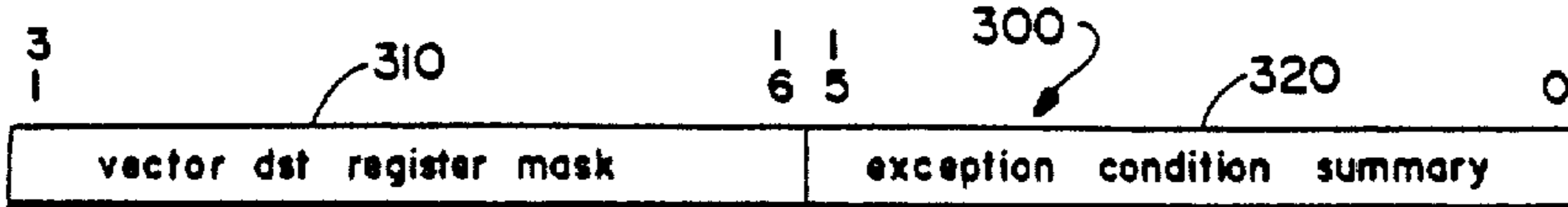
Vector Arithmetic Exception Register (VAER)
