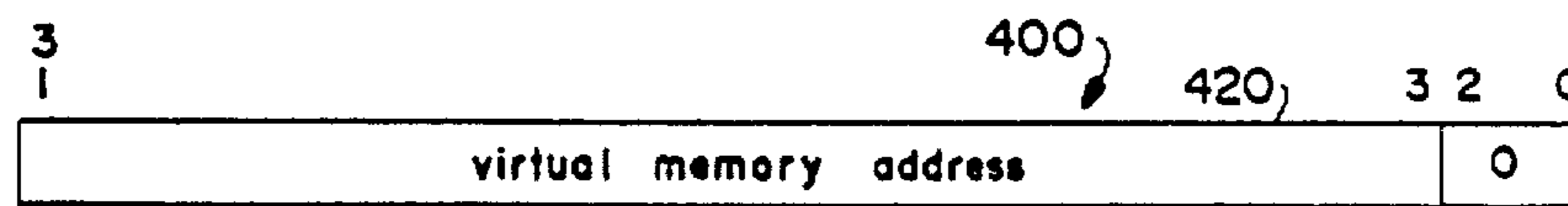
Vector State Address Register (VSAR)
