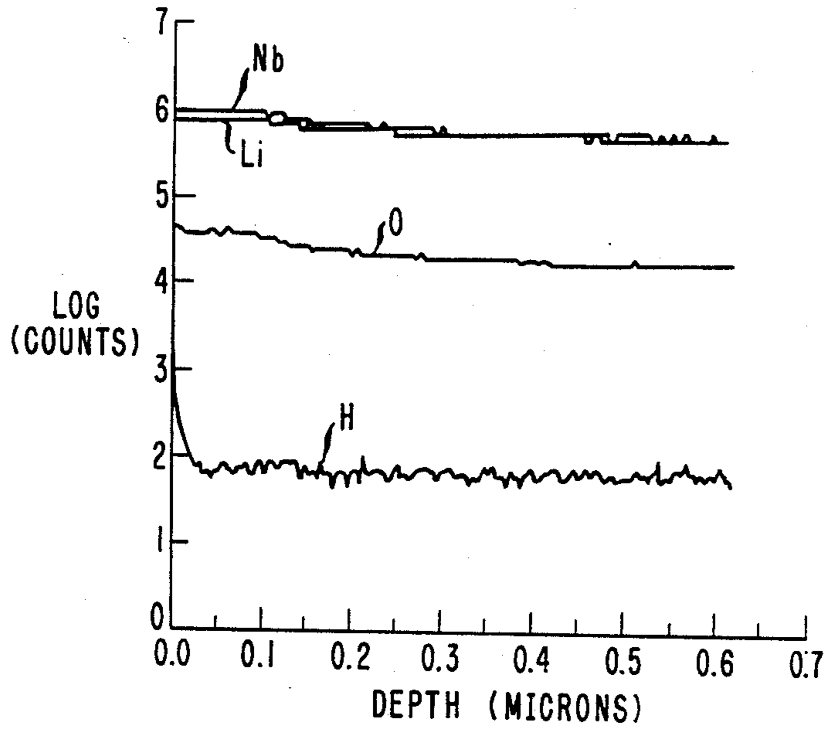
FIG. 3 UNTREATED SUBSTRATE
