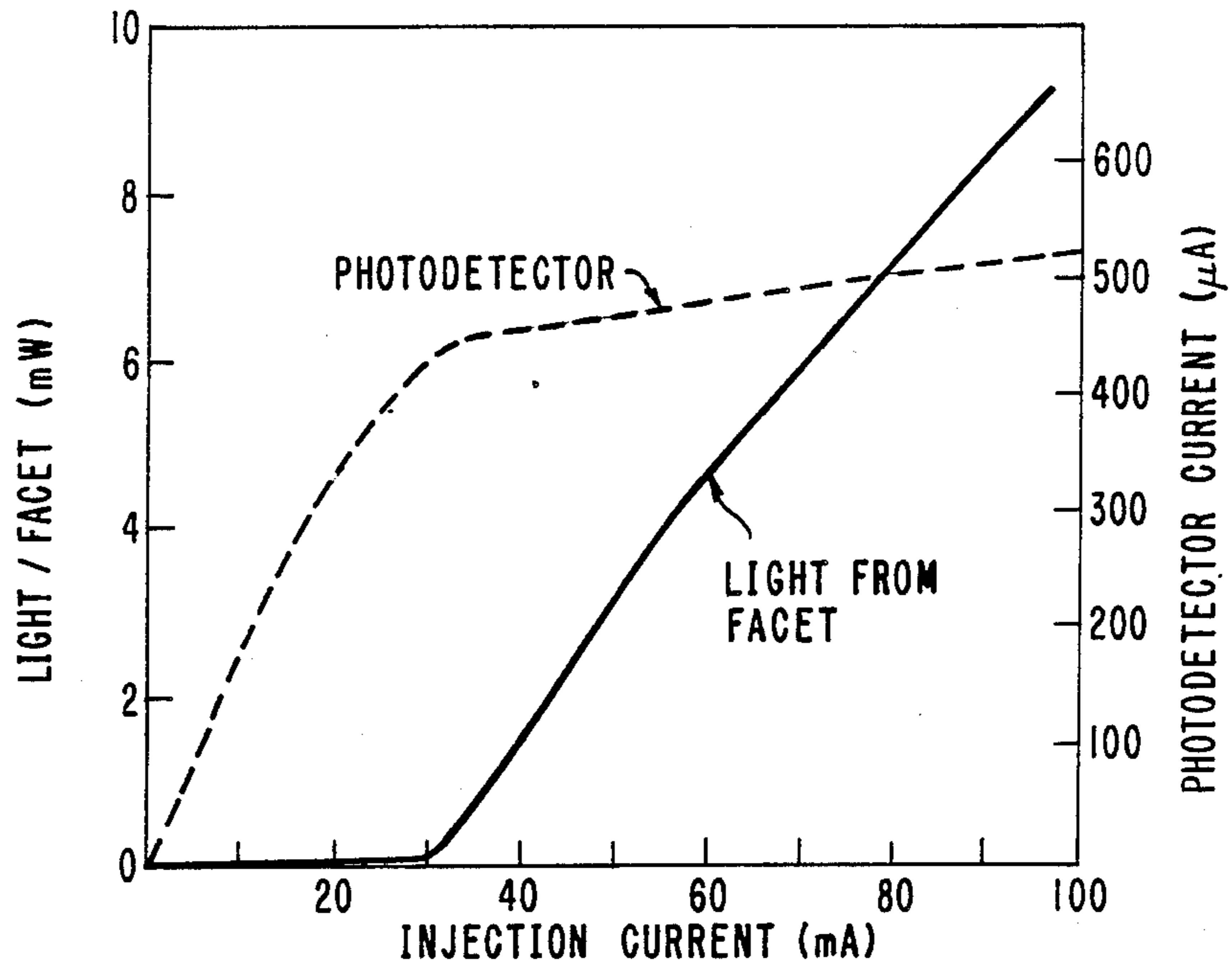
PERFORMANCE CHARACTERISTICS OF THE INTEGRATED LASER - PHOTODETECTOR
