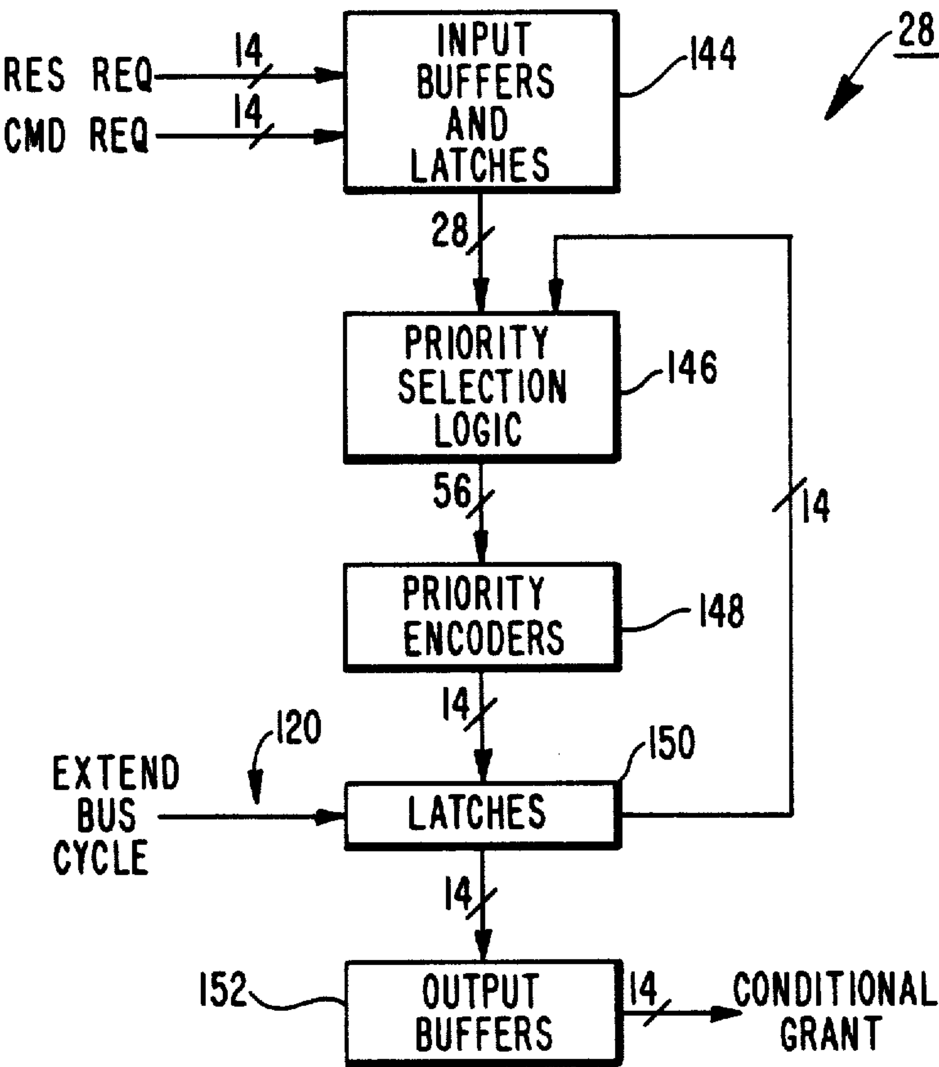
ARBITER BLOCK DIAGRAM
