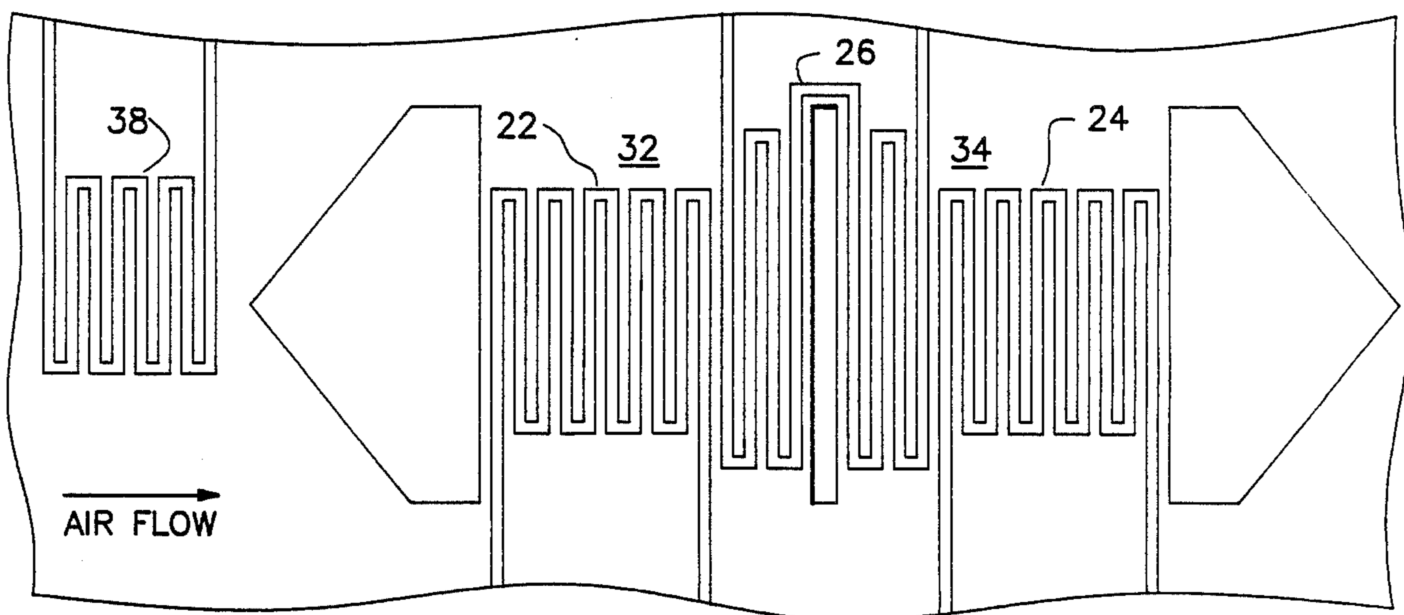
Fig. 2 (PRIOR ART)
