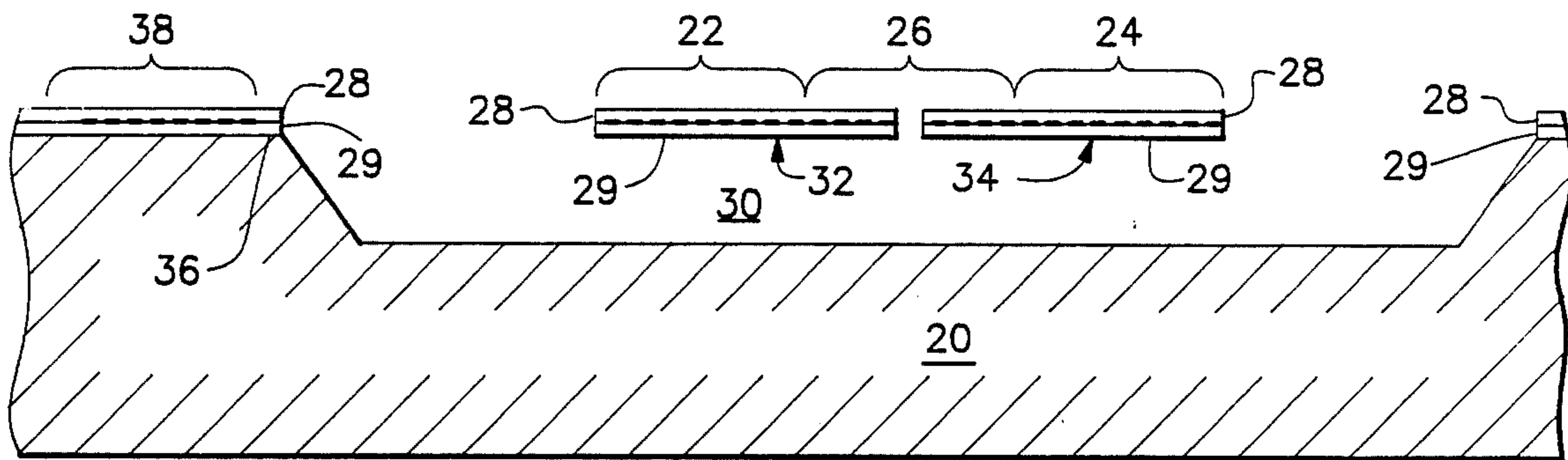
Fig. 1 (PRIOR ART)
