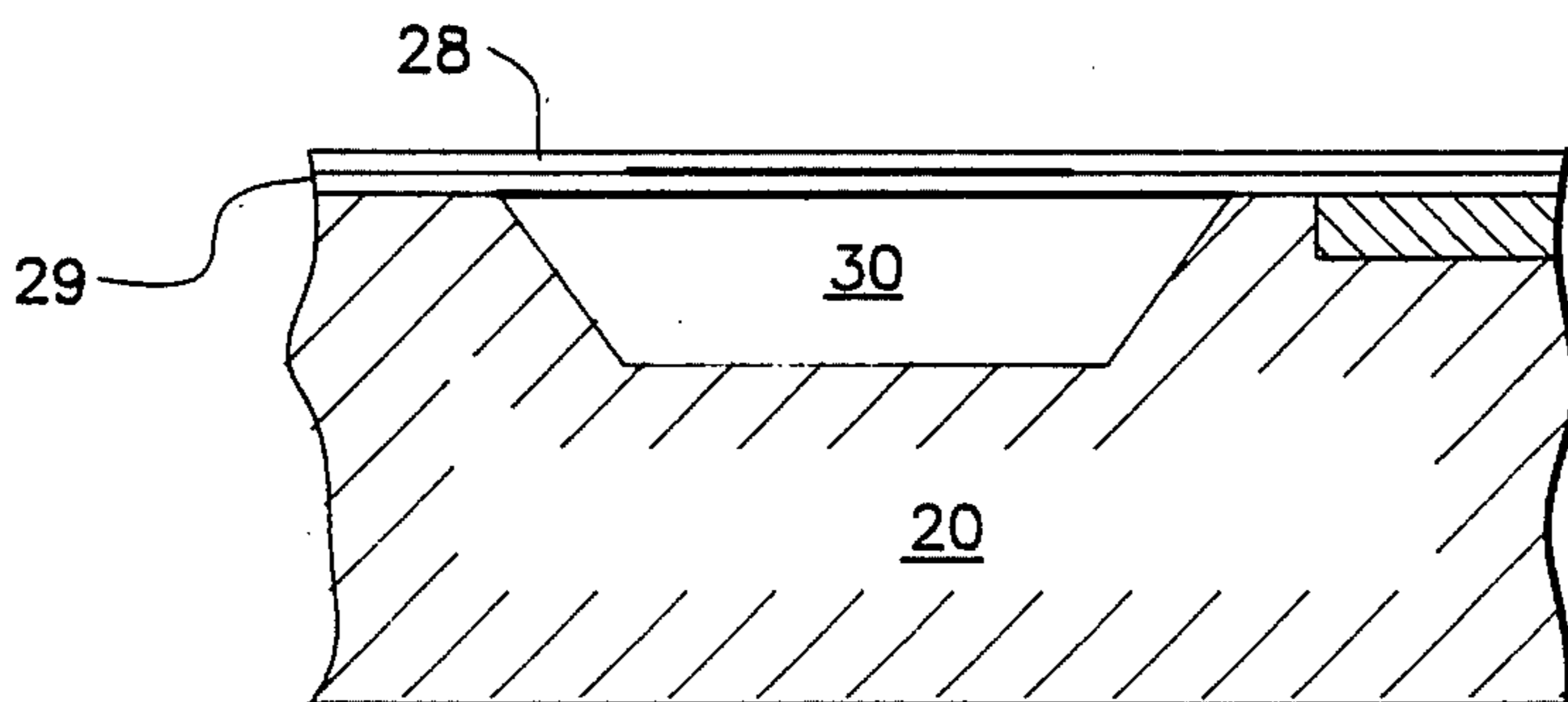
Fig. 3 (PRIOR ART)
