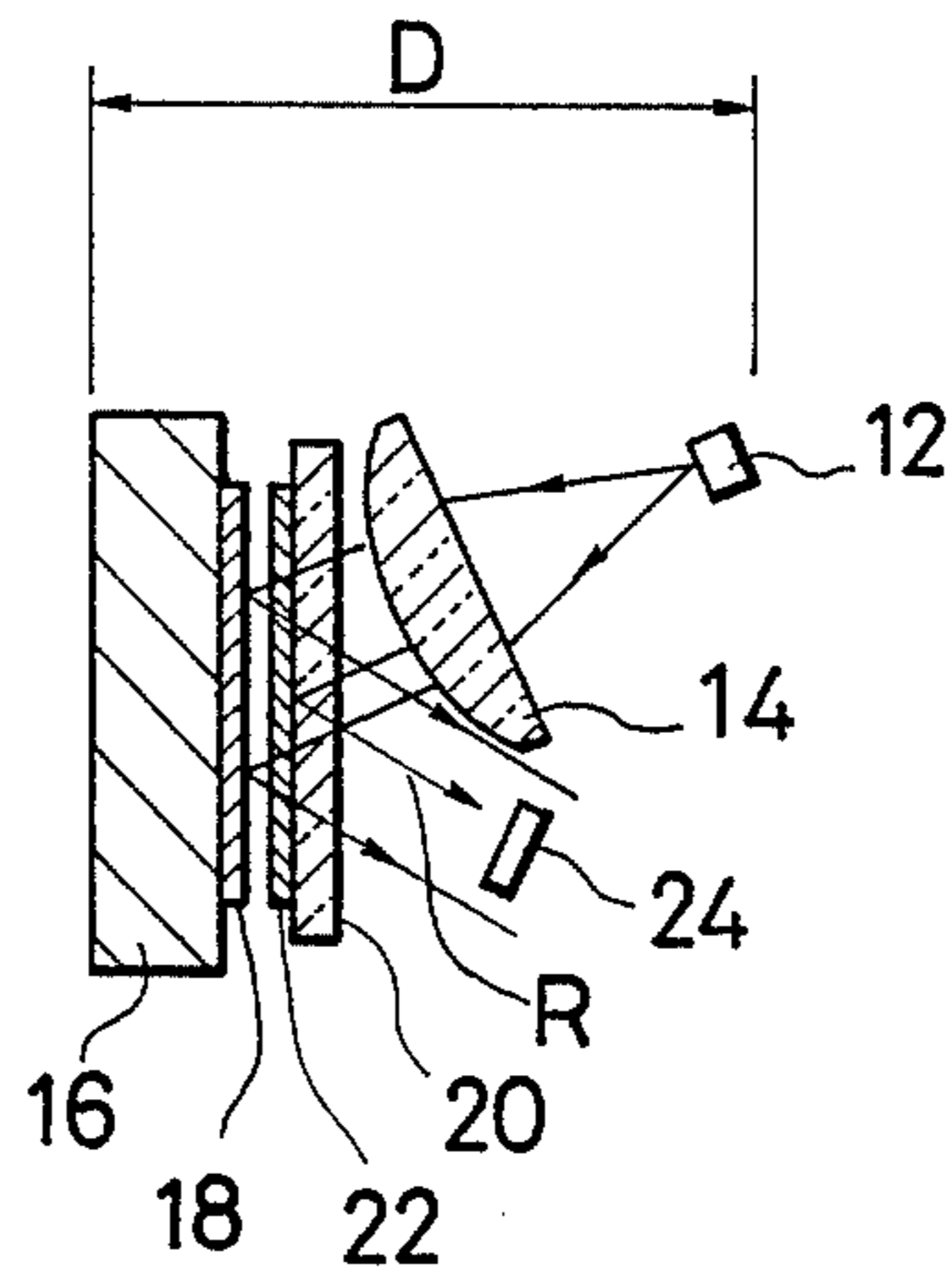
FIG. 15 PRIOR ART
