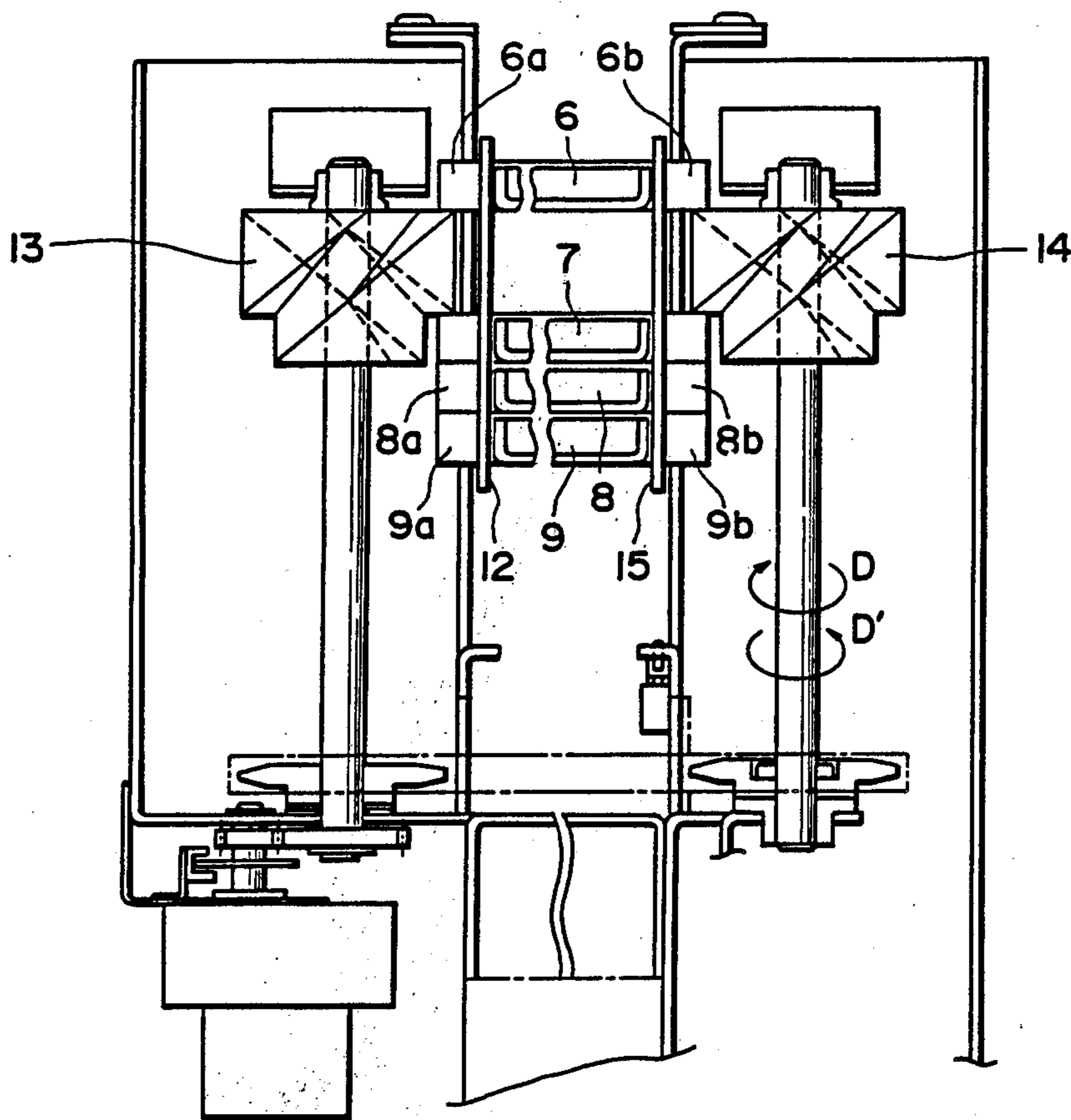
FIG. 2 PRIOR ART
