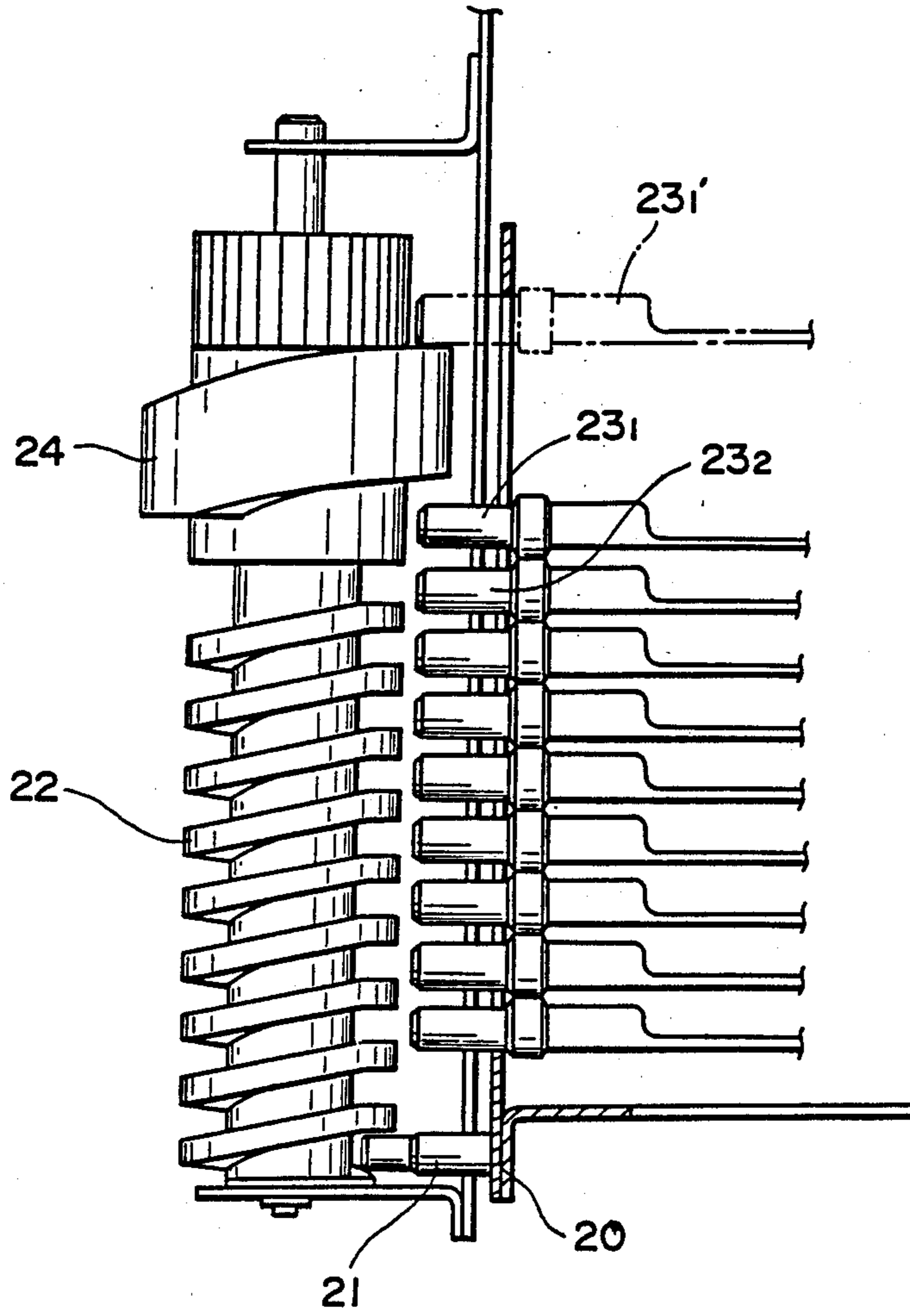
FIG. 3 PRIOR ART
