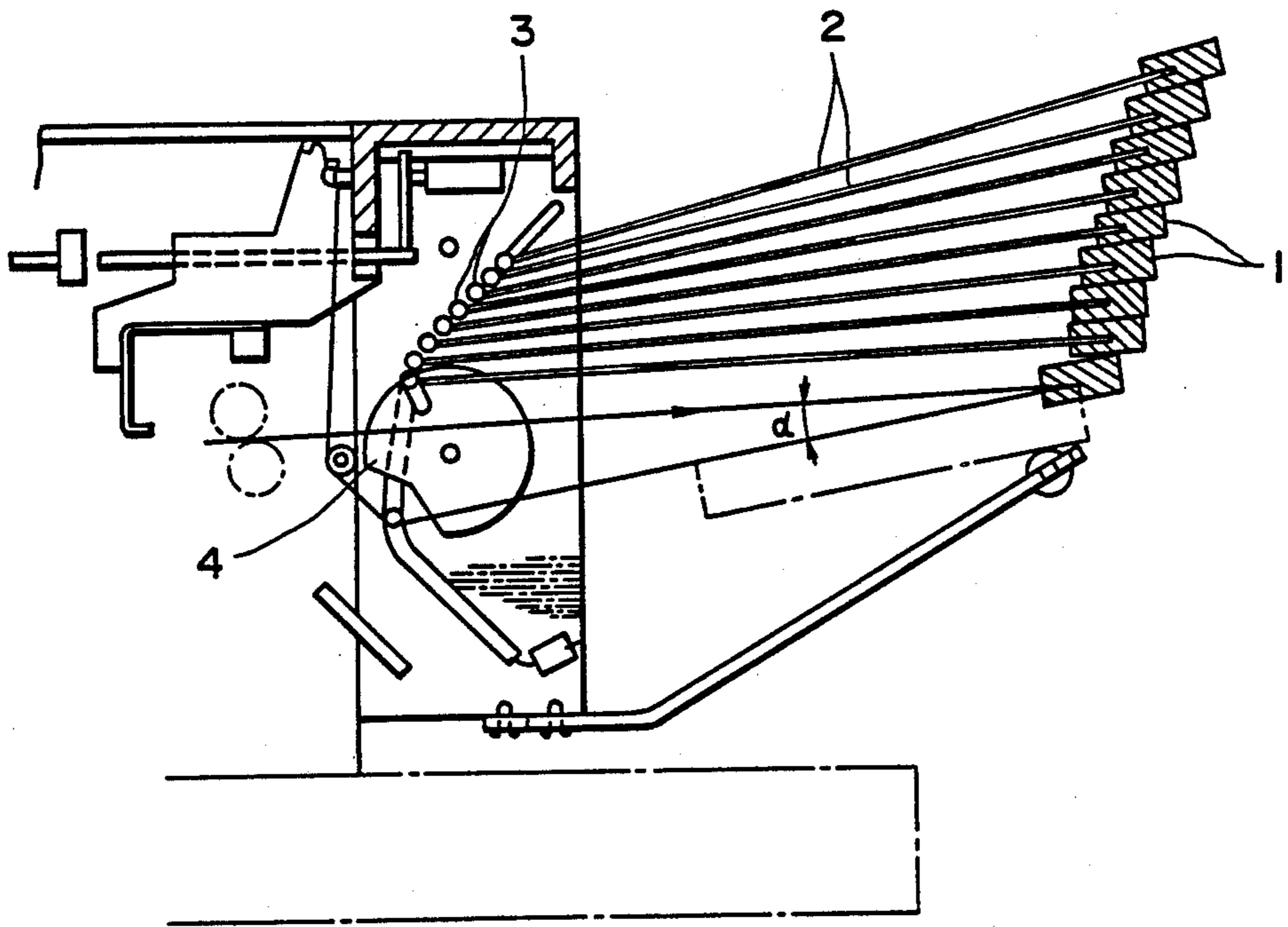
FIG. 1 PRIOR ART
