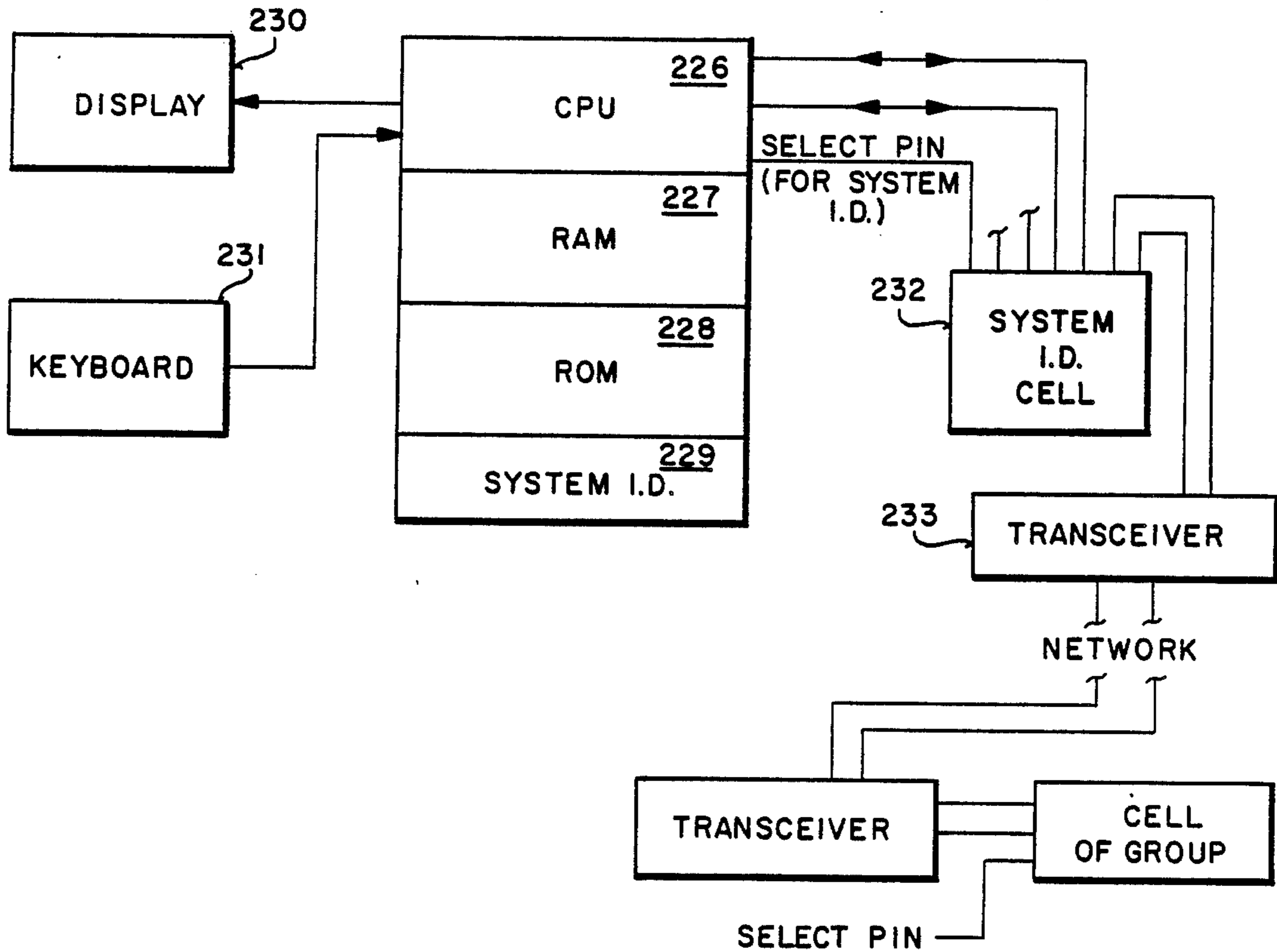
FIG 28 GROUPING DEVICE
