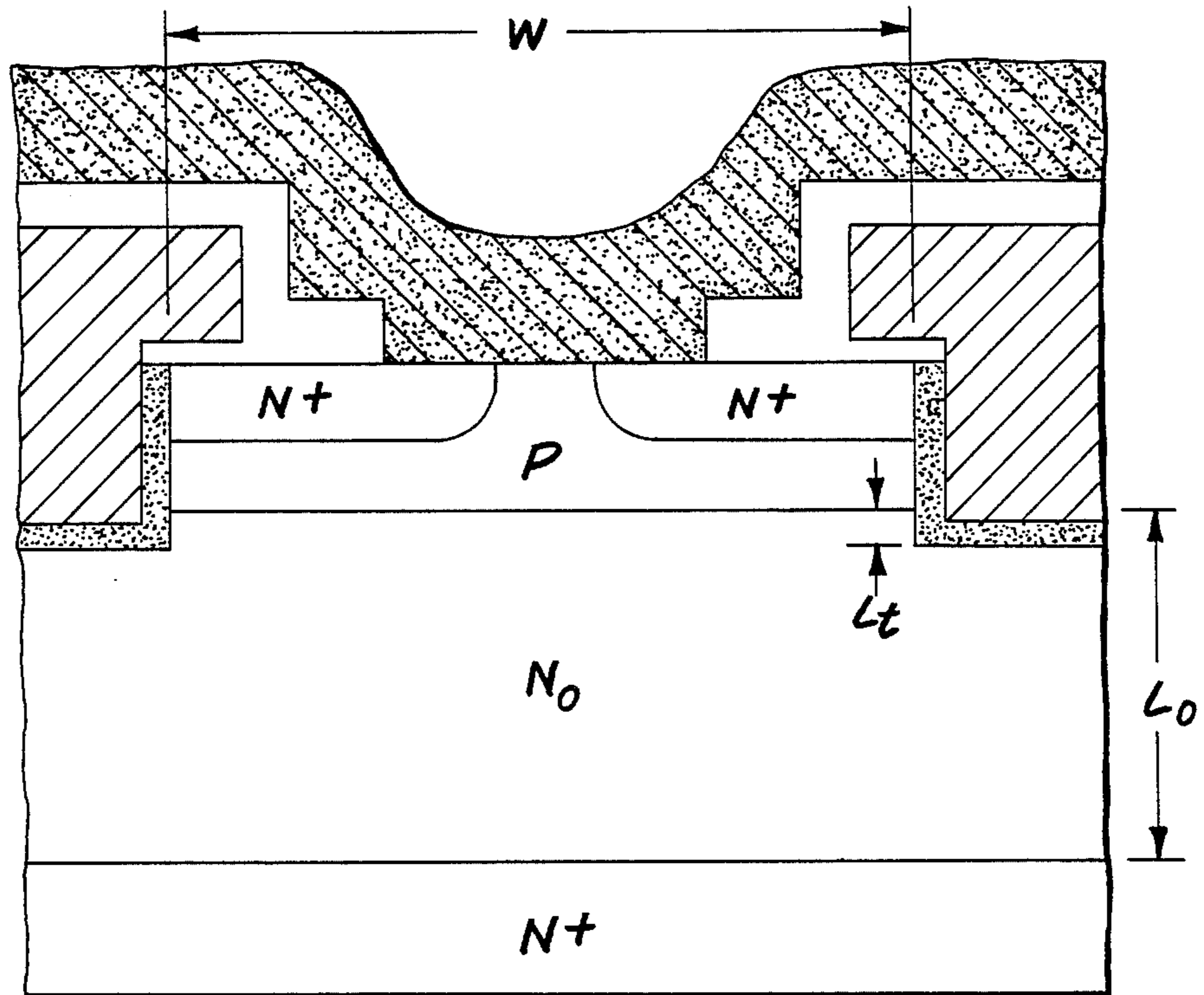
FIG. 1 CONVENTIONAL DEVICE
