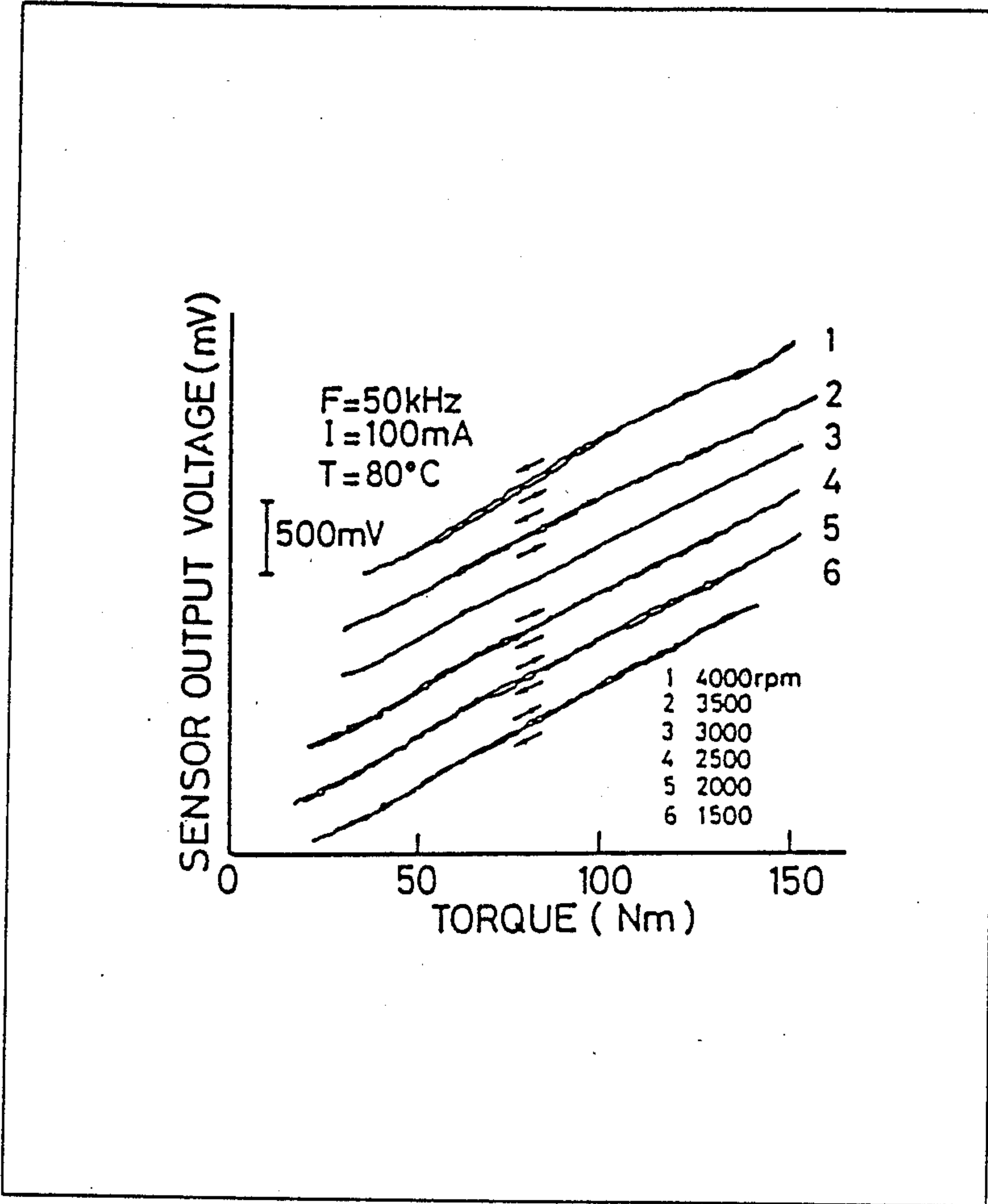
FIGURE 4: PRIOR ART
