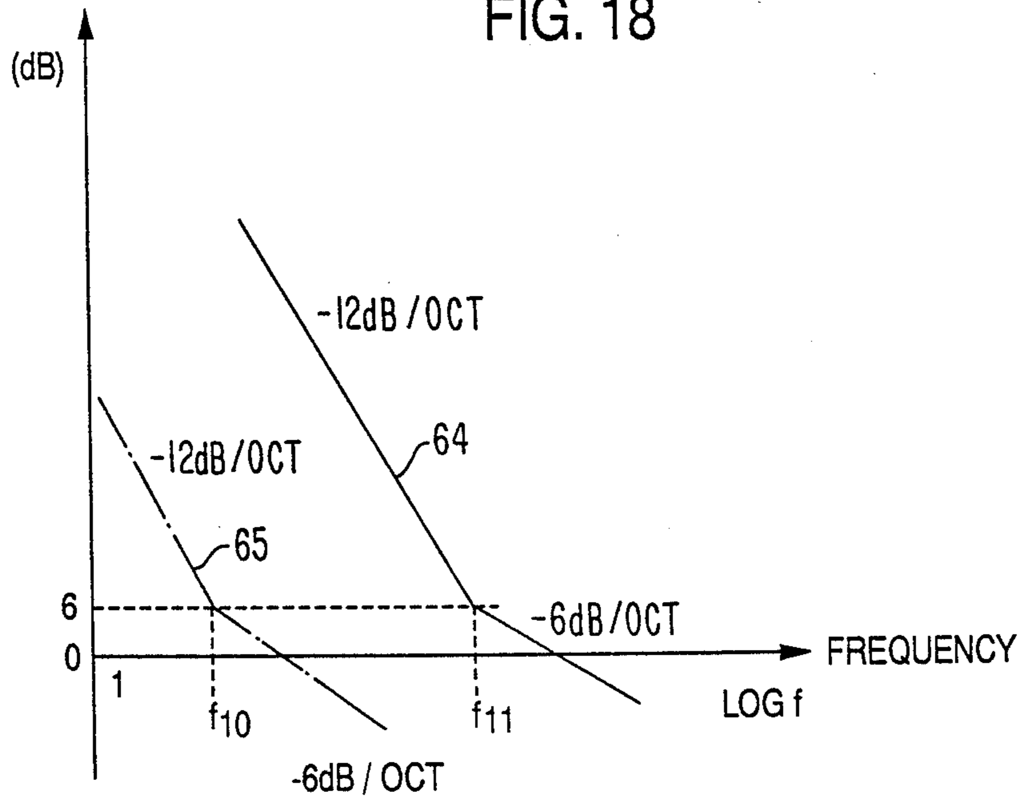
OPEN-LOOP TRANSMISSION CHARACTERISTICS
