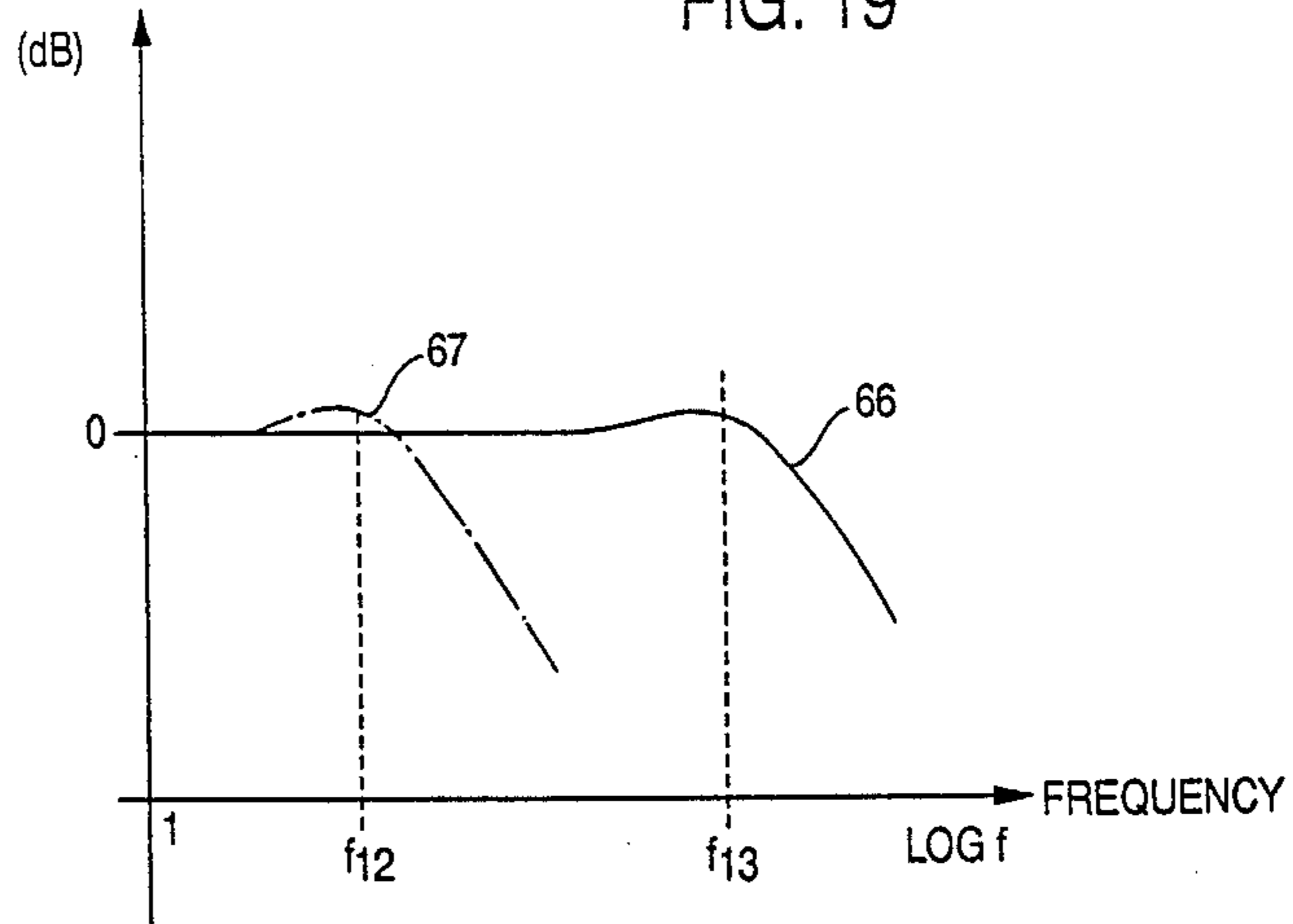
CLOSED-LOOP TRANSMISSION CHARACTERISTICS
