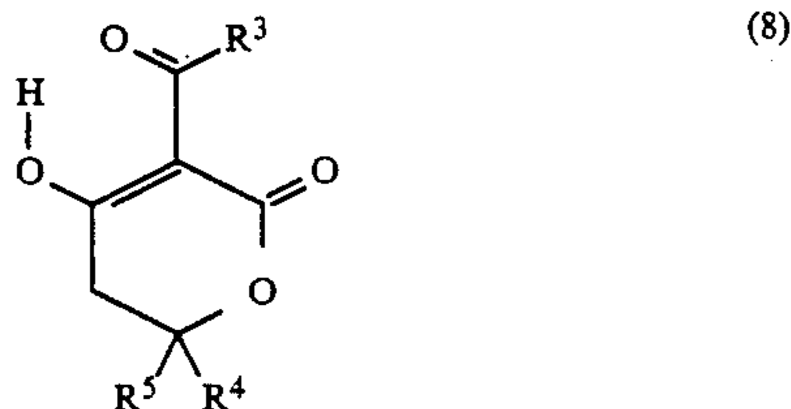
3-Acyl-4-hydroxy-6,6-disubstituted-5,6-dihydro-2H-pyran-2-ones
