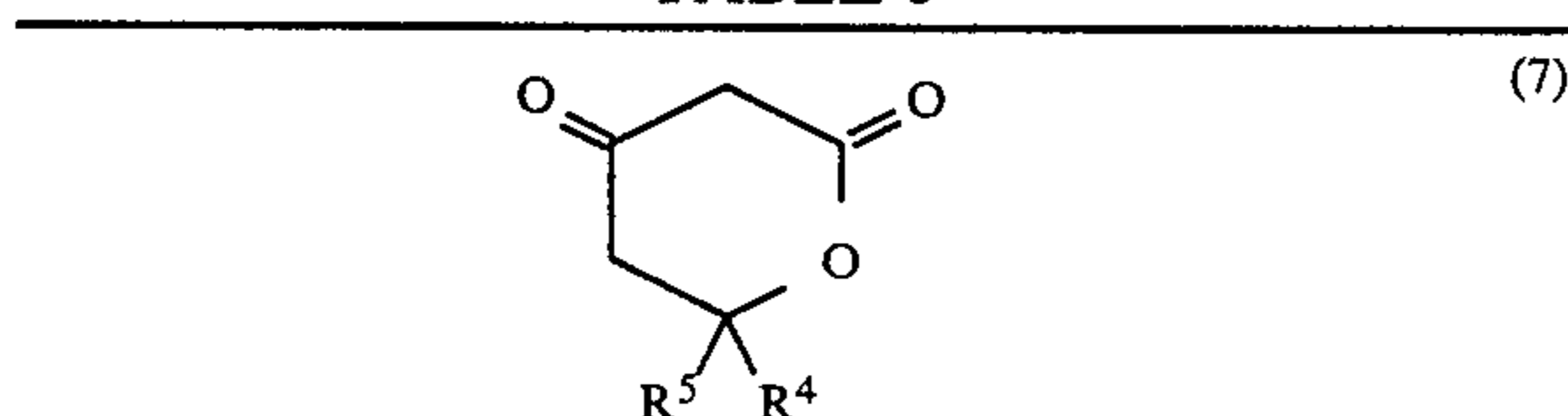
6,6-Disubstituted-5,6-dihydro-2H-pyran-2,4-diones
