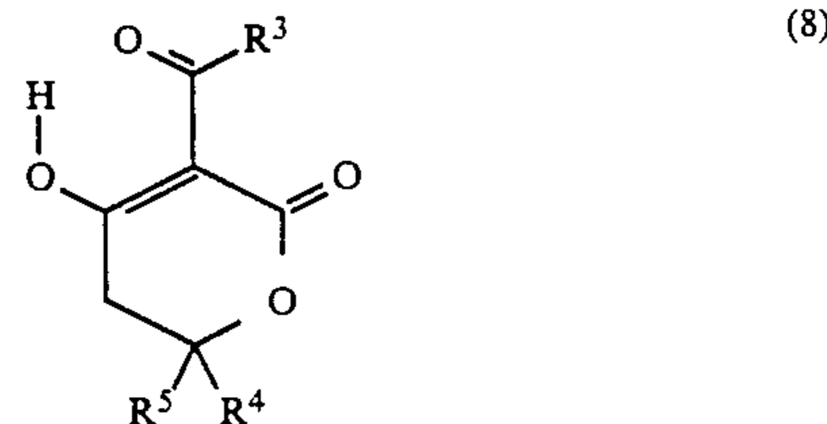
3-Acyl-4-hydroxy-6,6-disubstituted-5,6-dihydro-2H-pyran-2-ones
