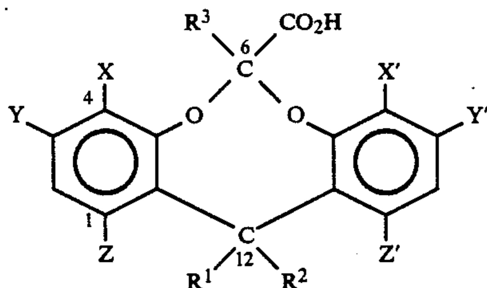
Formula I
