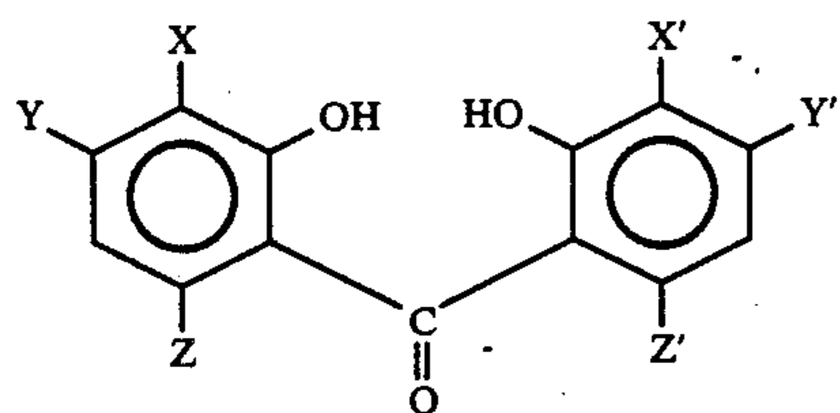
Formula IX
