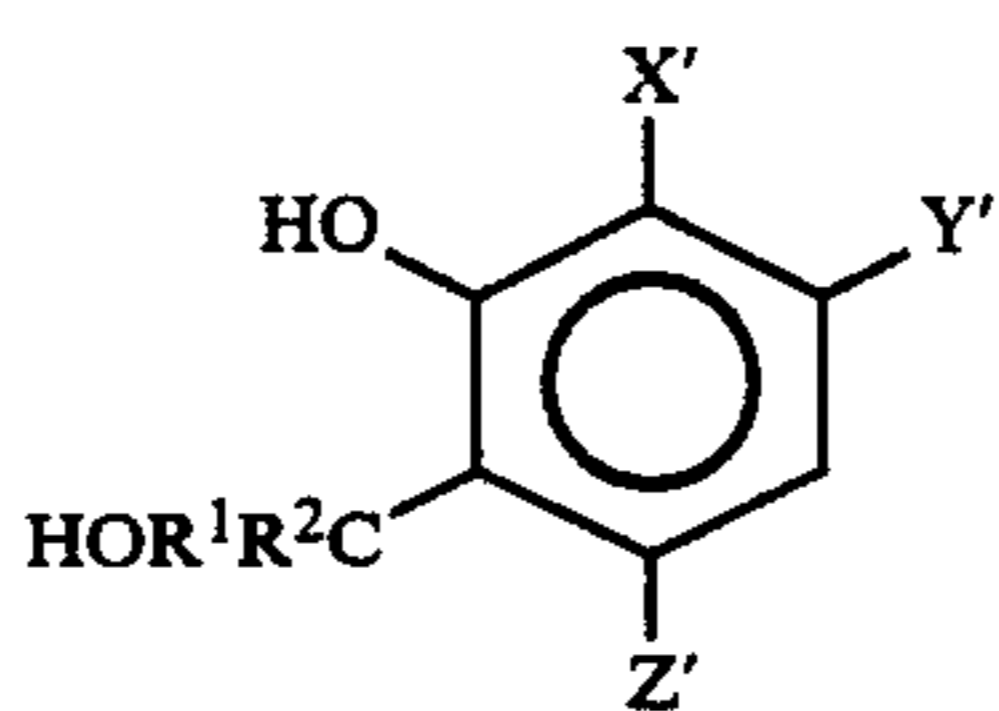
Formula VIII
