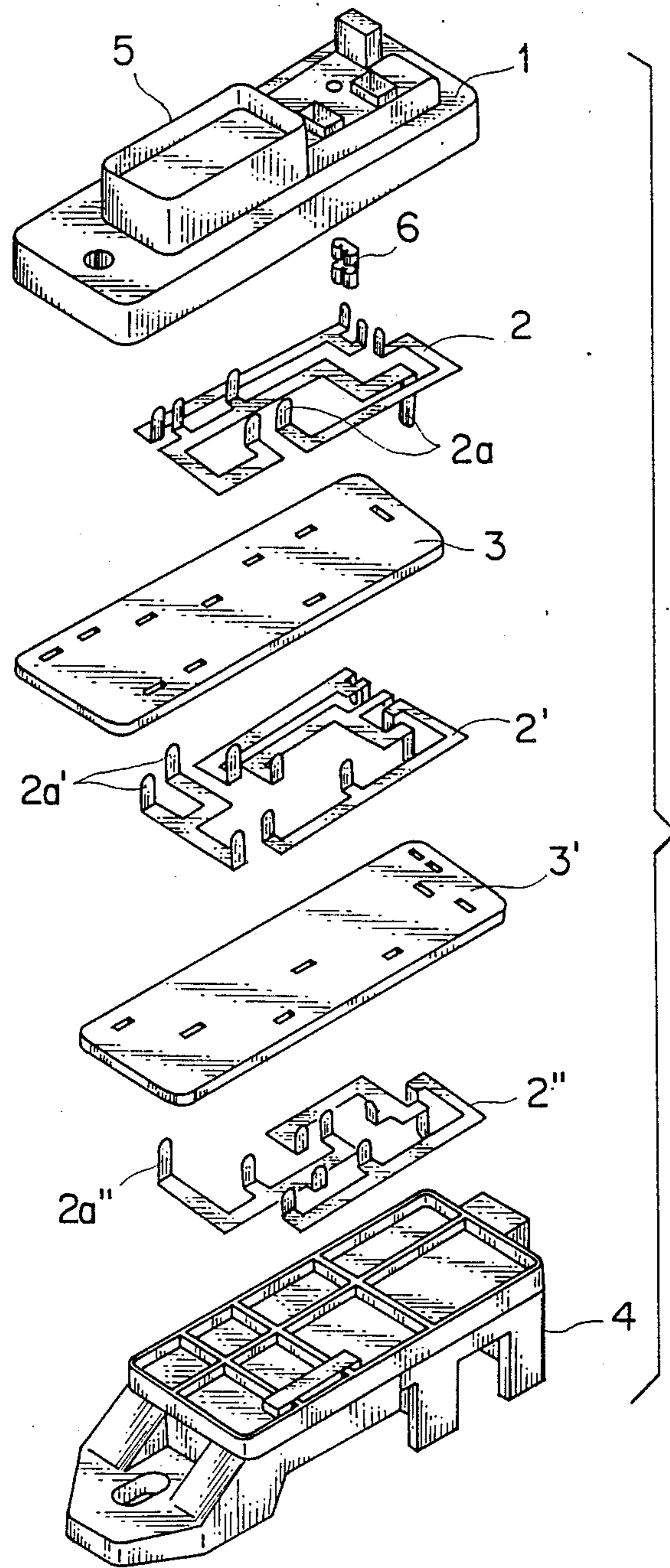
FIG. 6 PRIOR ART
