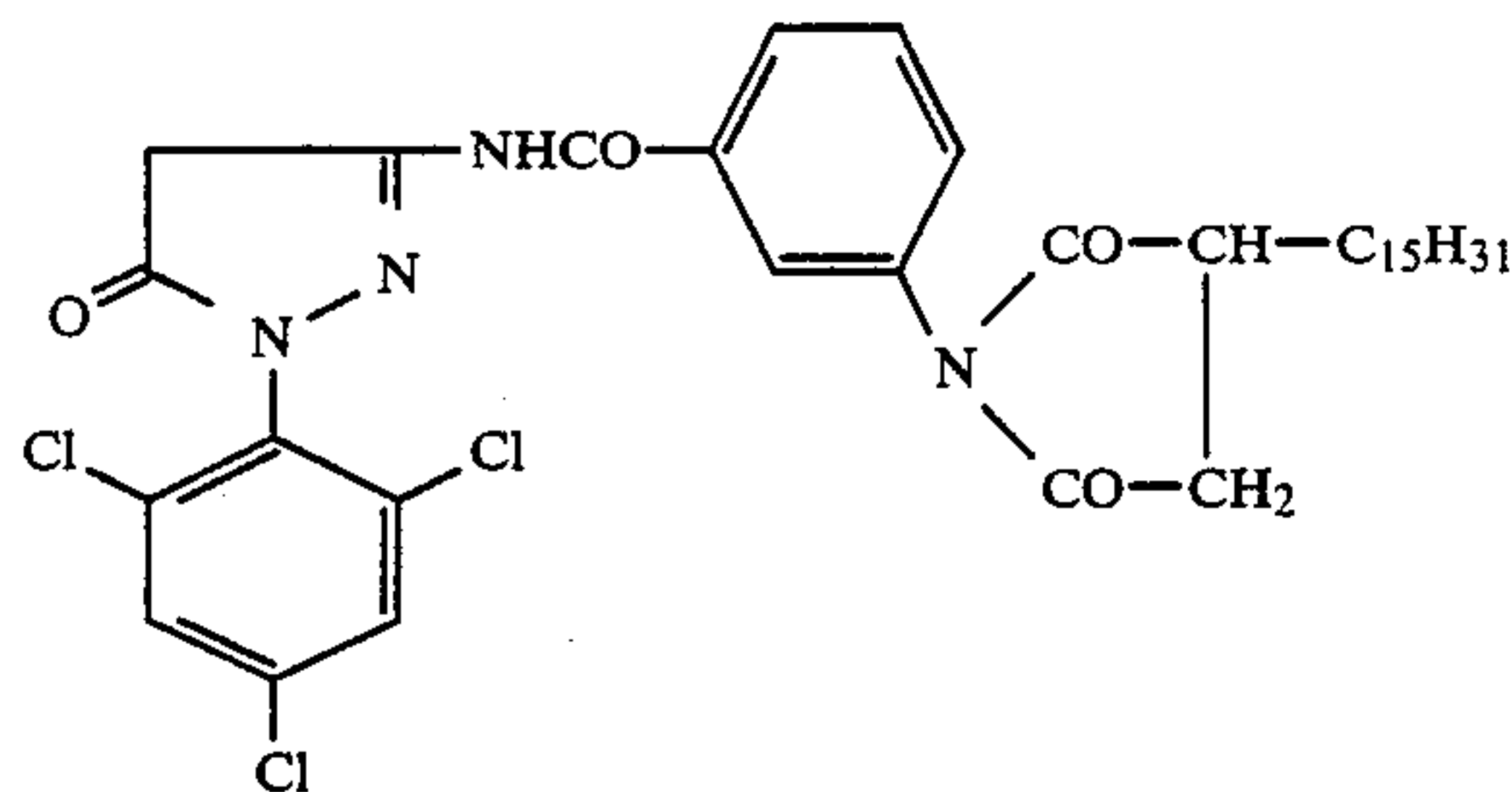
Comparative coupler (26-2)
