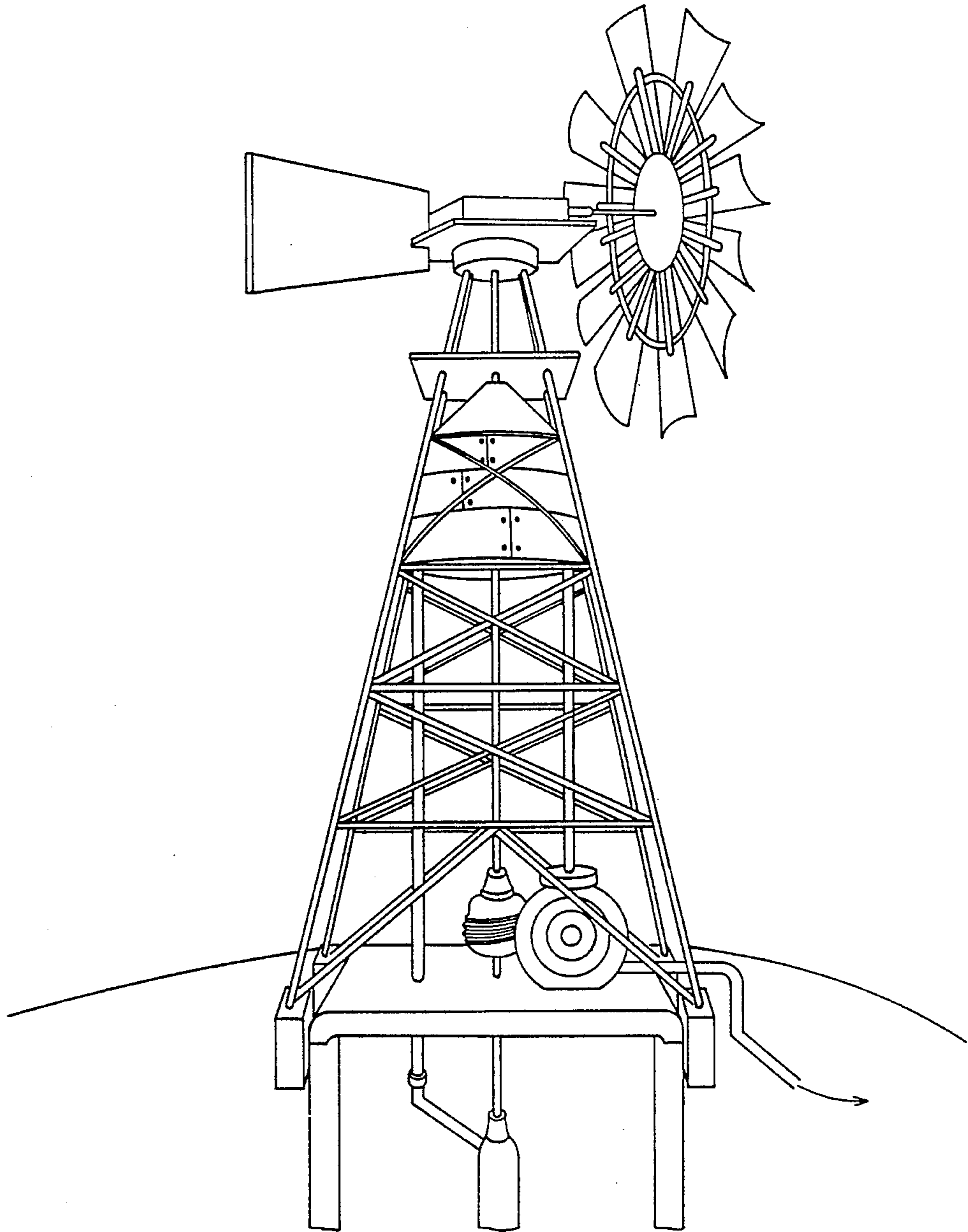
FIG. 1 PRIOR ART
