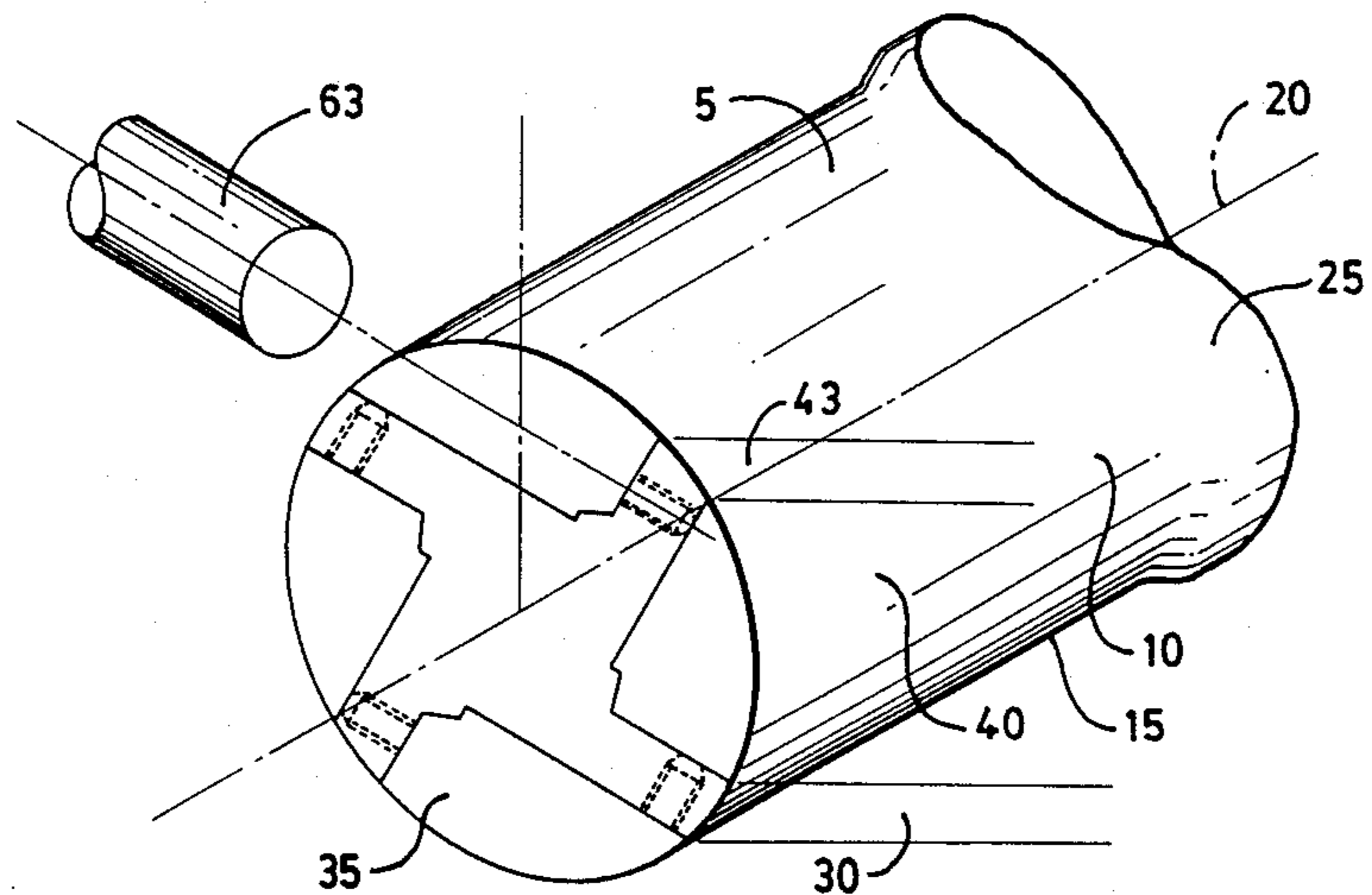
FIG. 1 PRIOR ART
