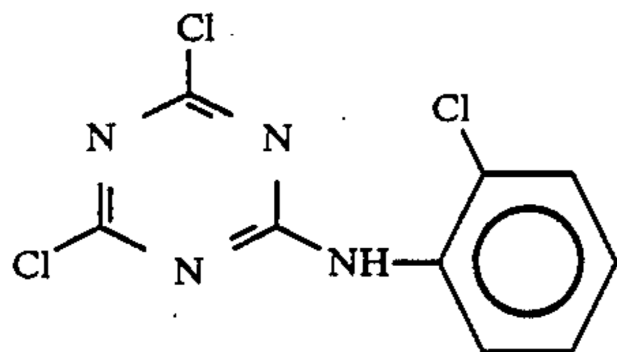
(ANILAZINE)
