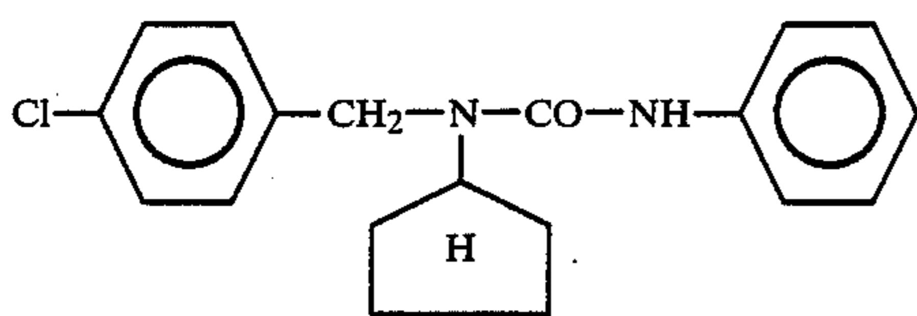
(PENCYCURON)
