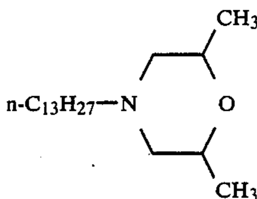
(TRIDEMORPH)
