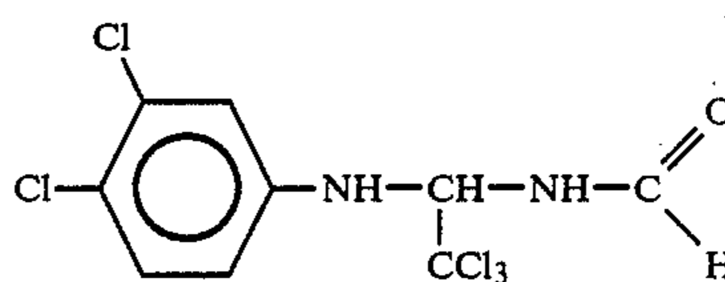
(CHLORANIFORMETHANE)
