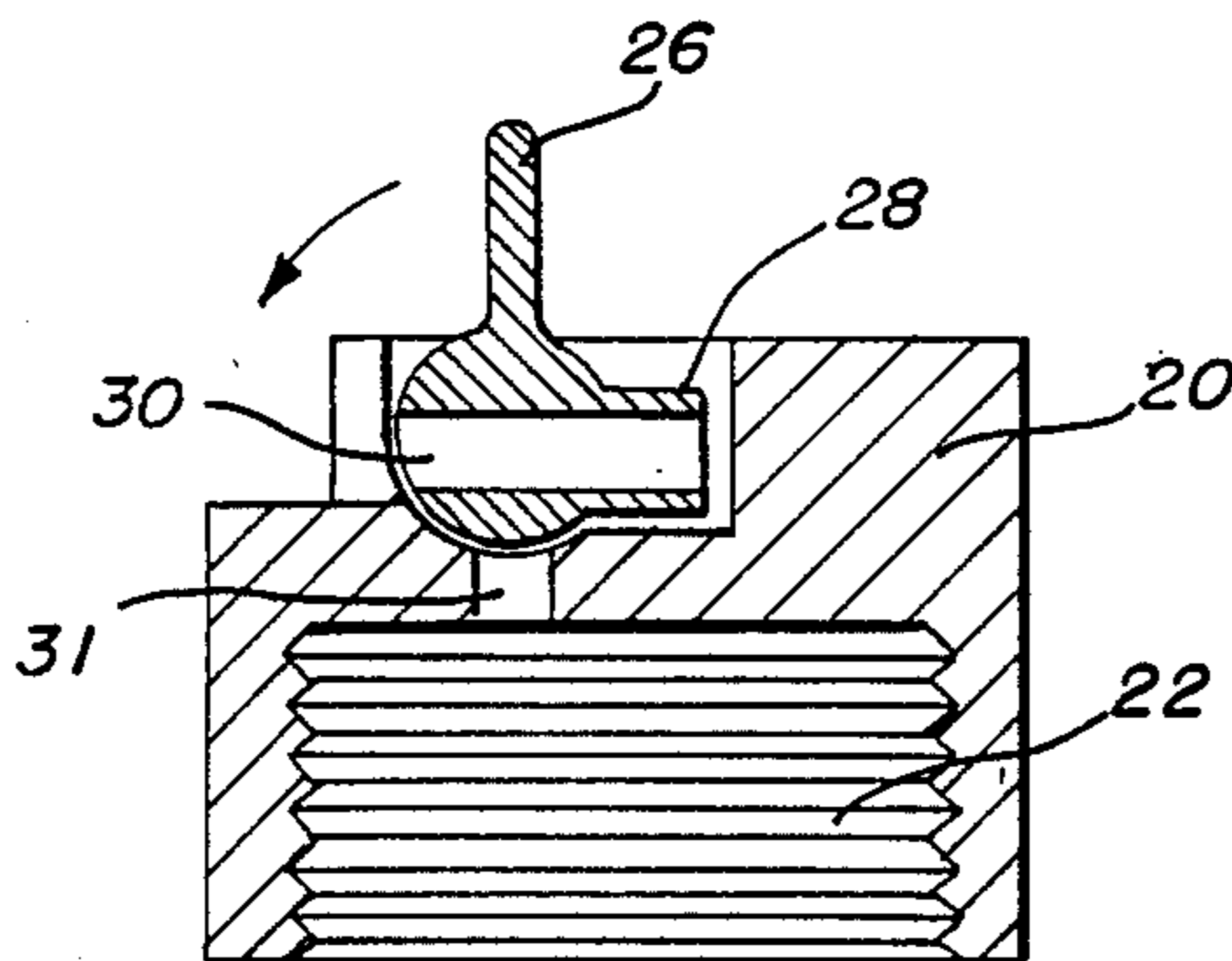
FIG. 5A (CLOSED)
