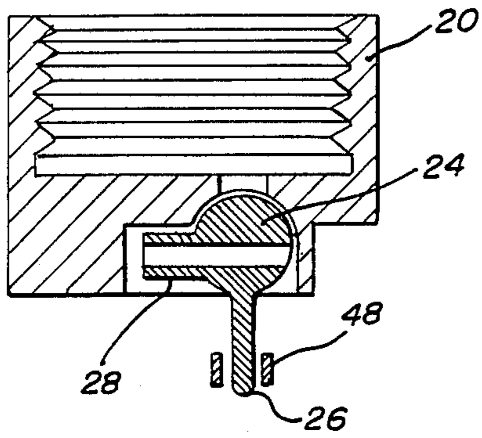
FIG. 8A (CLOSED)
