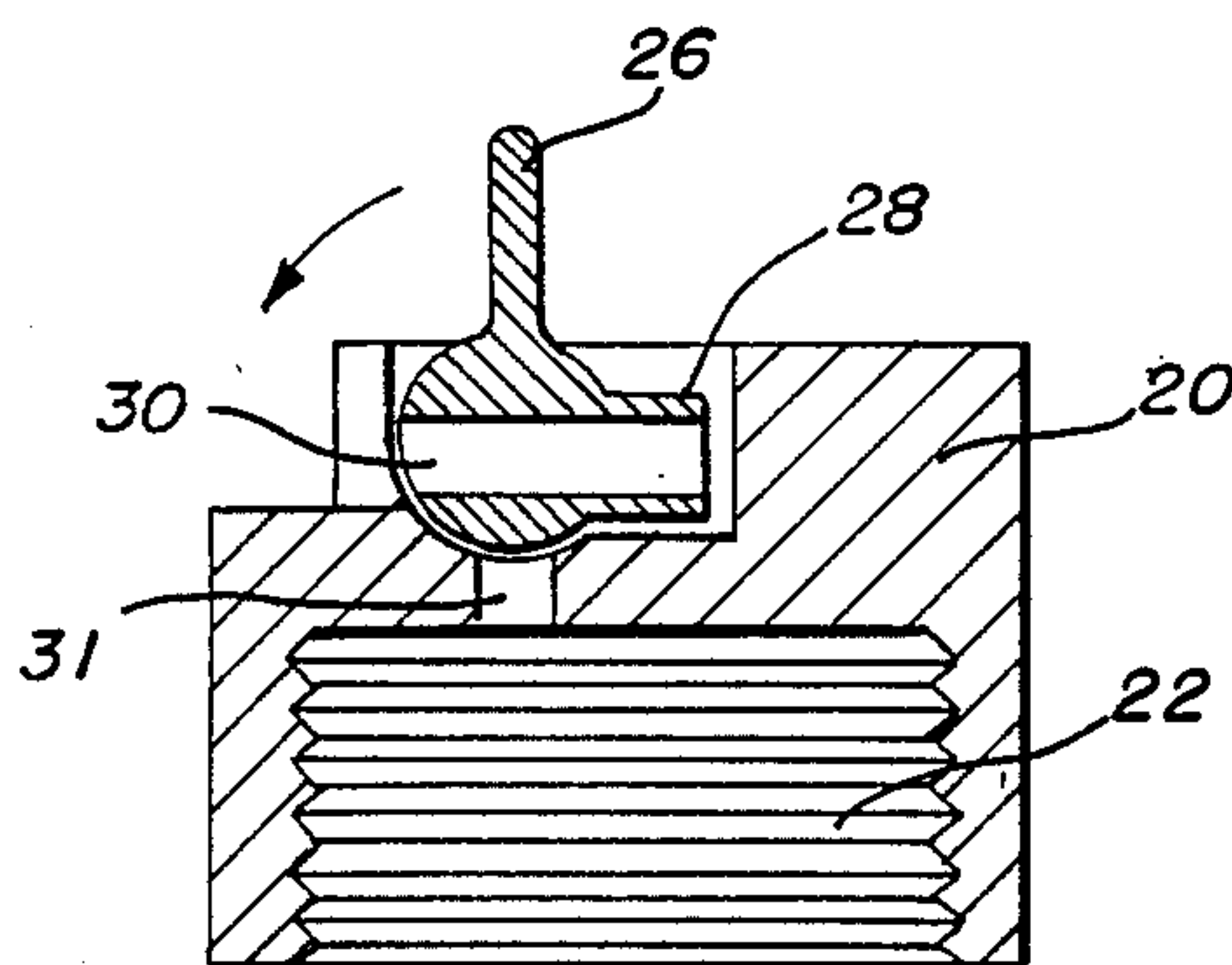
FIG. 5A (CLOSED)
