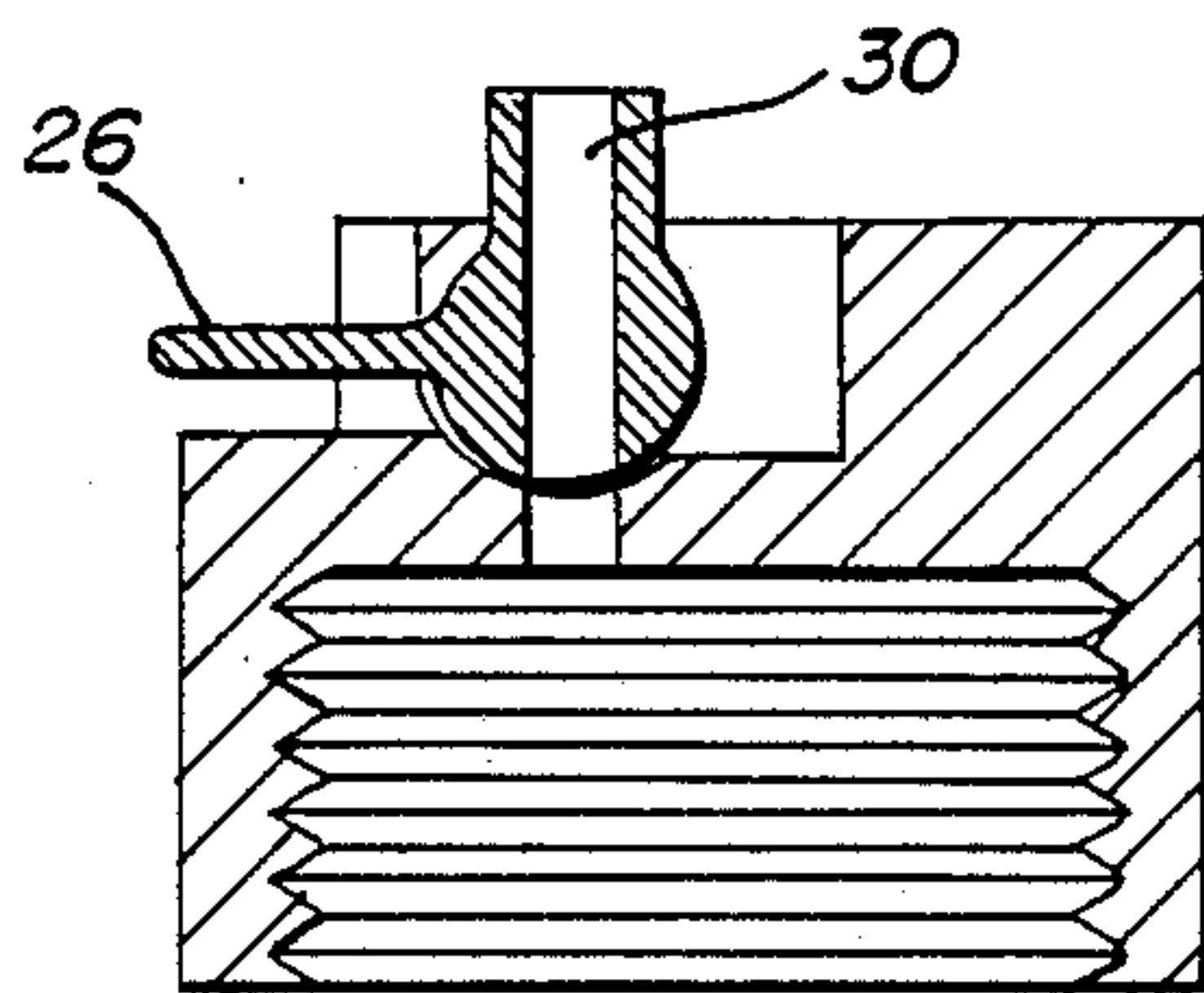
FIG. 5B (OPEN)
