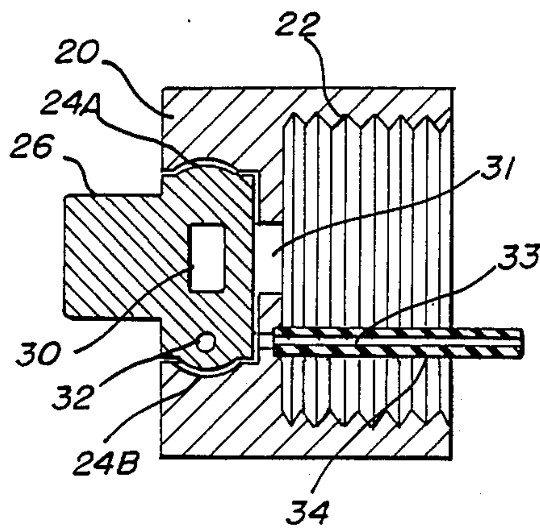
FIG. 4 (CLOSED)
