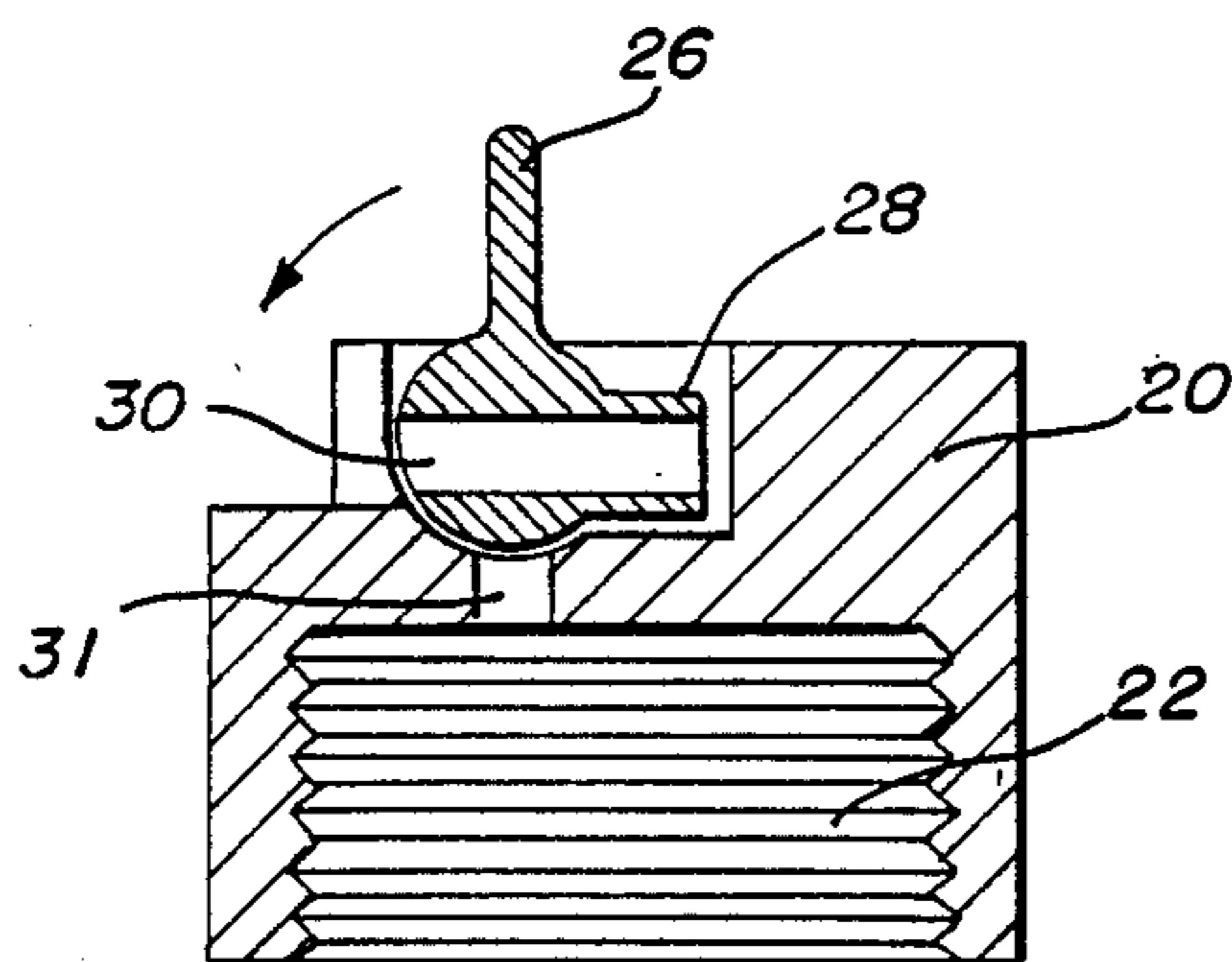
FIG. 5A (CLOSED)
