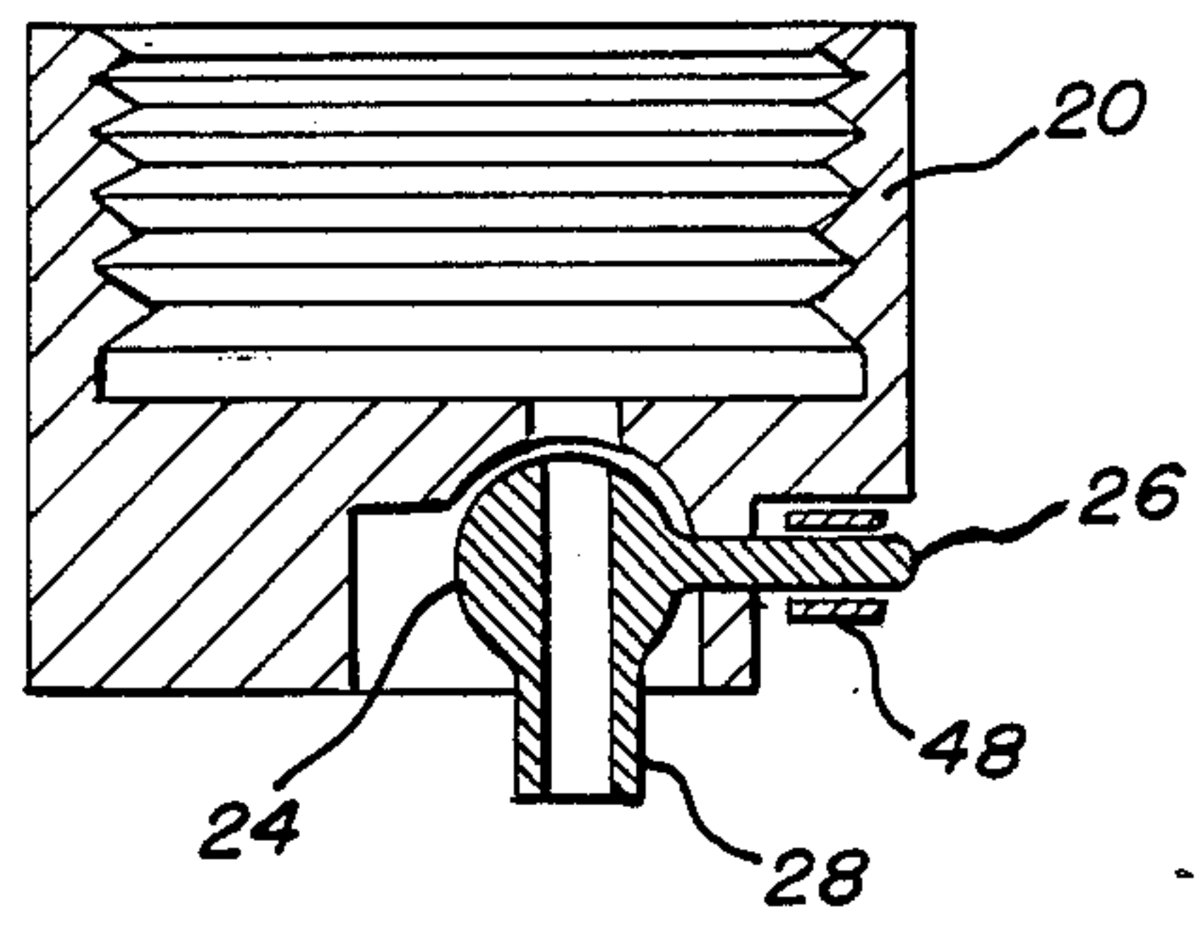
FIG. 8B (OPEN)
