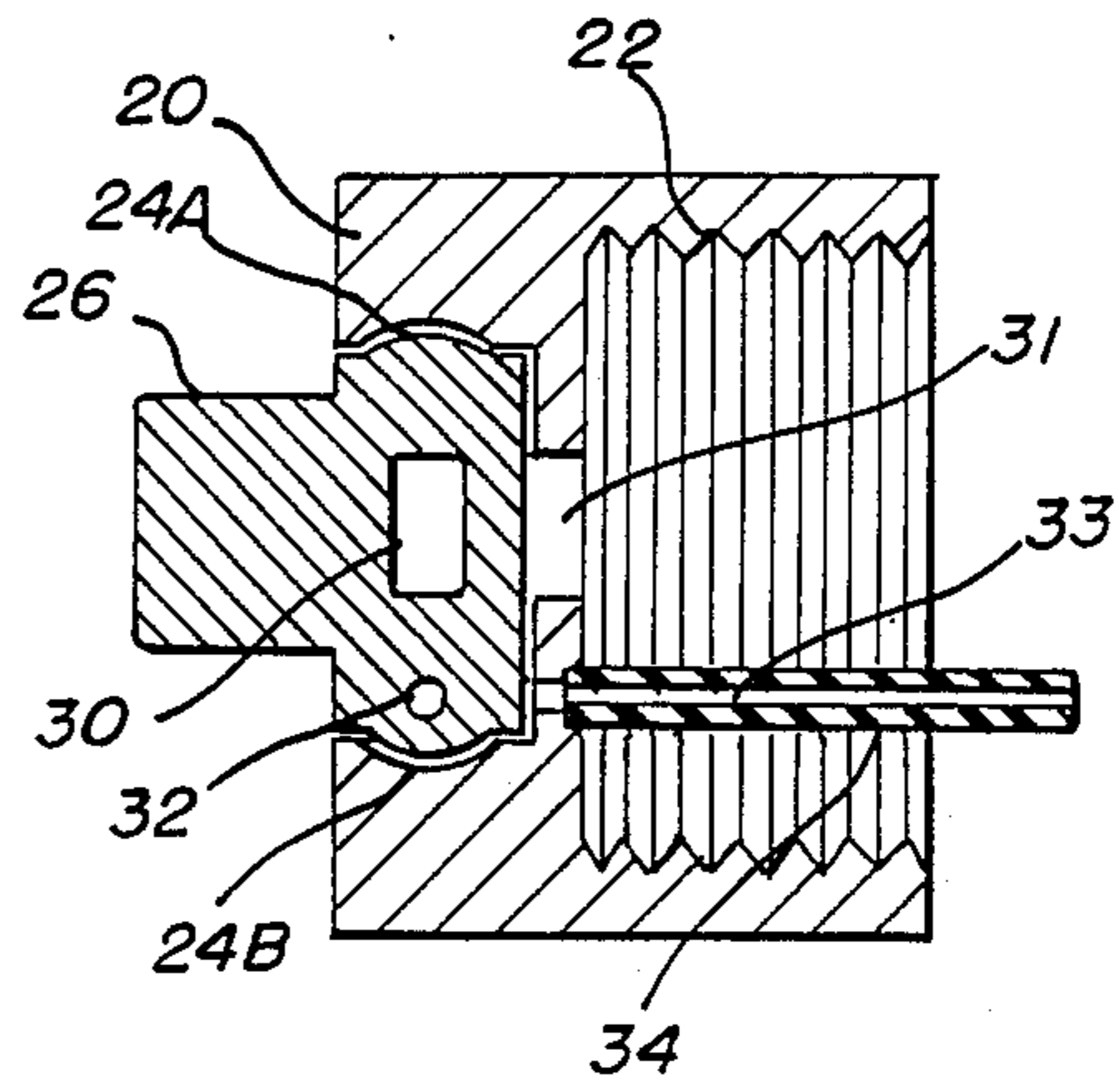
FIG. 4 (CLOSED)
