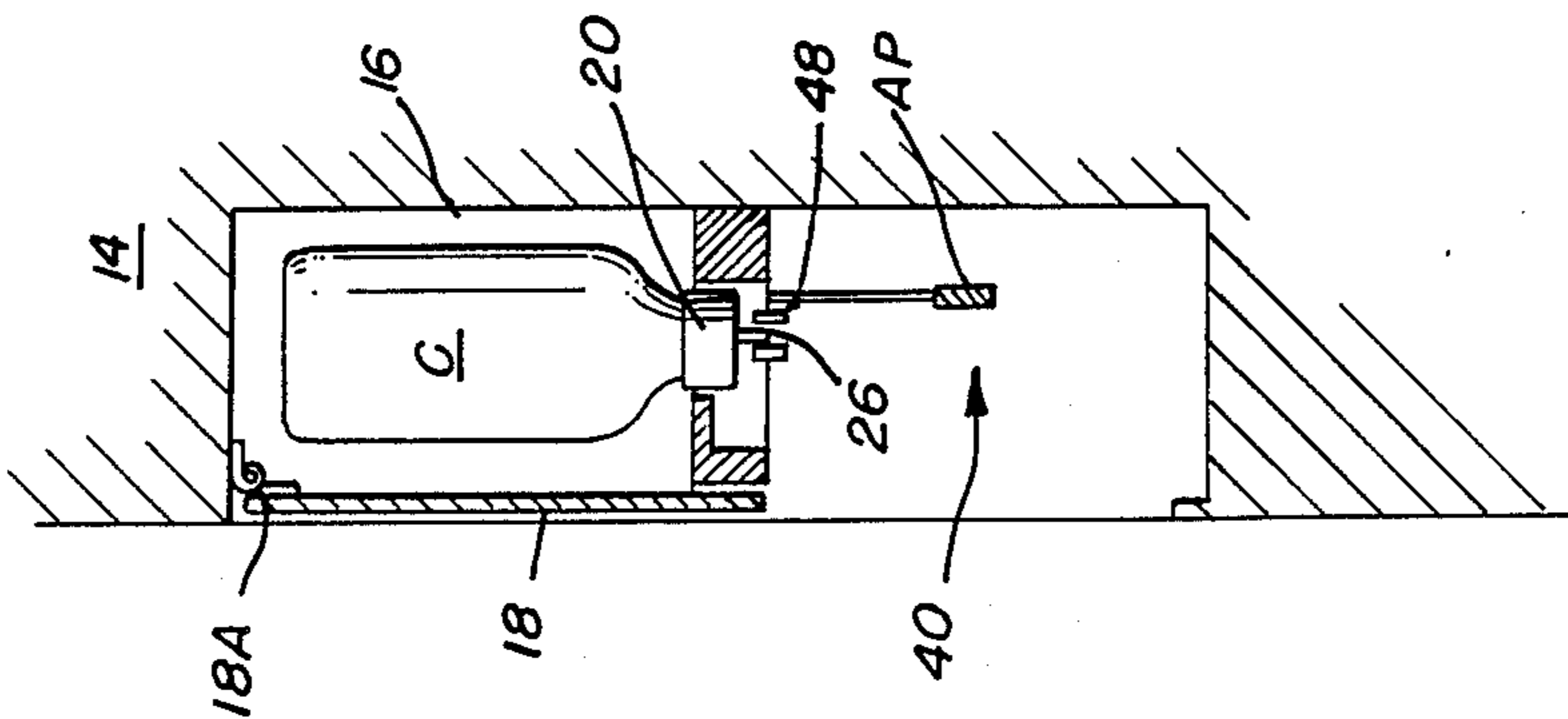
FIG. 2A (CLOSED POSITION)
