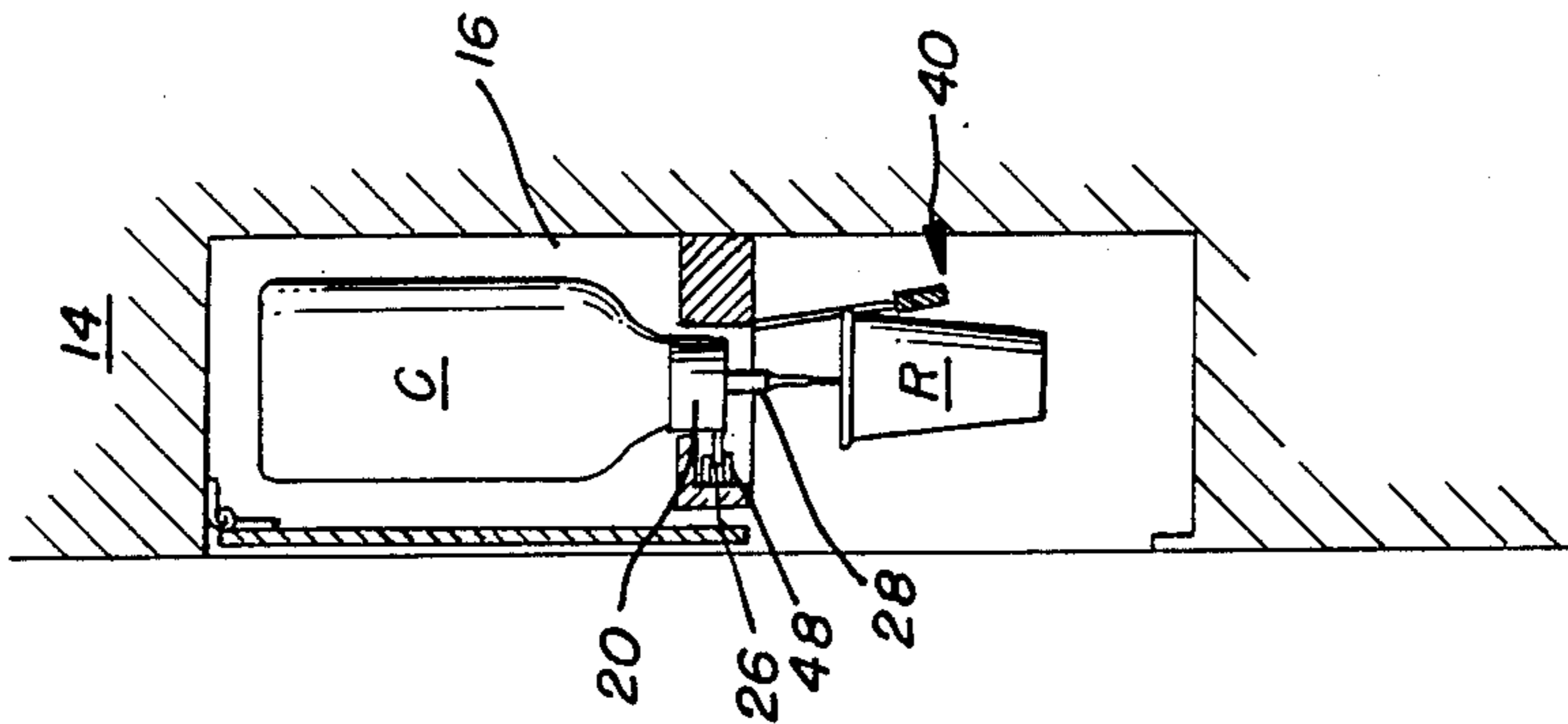
FIG. 2B (OPEN POSITION)
