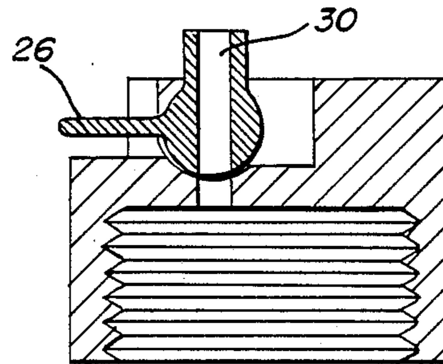
FIG. 5B (OPEN)
