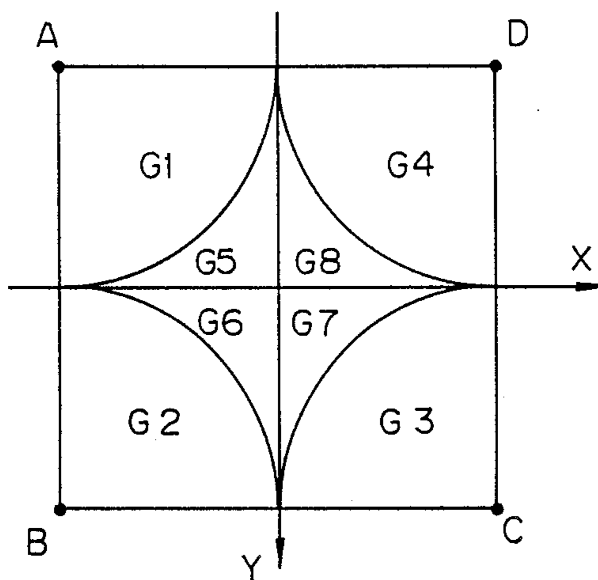
Fig. 3 CURVE DEFINITION
