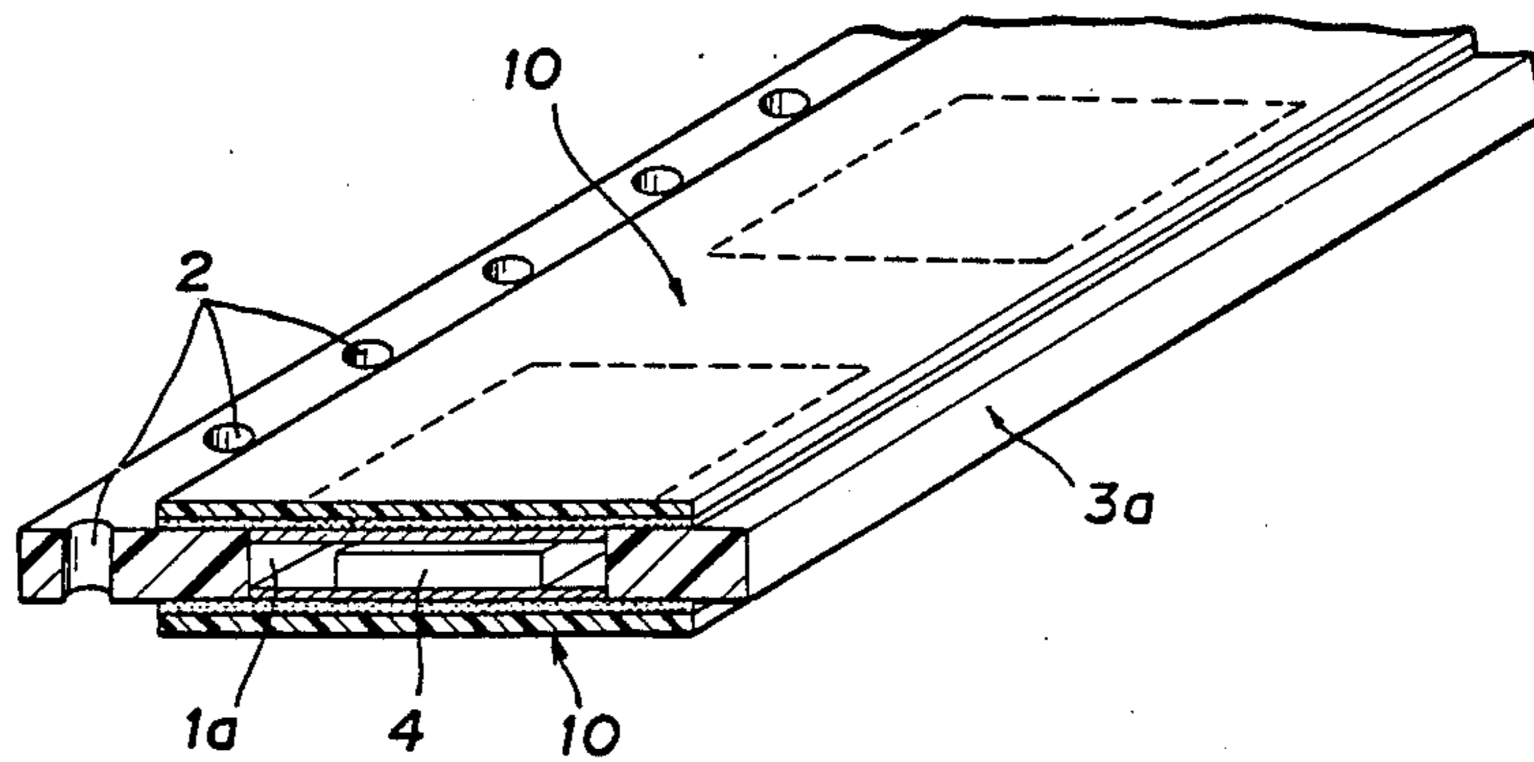
FIG. 4 PRIOR ART
