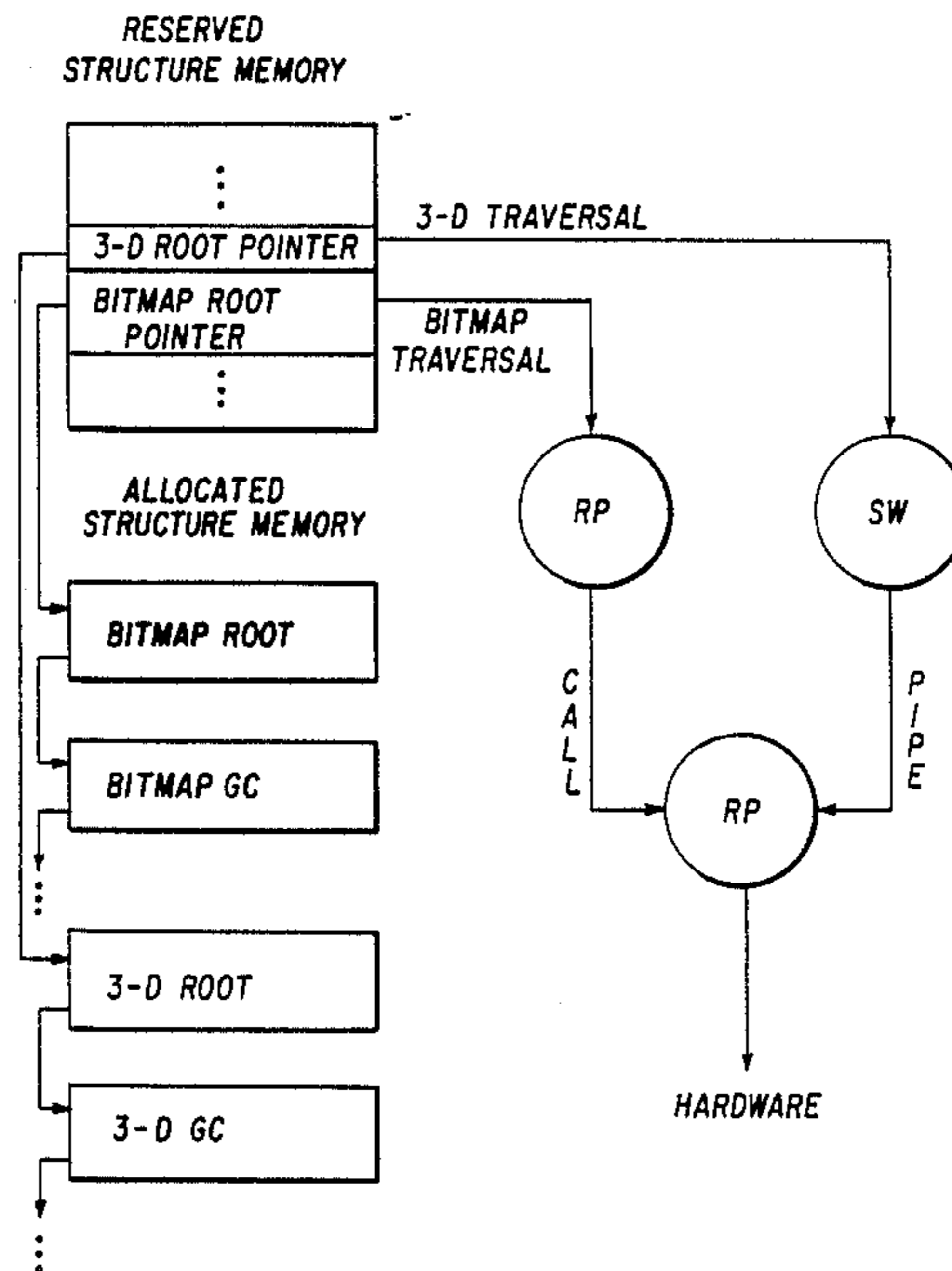
GRAPHICS CONTEXT AND TRAVERSAL MODEL
