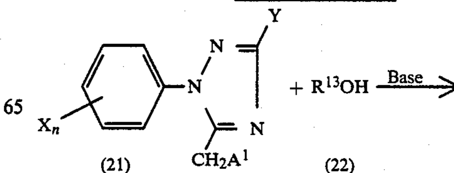
Reaction scheme 6
