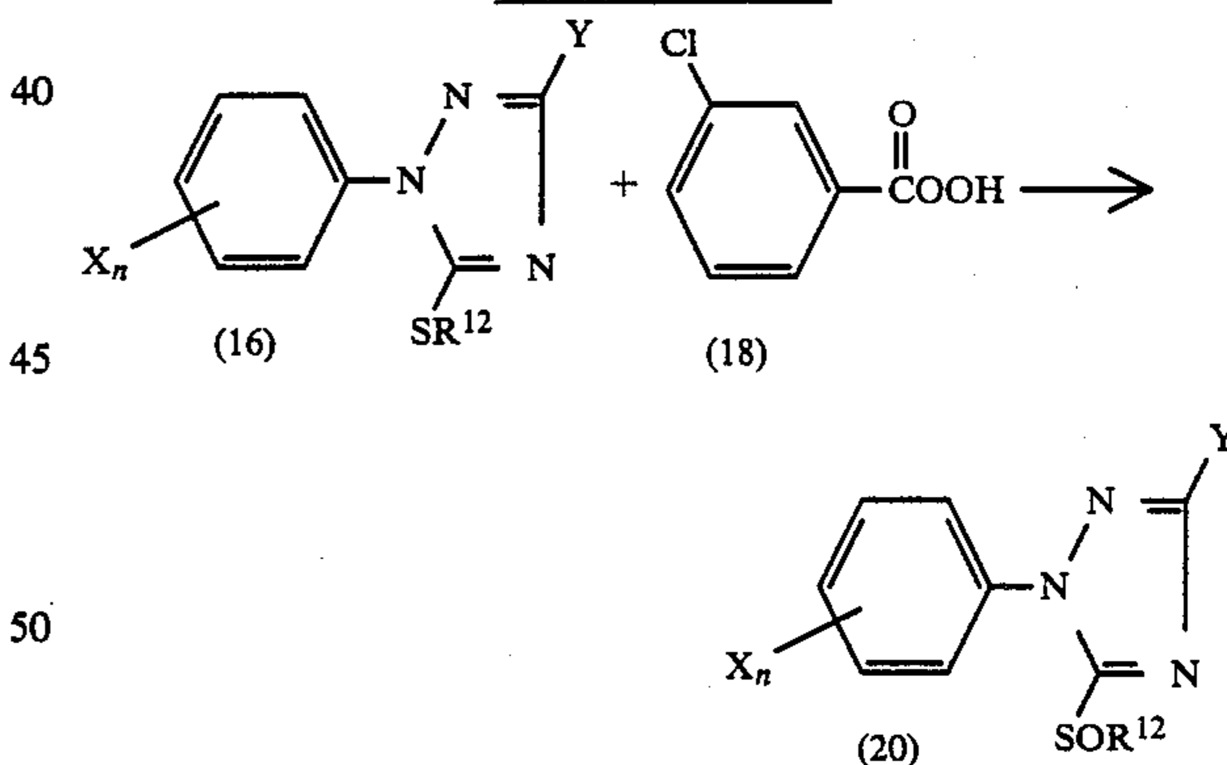
Reaction scheme 5
