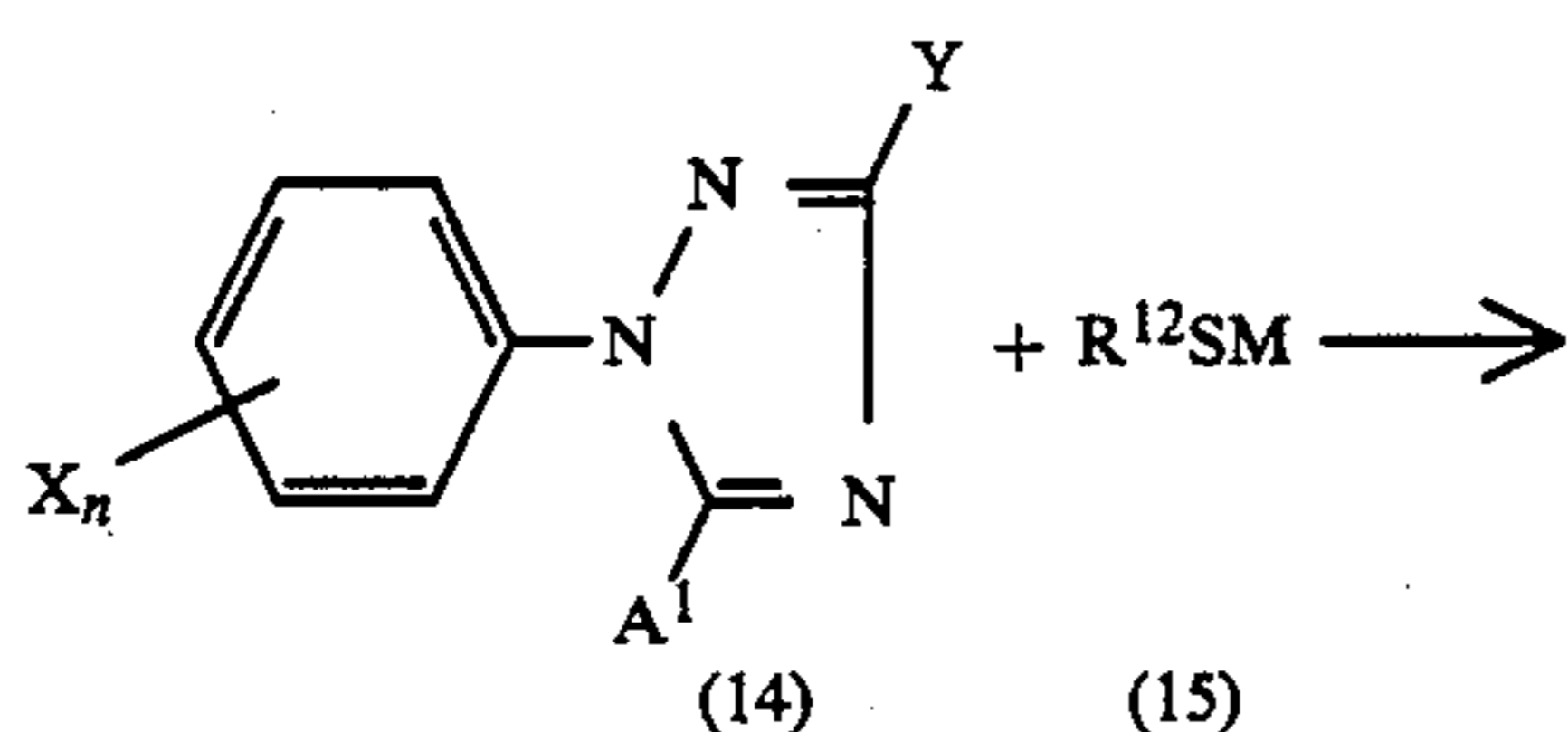
Reaction scheme 4
