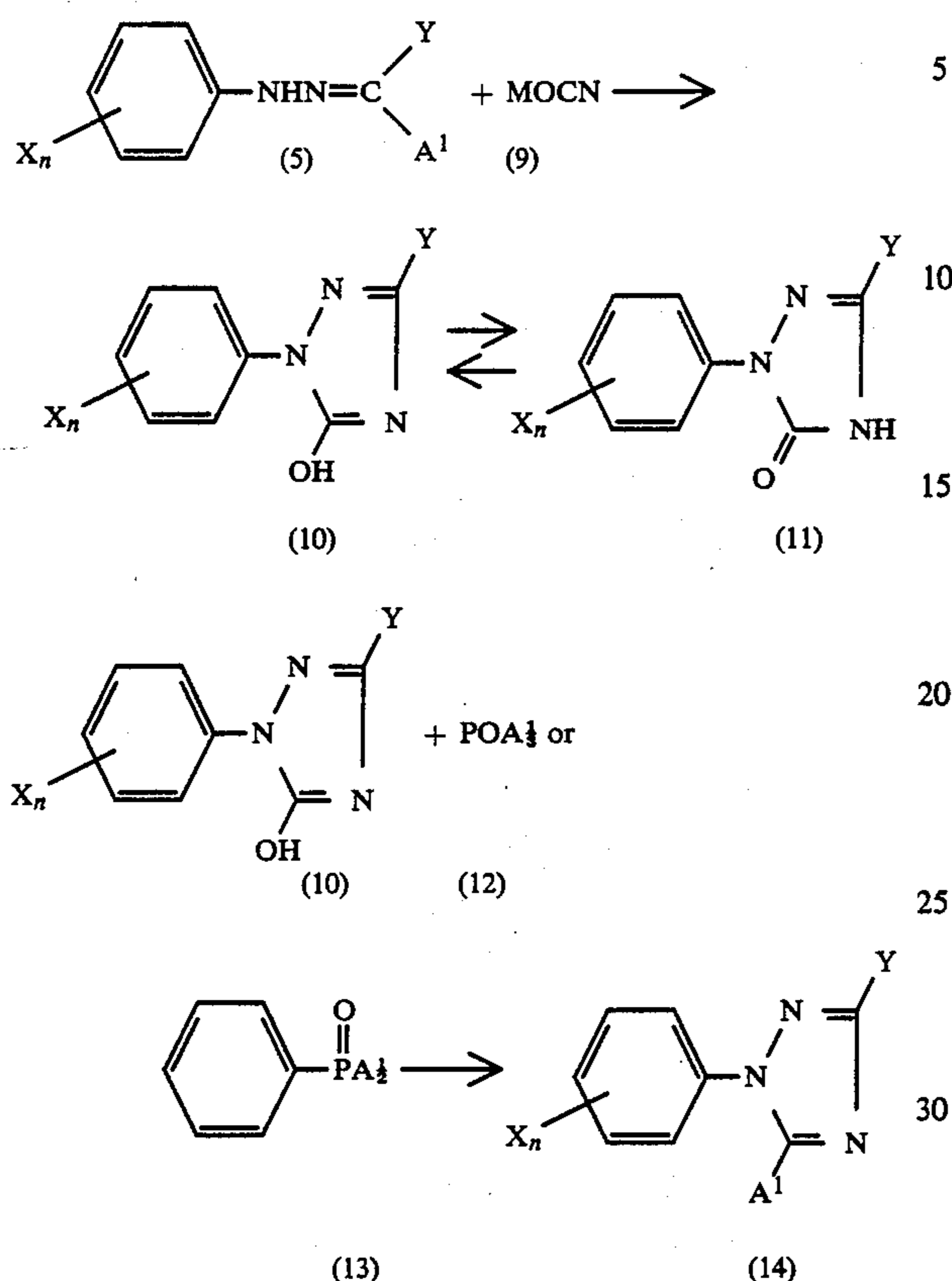
Reaction scheme 3
