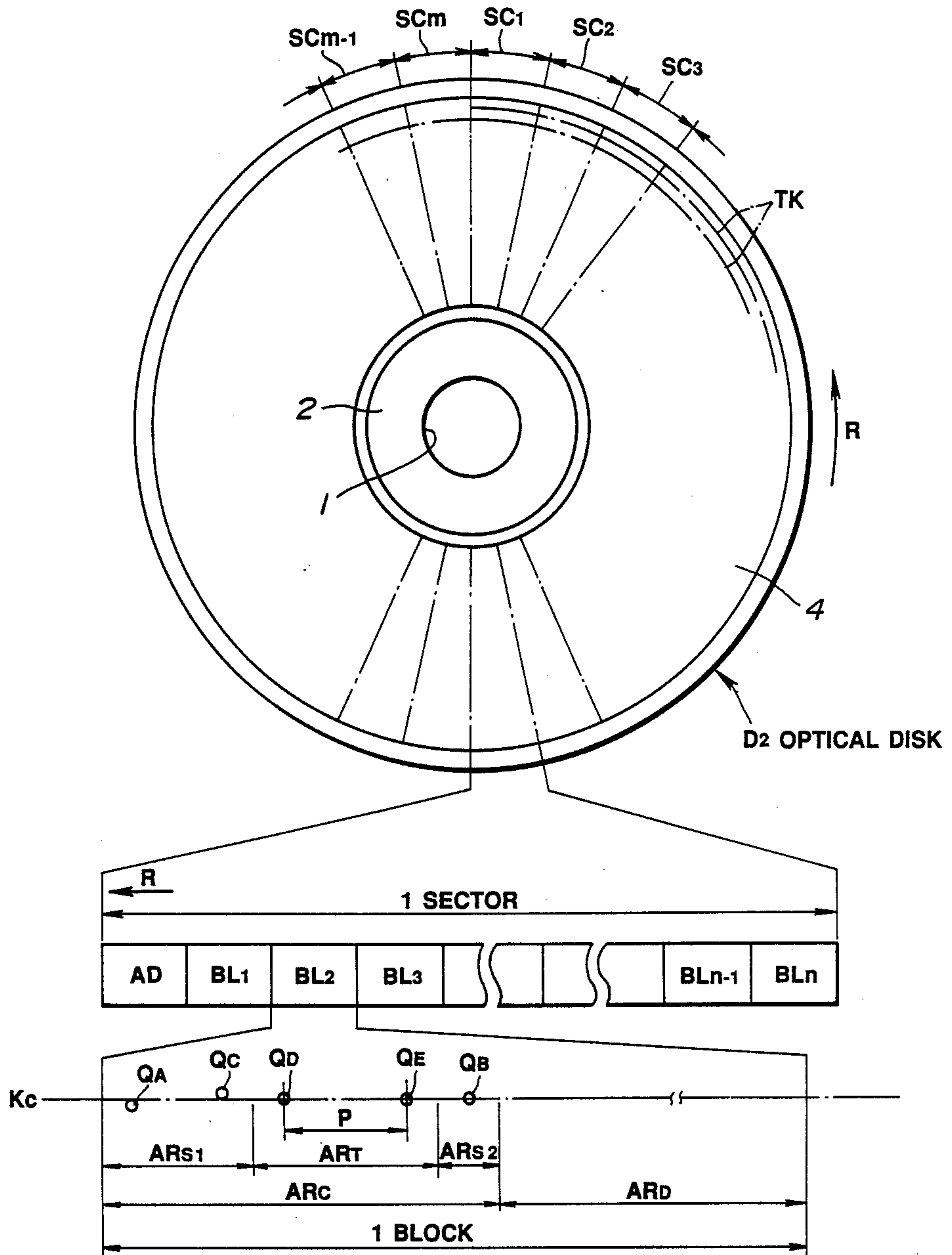
RECORDING FORMAT OF OPTICAL DISK
