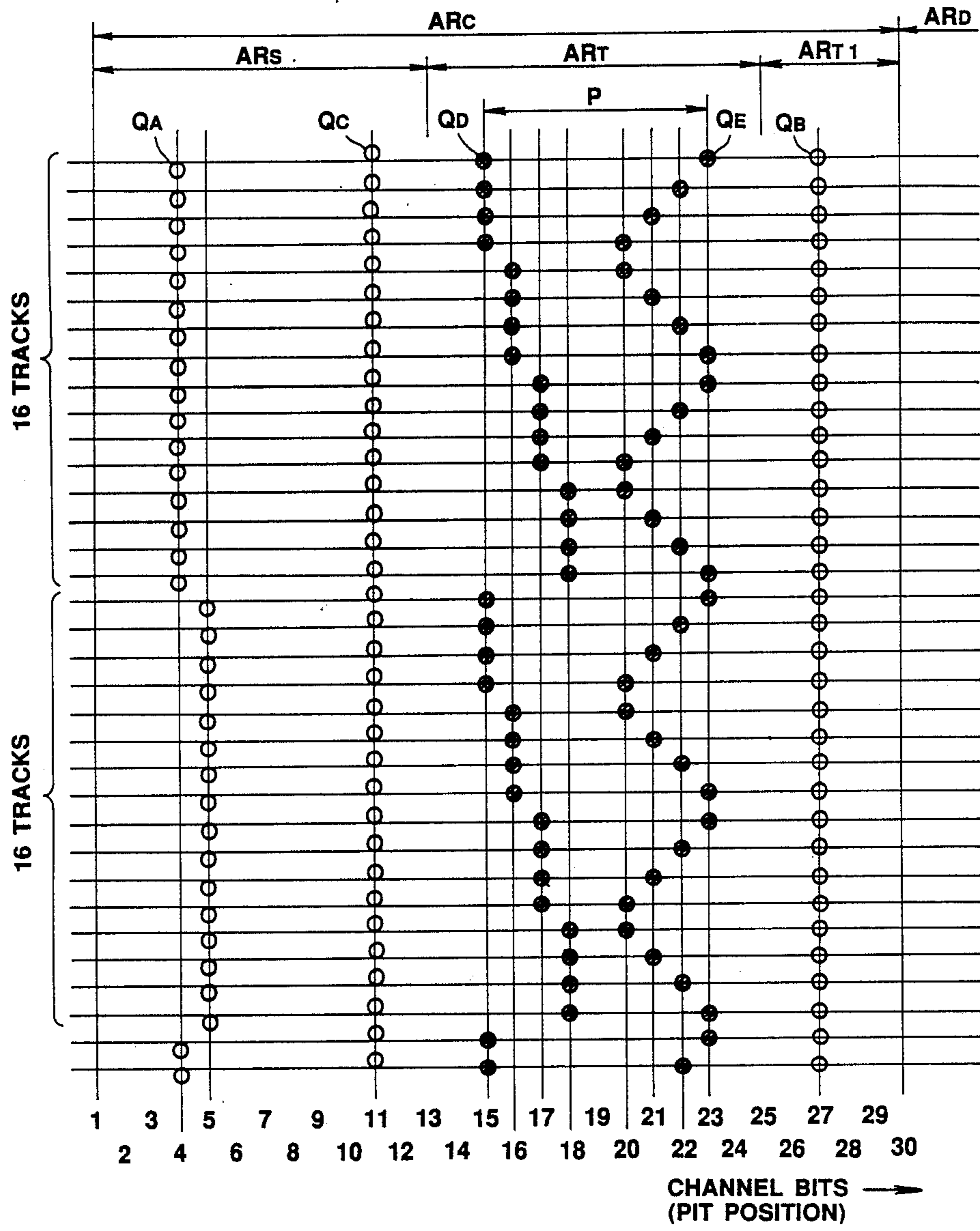
RECORDING STATE OF CONTROL RECORDING REGION
