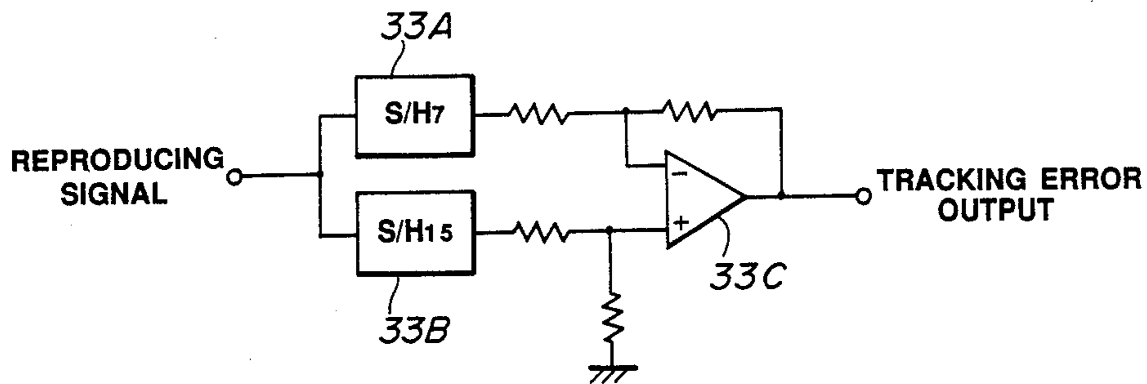
TRACKING ERROR DETECTION CIRCUIT
