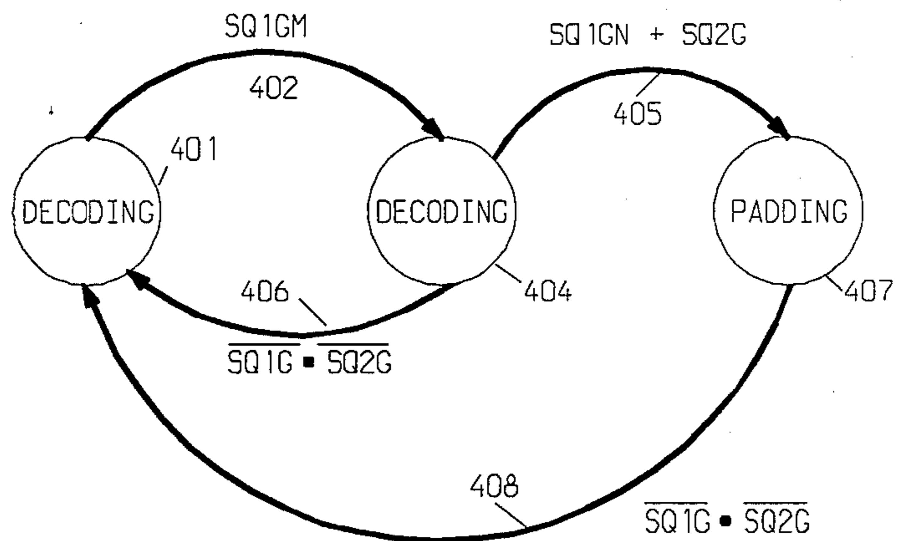
FIG. 4 CODEC CONTROLLER DECOMPRESSOR STATE DIAGRAM
