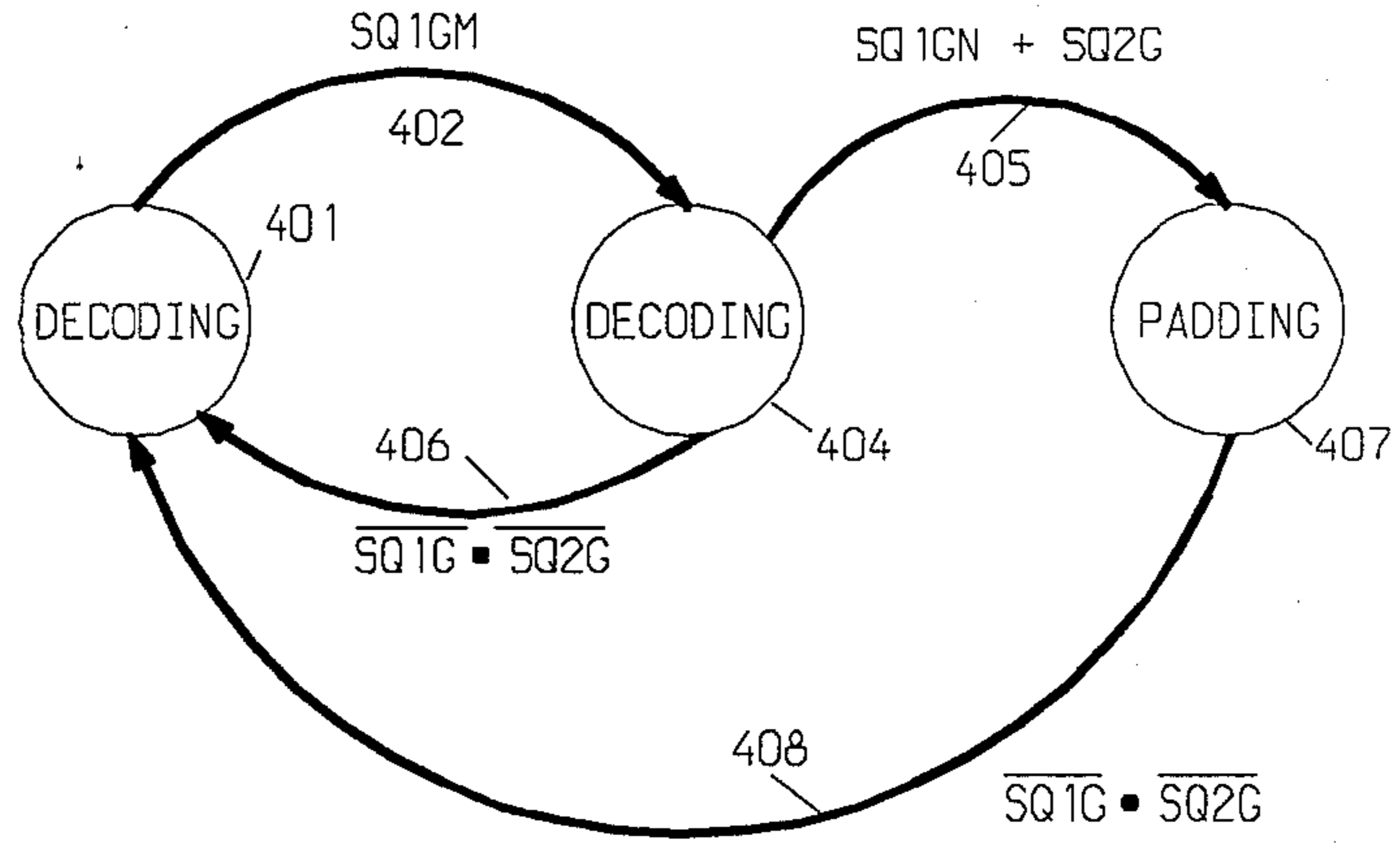
FIG. 4 CODEC CONTROLLER DECOMPRESSOR STATE DIAGRAM
