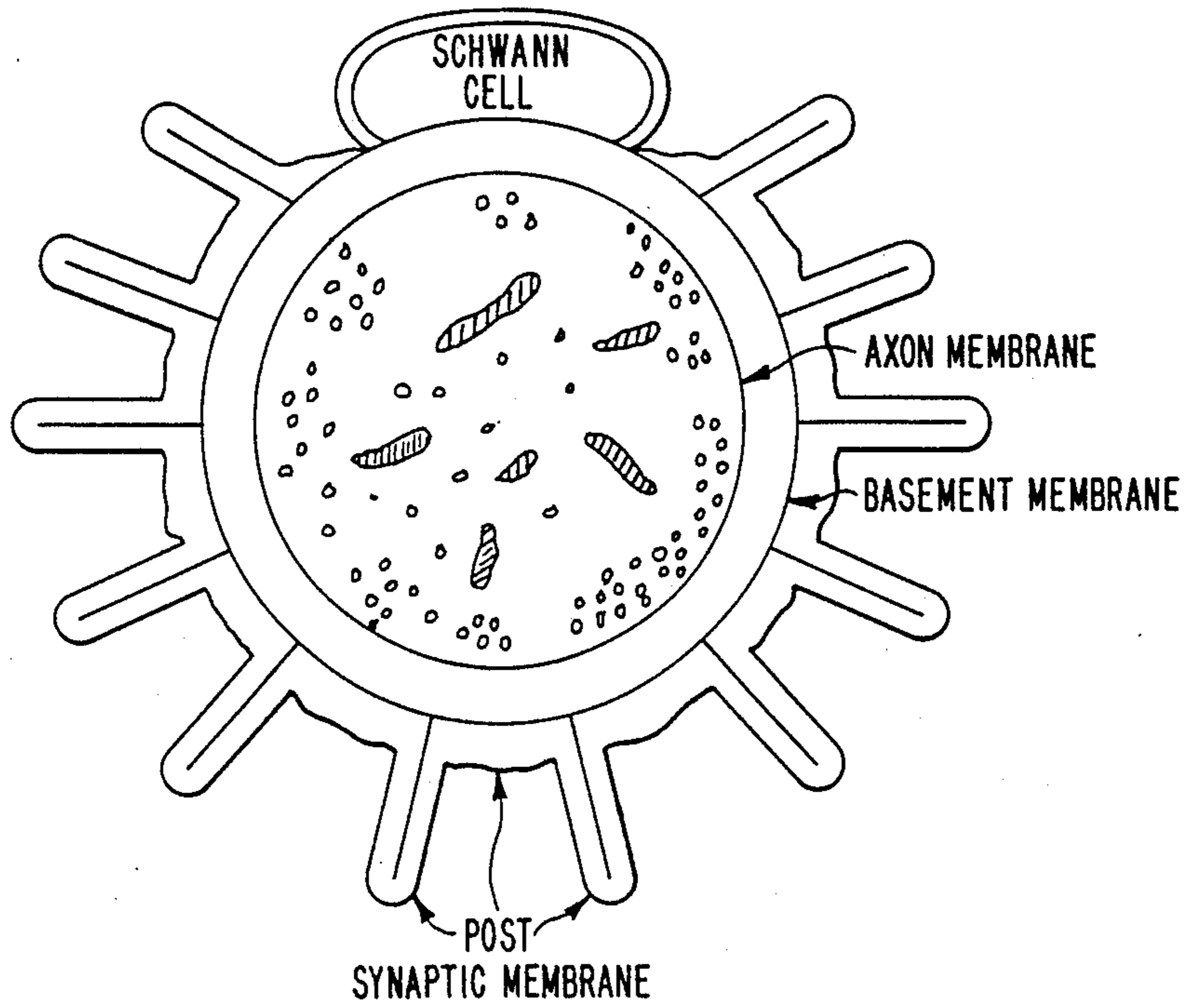
FIG. 2 NEUROMUSCULAR JUNCTION
