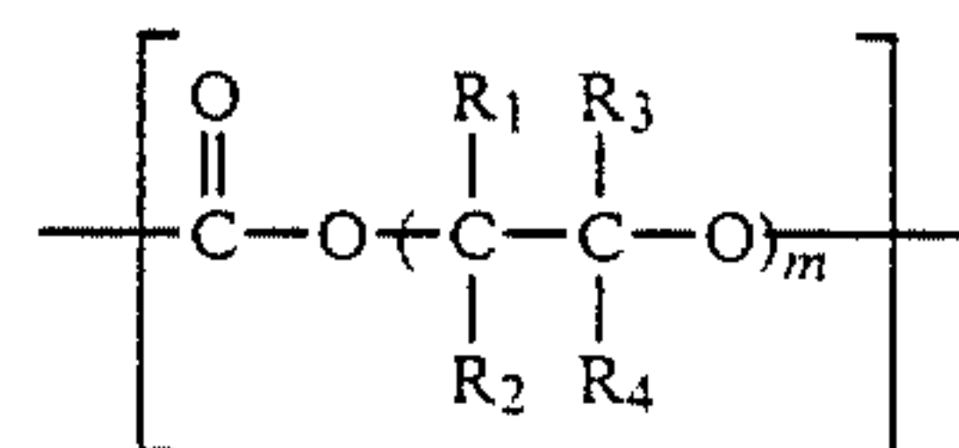
Structure III
