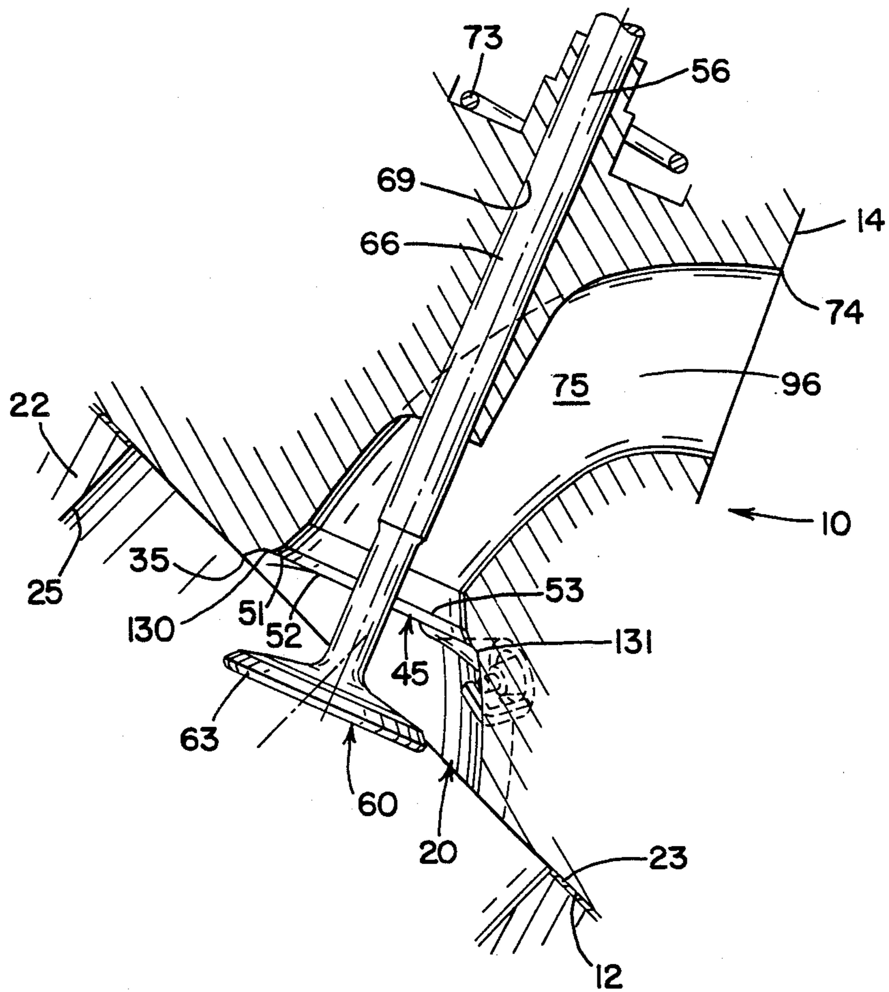
FIG. II (EXHAUST)
