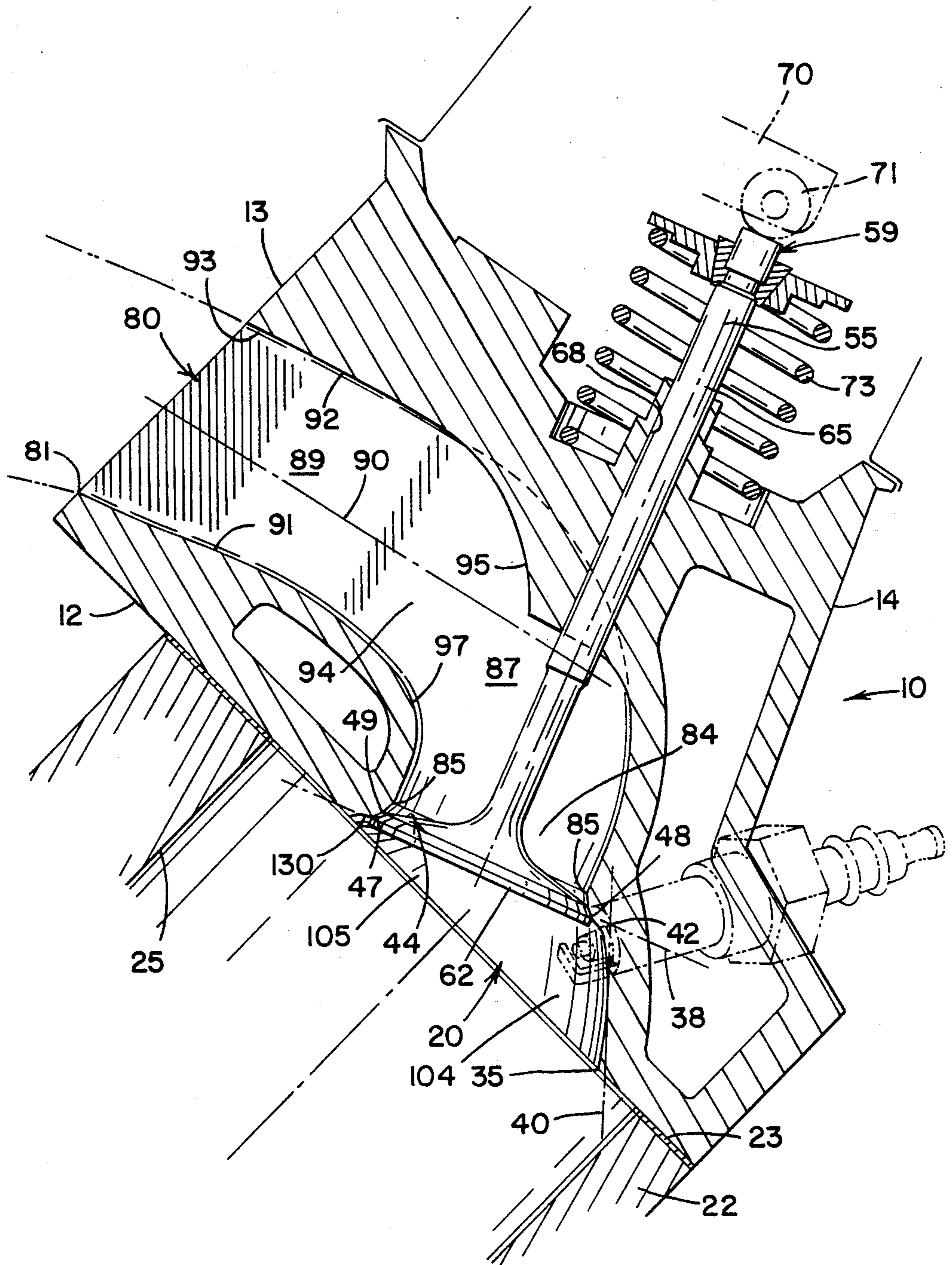
FIG. 4 (INTAKE)
