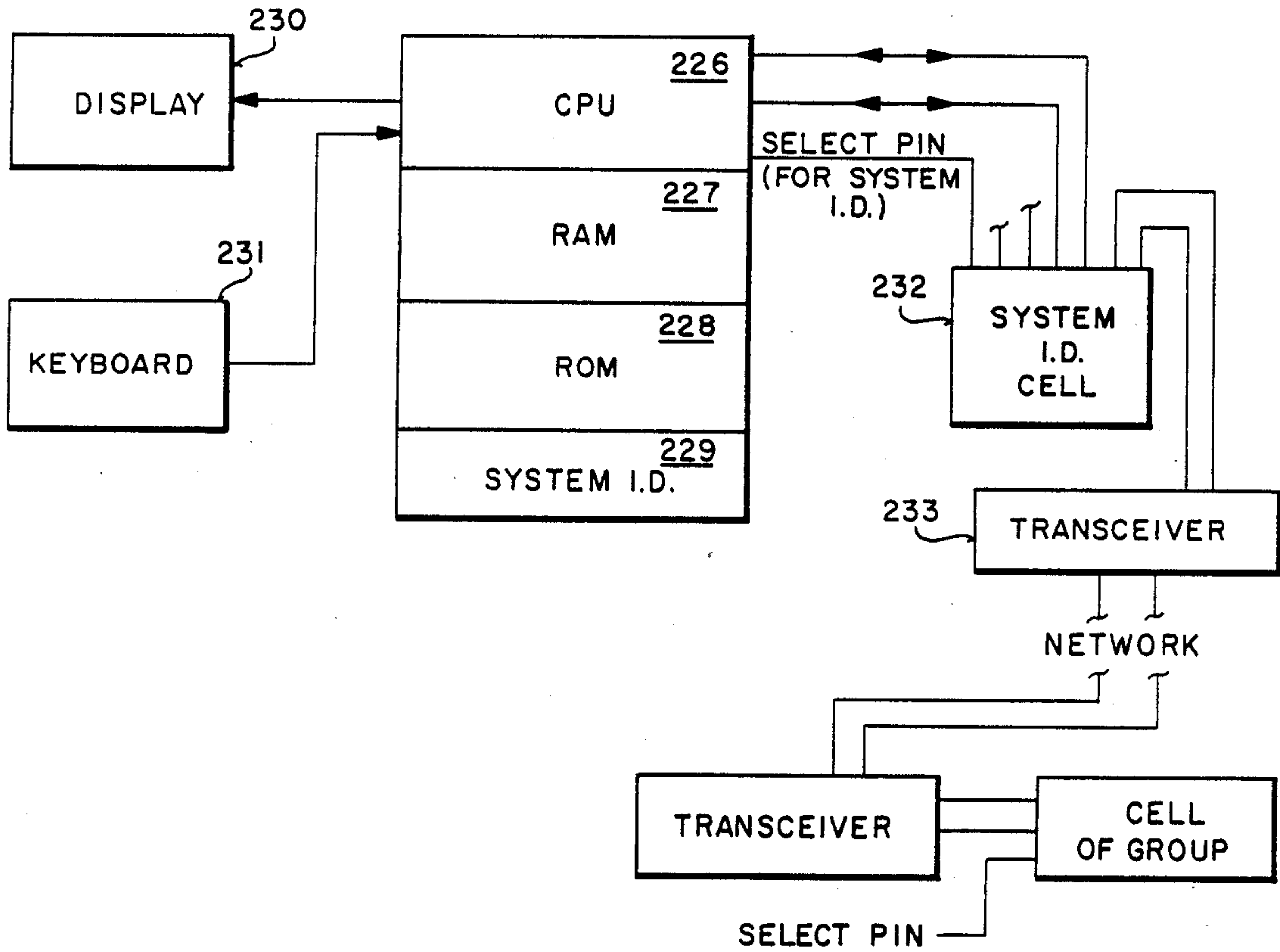
FIG 28 GROUPING DEVICE
