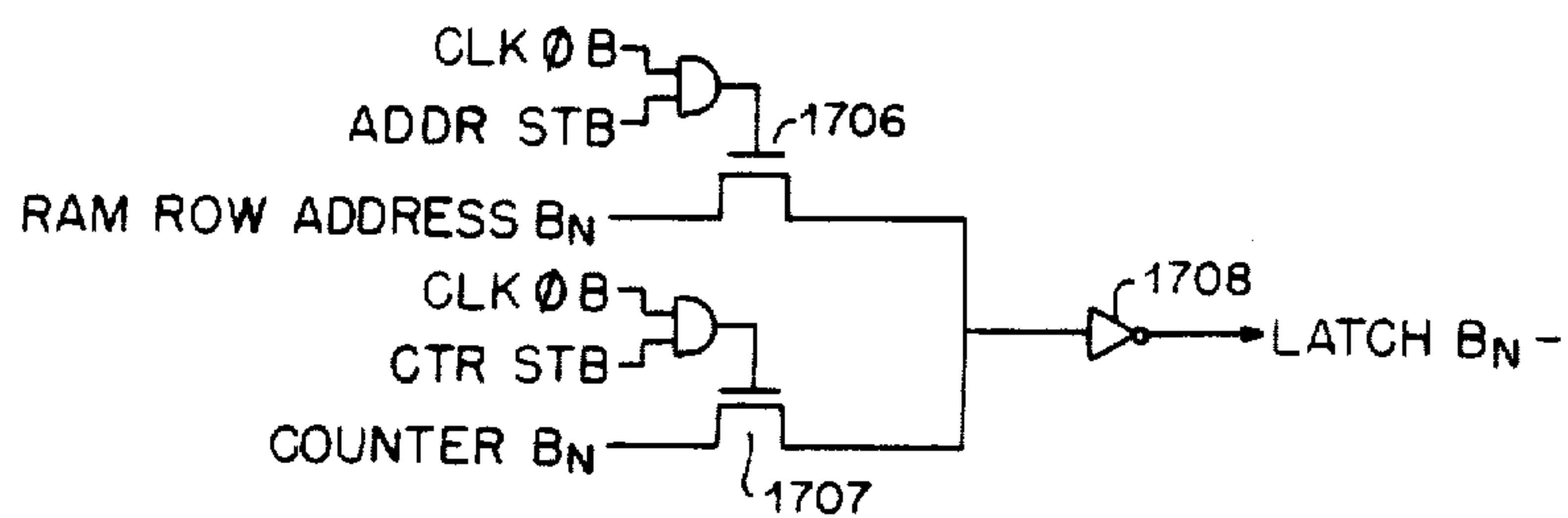
FIG. 14B. MUX/LATCH DETAIL
