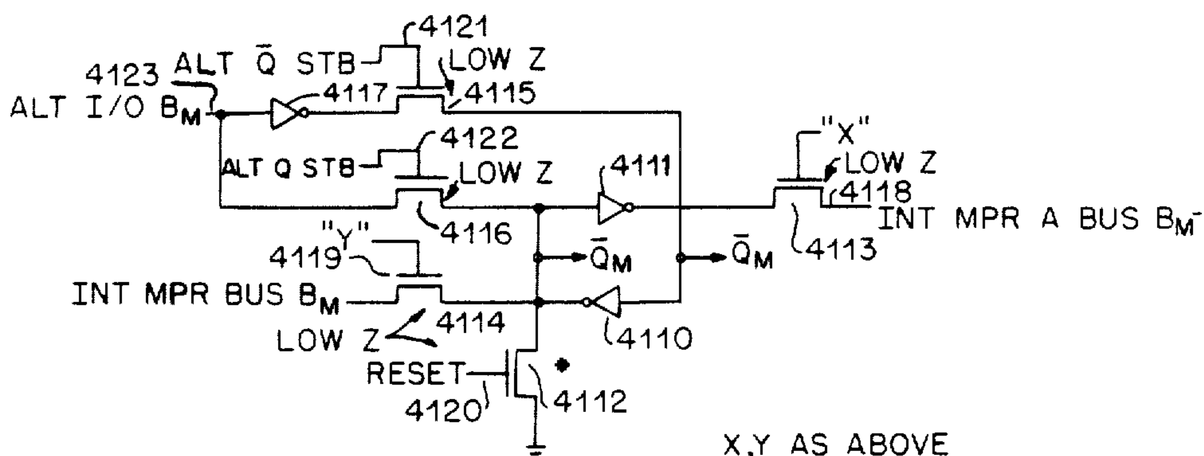
MPR FIG. 20B. ALTERNATE INPUTS
