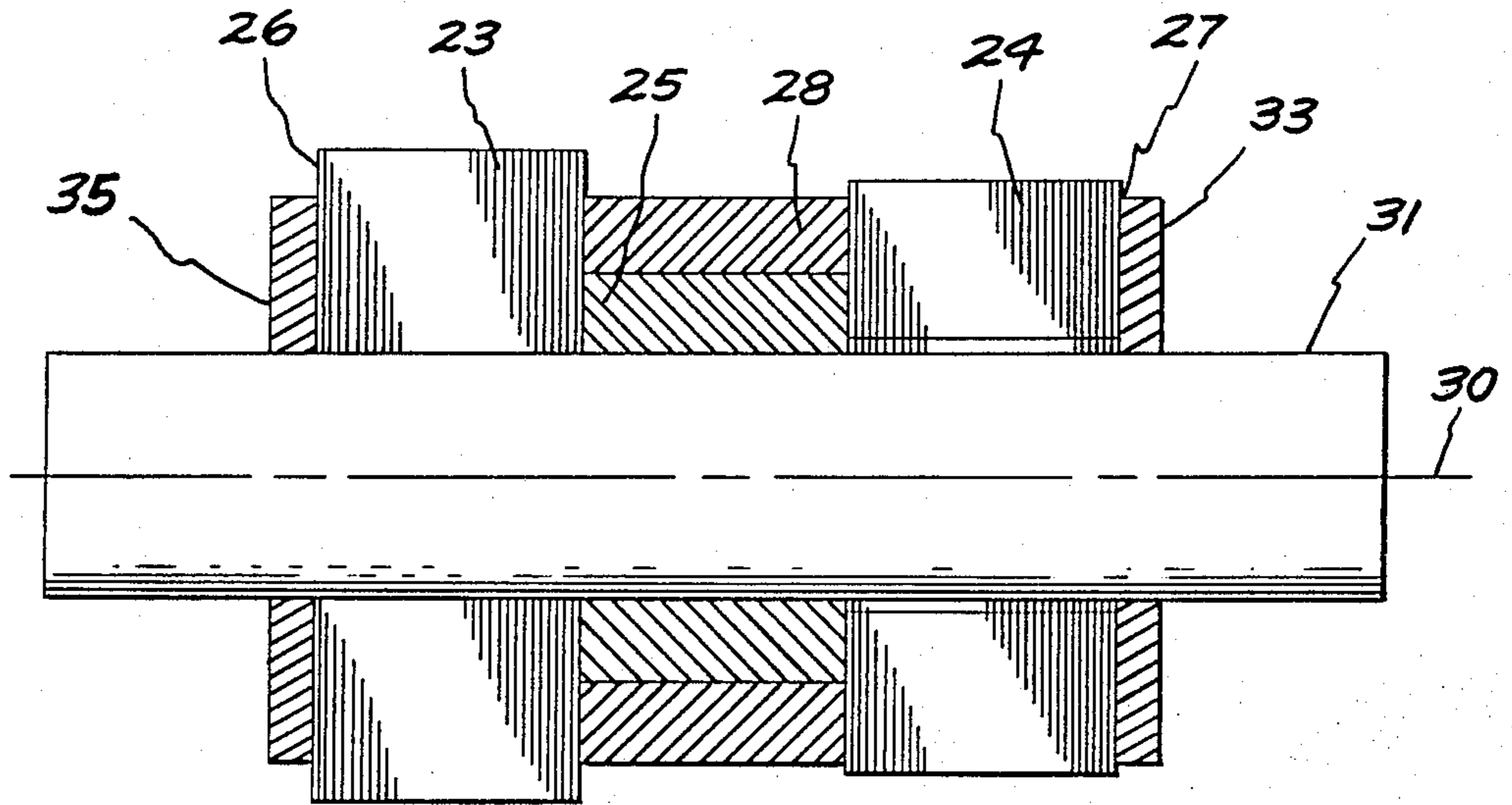
FIG. 3 (PRIOR ART)
