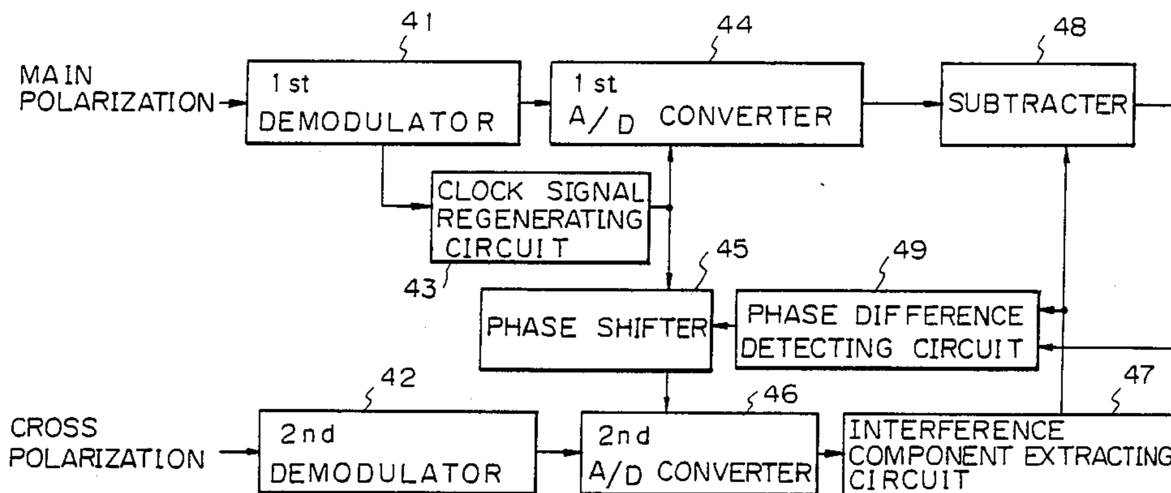
PRINCIPAL BLOCK DIAGRAM OF INVENTION
