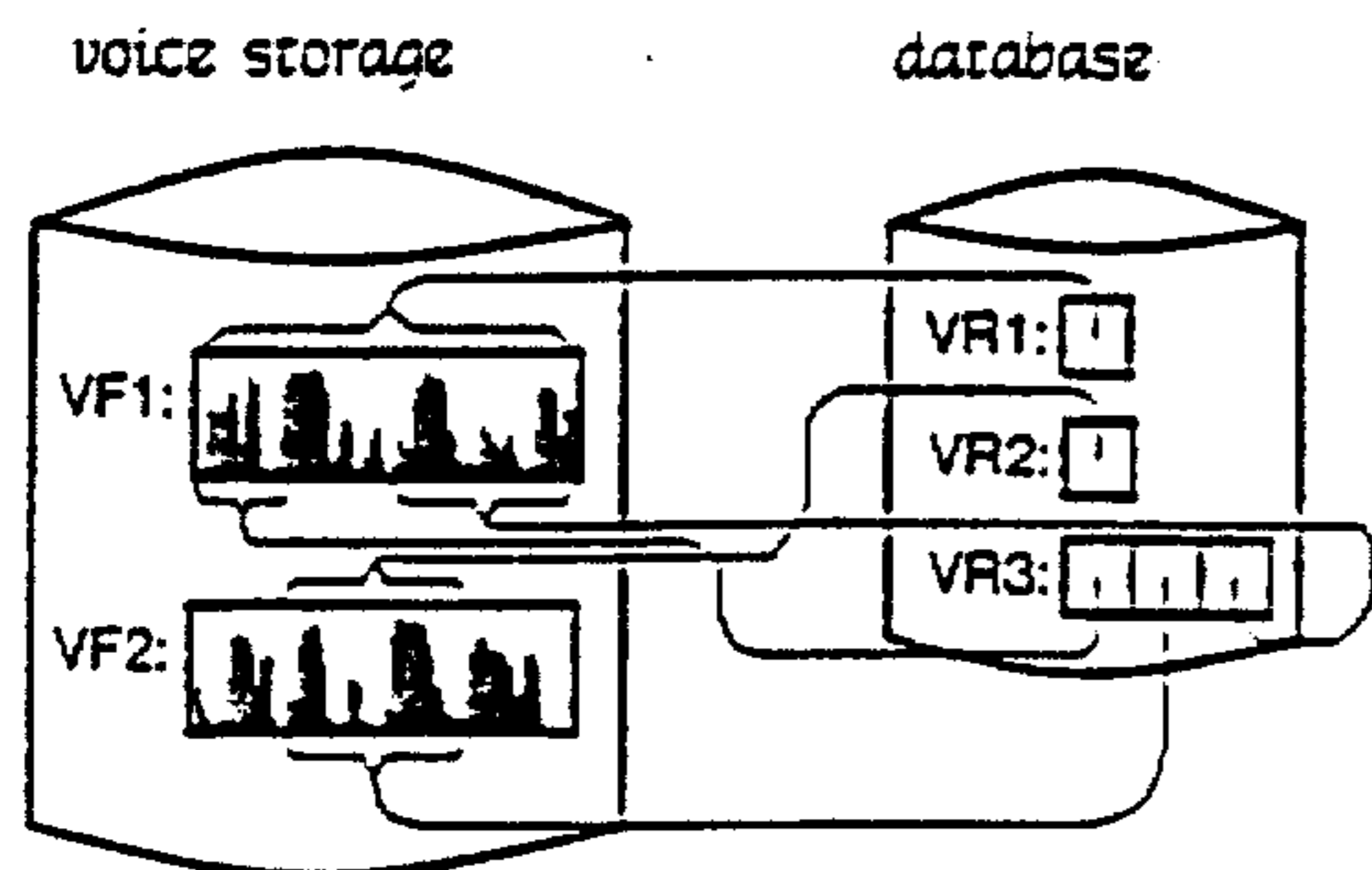
Figure 4. Structure of VR 3 after REPLACE operation.
