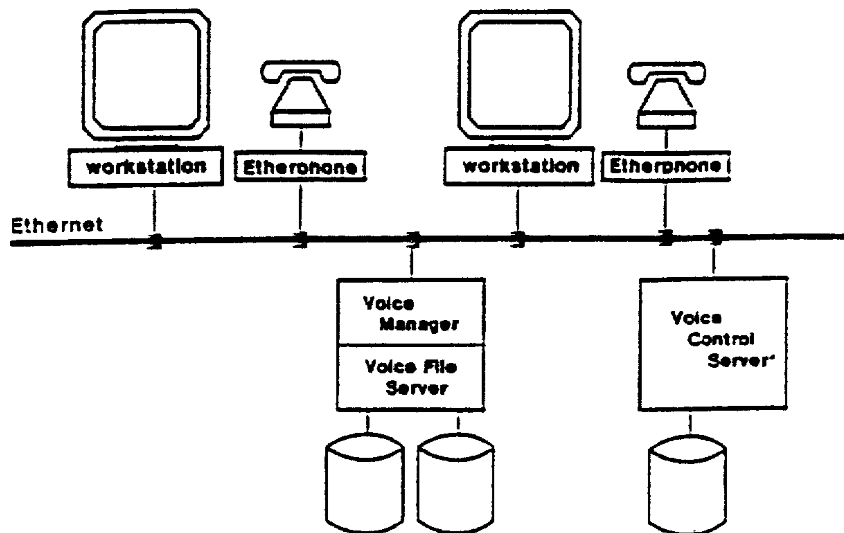
Figure 1. A simple Etherphone system environment.
