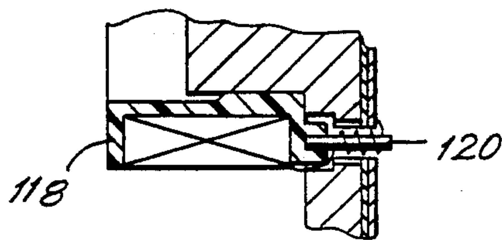
FIG. 10 PRIOR ART
