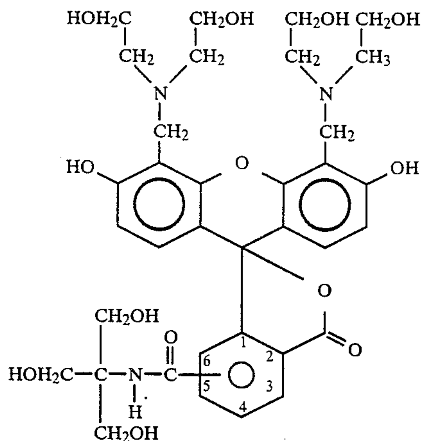
5(6)-carboxyfluorescein-tris(methylol)methylamide-4',5'-bis(methylenediethanolamine)
