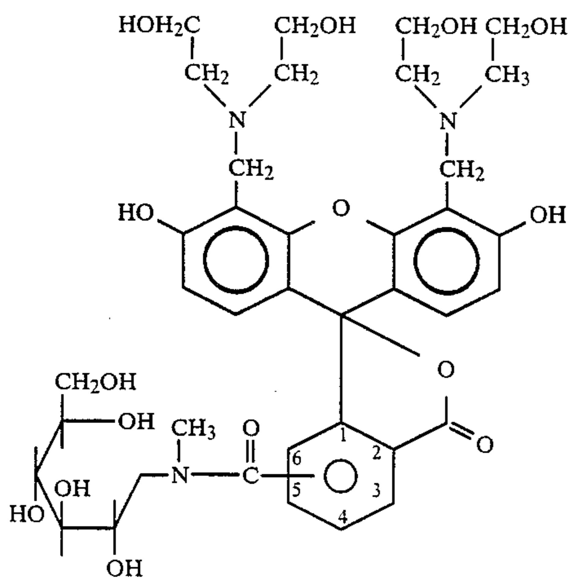
5(6)-carboxyfluorescein-N-methylglucamide-4',5'-bis(methylenediethanolamine)
