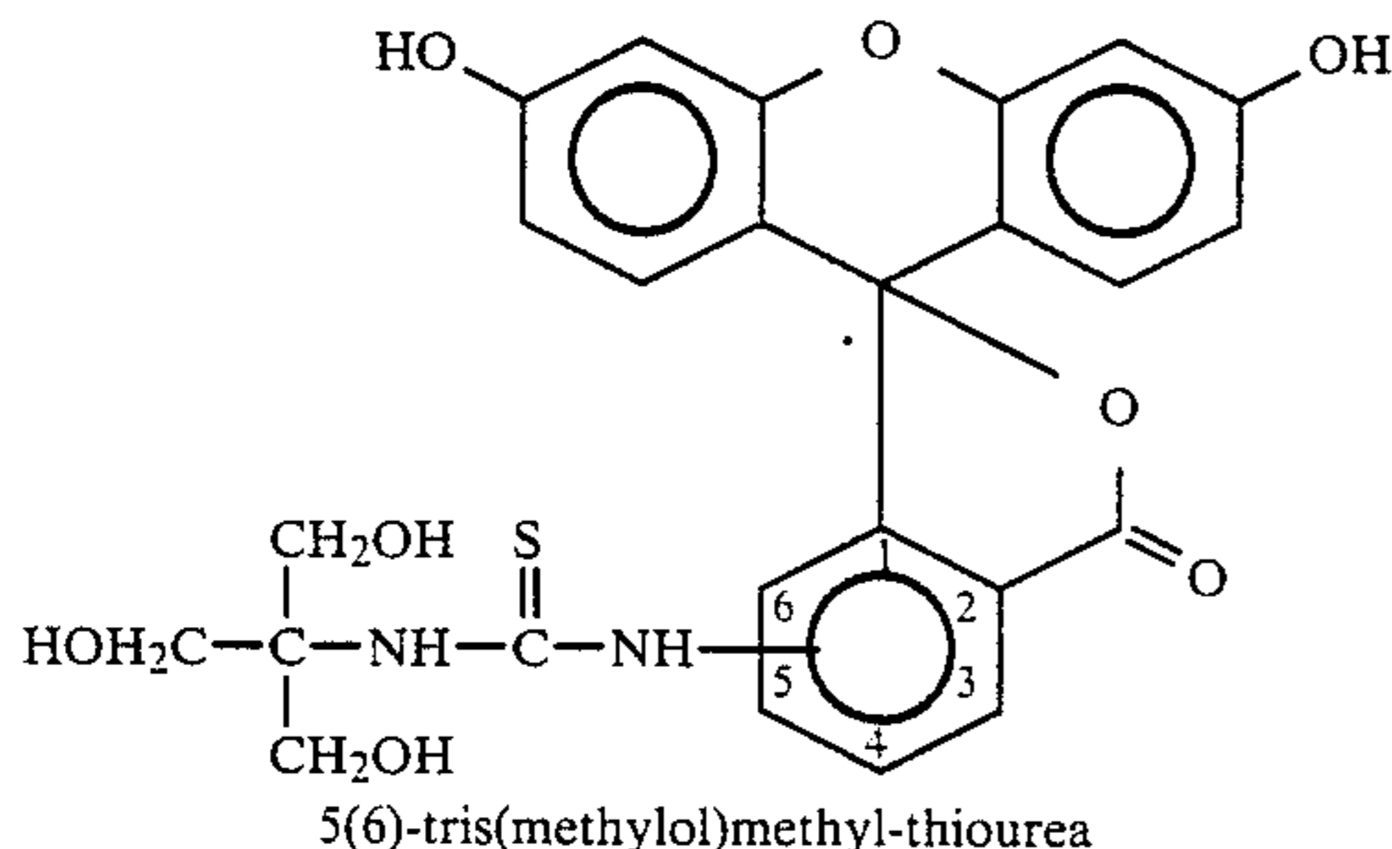
5(6)-tris(methylol)methyl-thiourea
