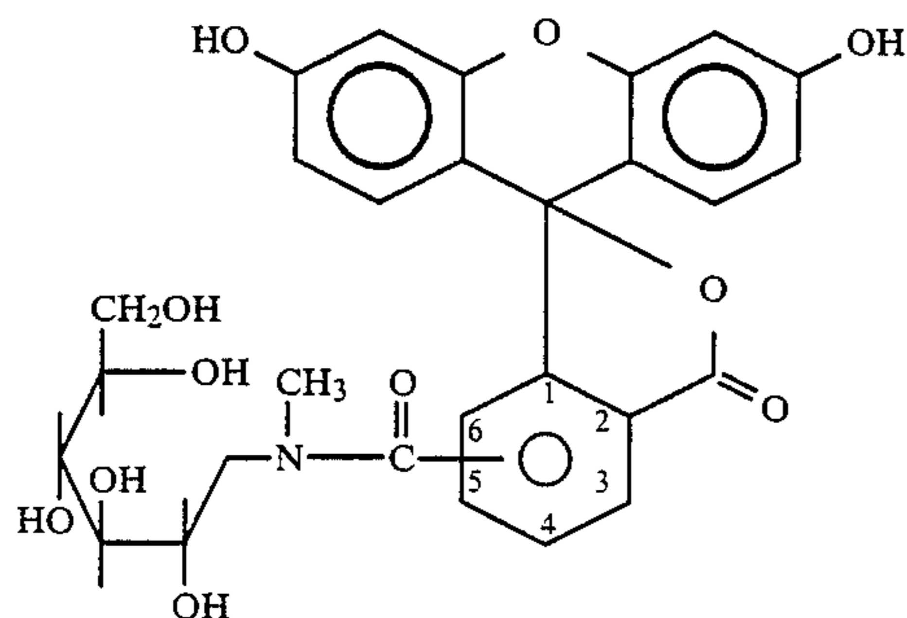
5(6)-carboxyfluorescein-N-methylglucamide
