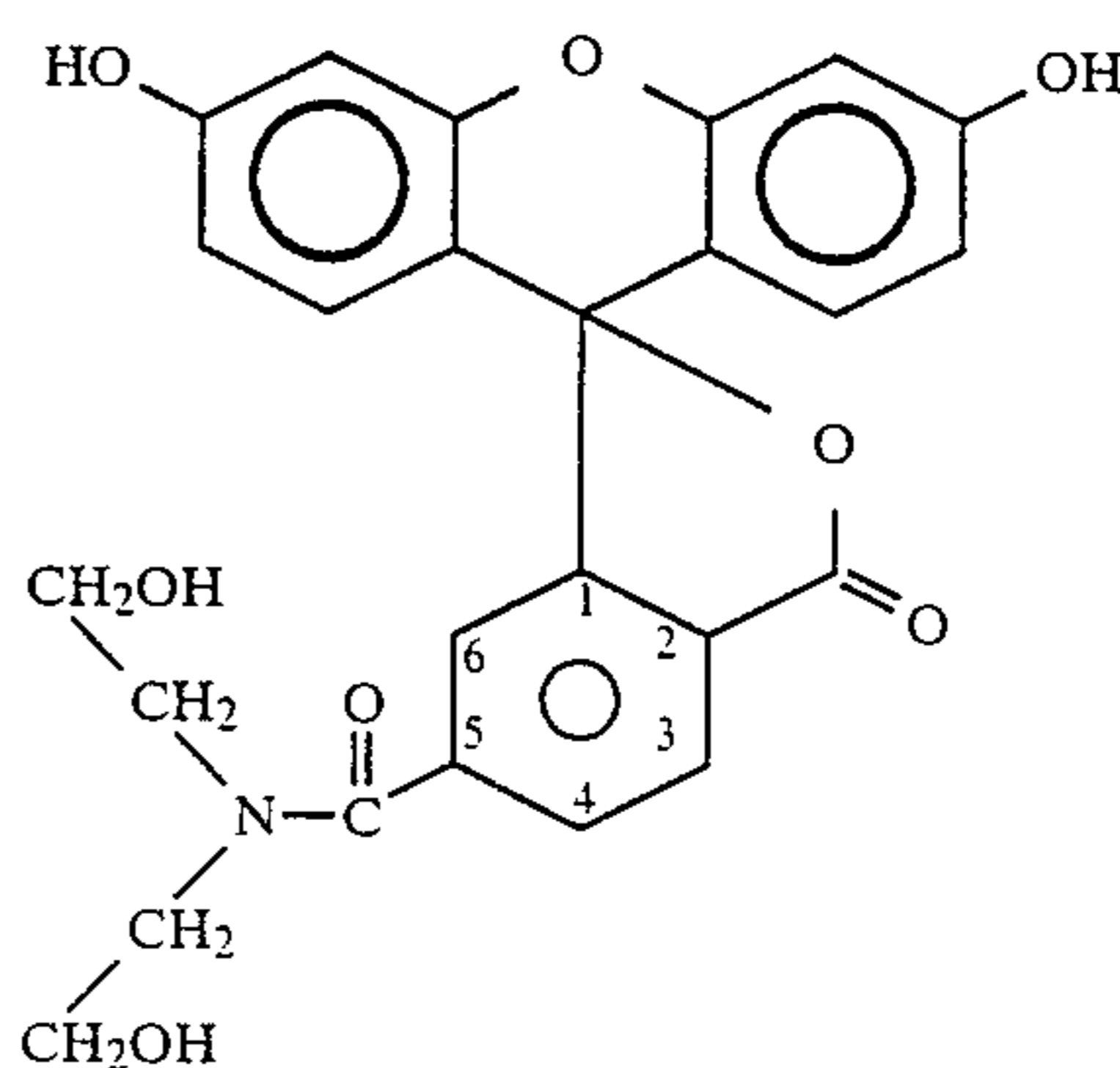
5-carboxyfluorescein-diethanolamide
