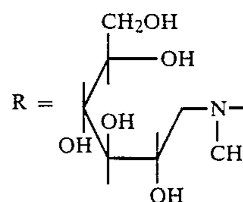
5(6)-carboxyfluorescein-N-methylglucamide-4',5'-bis(N-methylglucaminomethyl)
