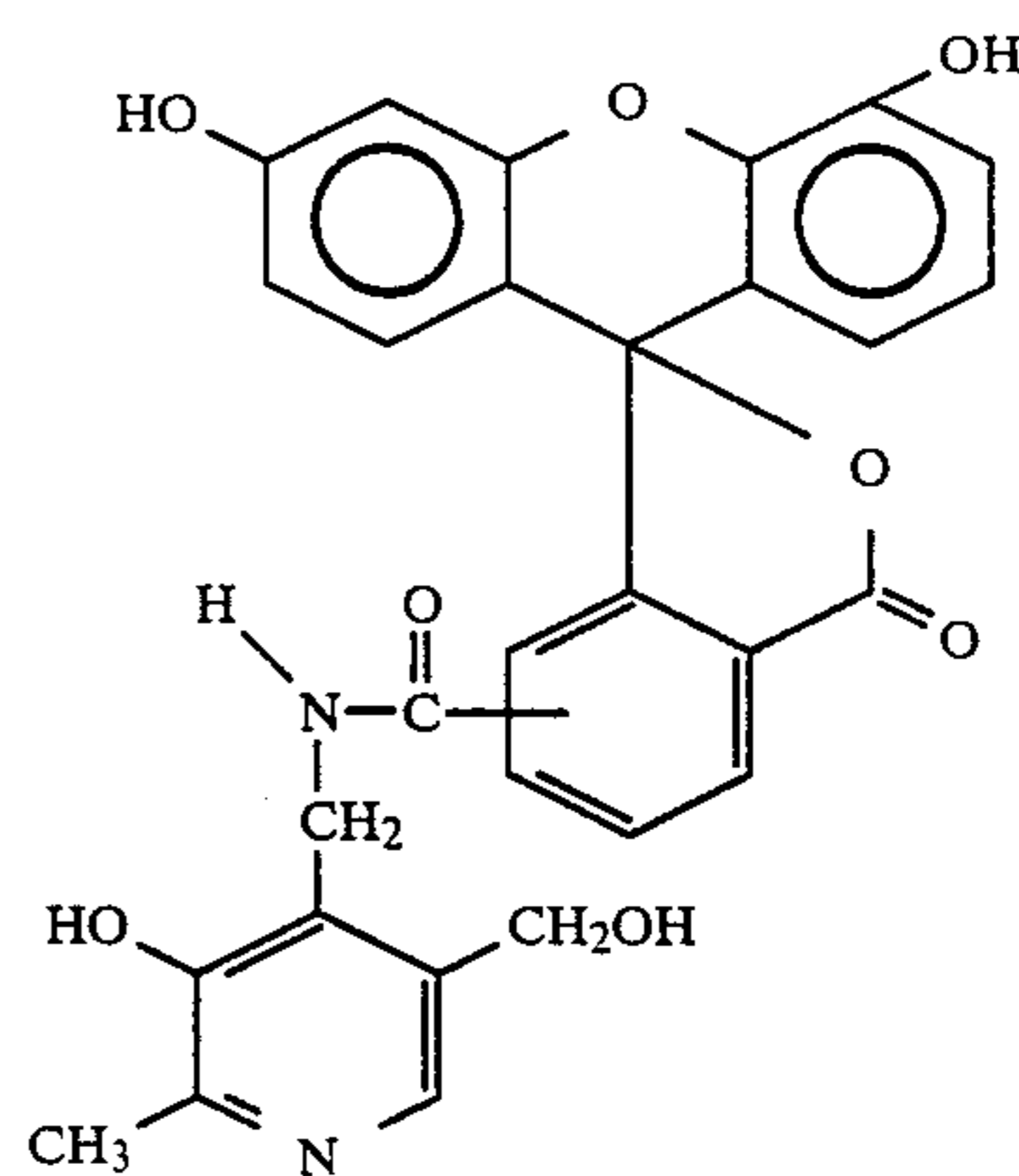
5(6)-carboxyfluorescein-pyridoxamide
