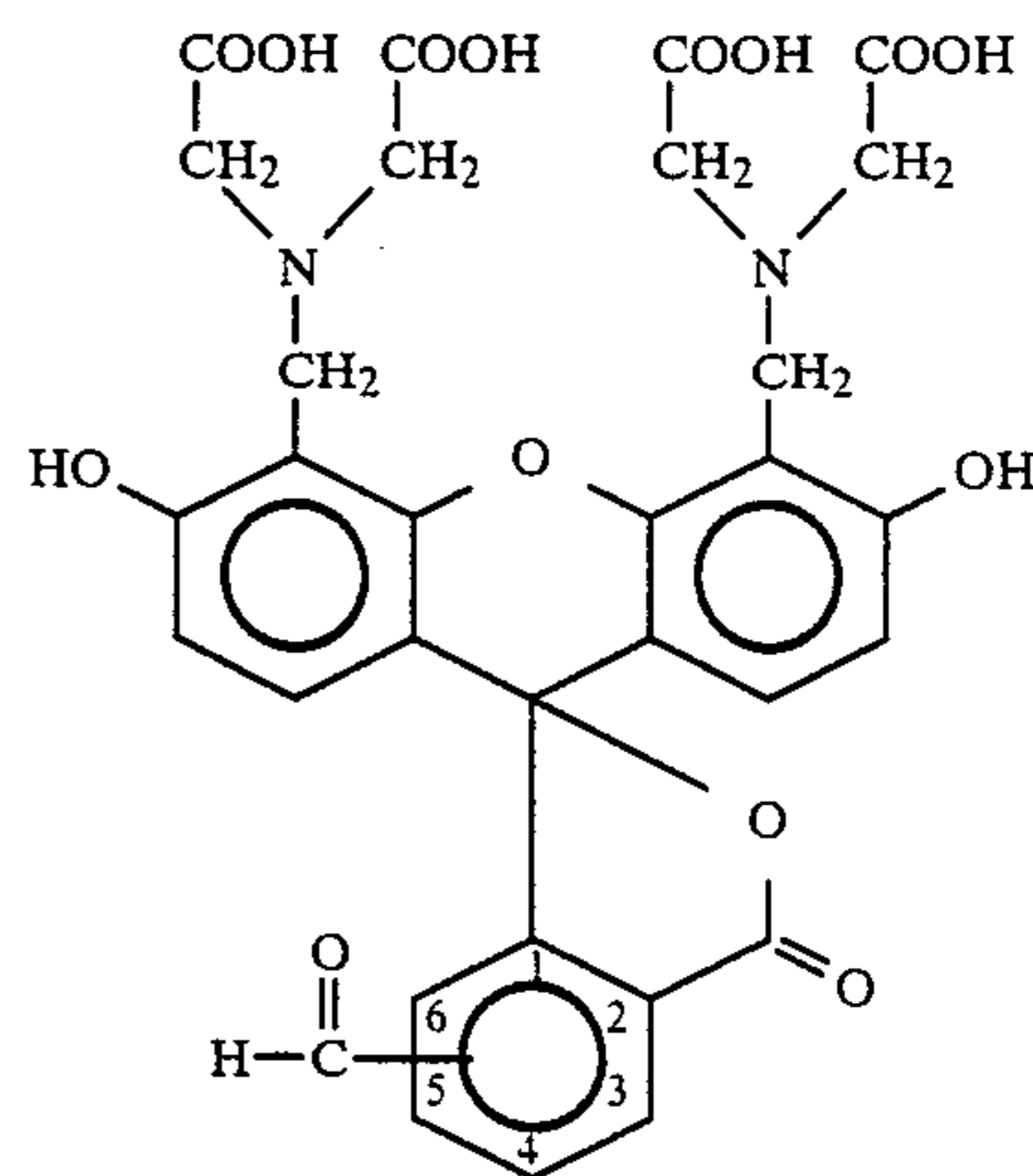
5(6)-carboxyfluorescein-4',5'-bis(methyleneiminodiacetic acid)
