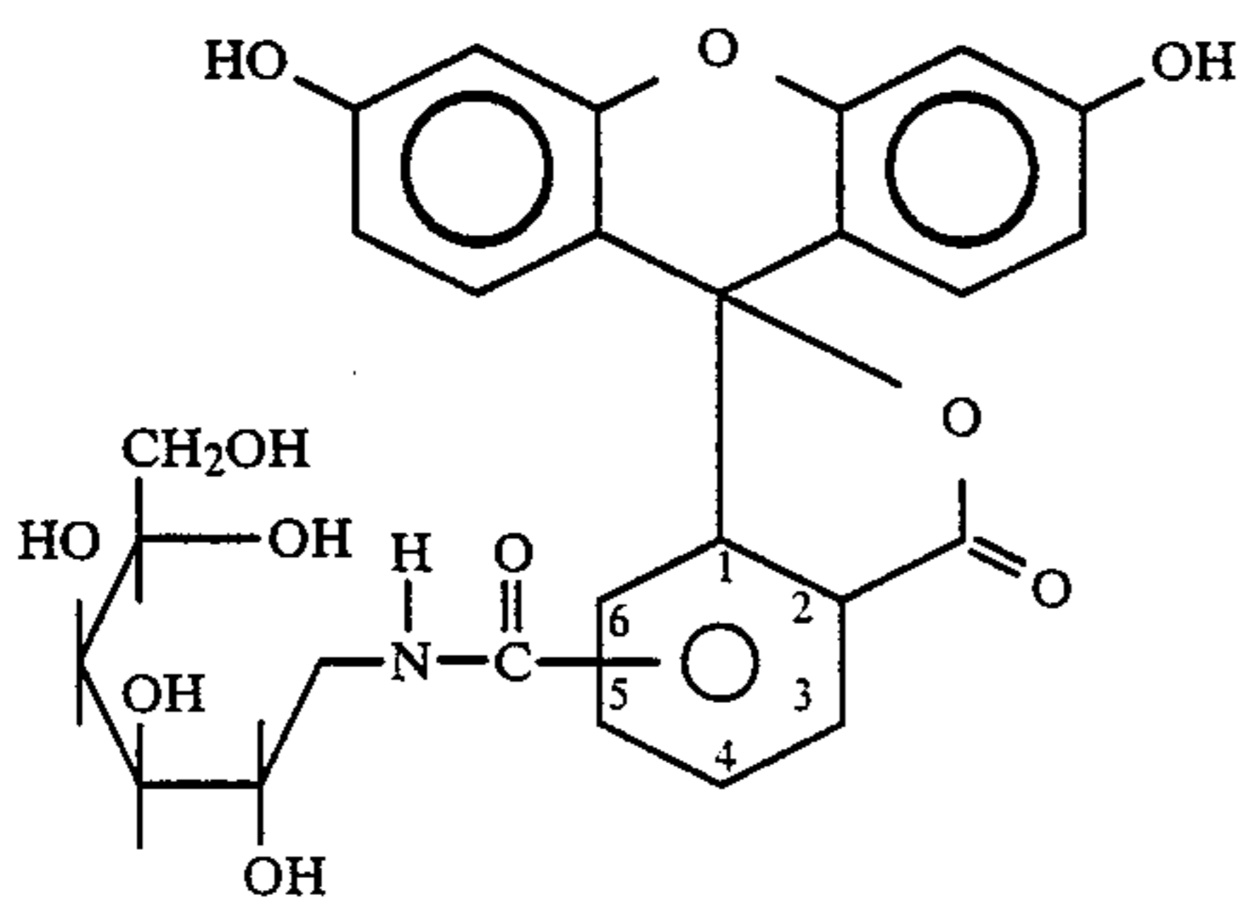
5(6)-carboxyfluorescein-galactosamide
