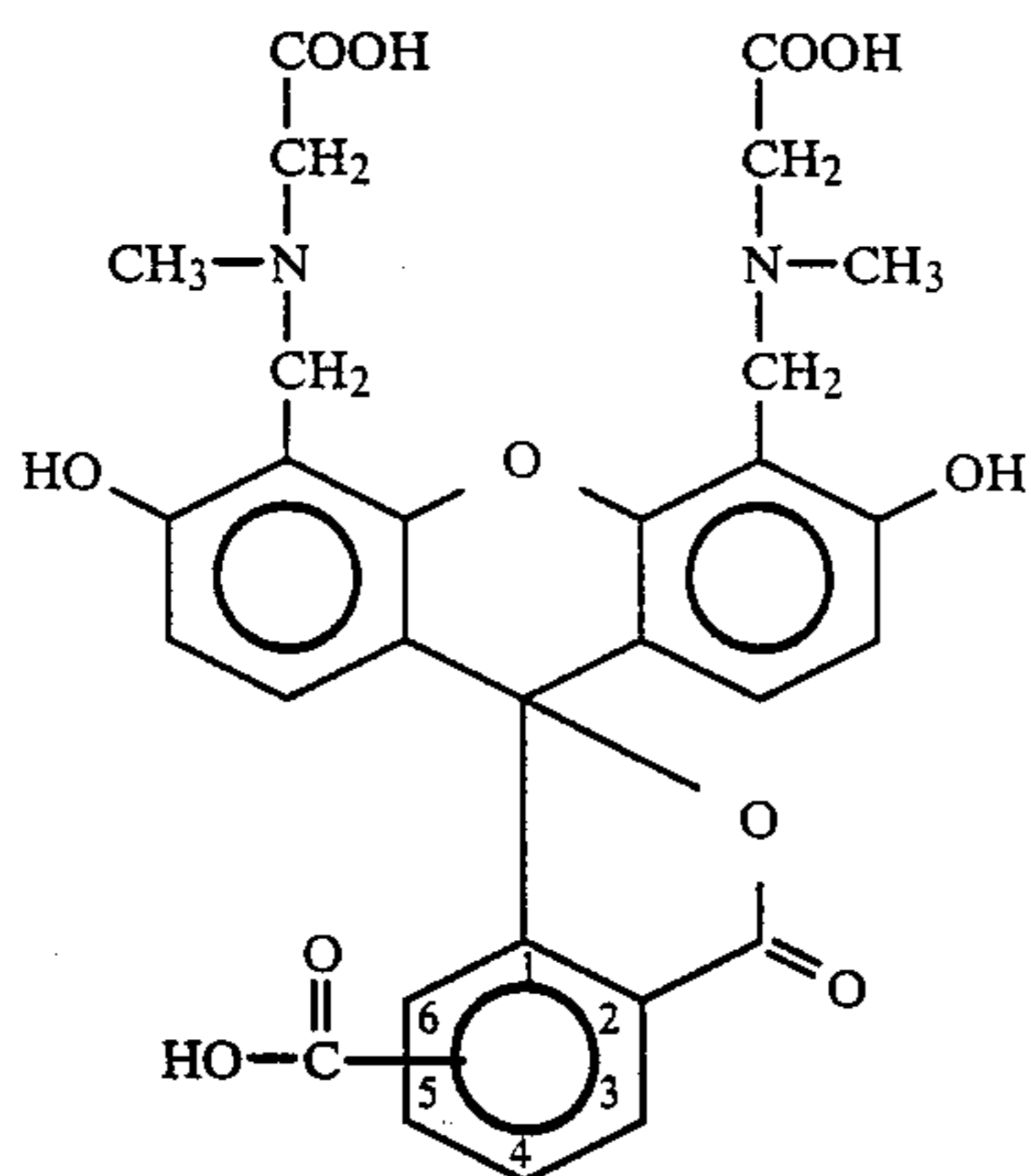
5(6)-carboxyfluorescein-4',5'-bis(methylenesarcosine)
