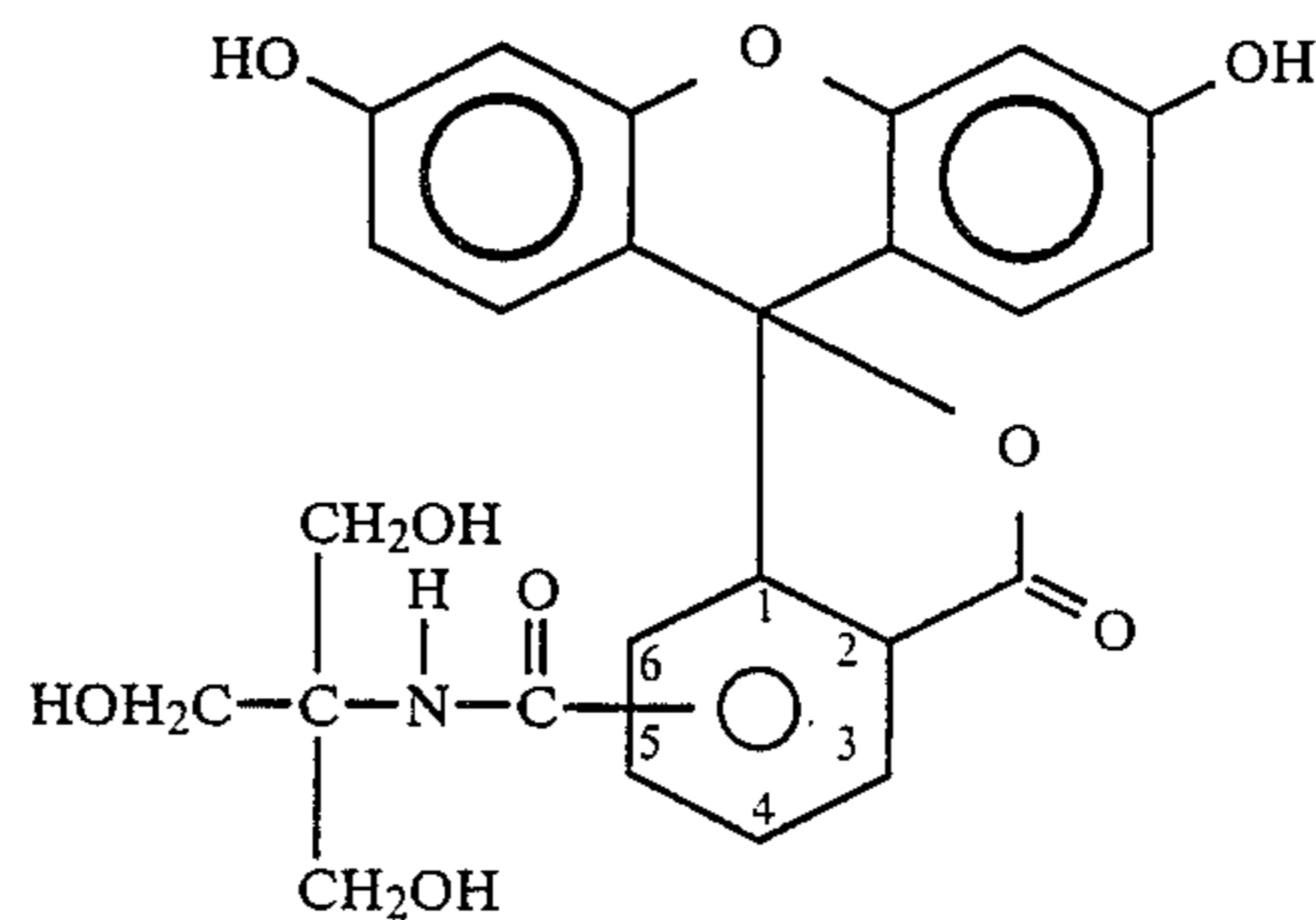
5(6)-carboxyfluorescein-tris(methylol)methylamide
