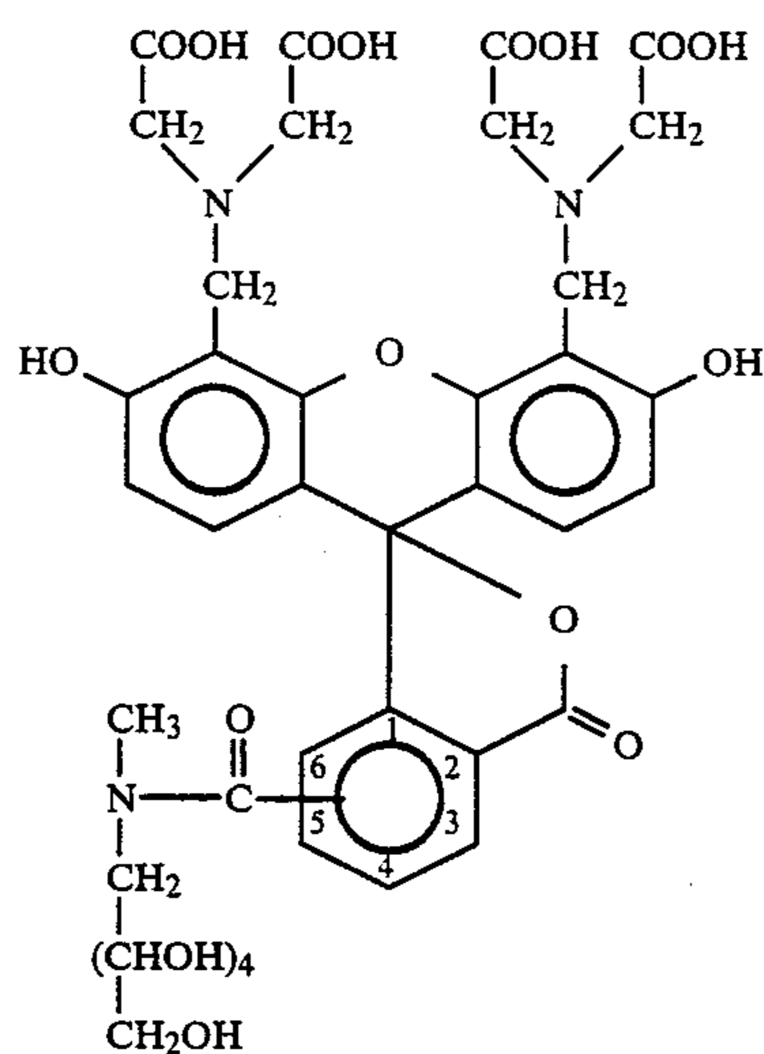
5(6)-carboxyfluorescein-N-methylglucamide-4',5'-bis(methyleneiminodiacetic acid)
