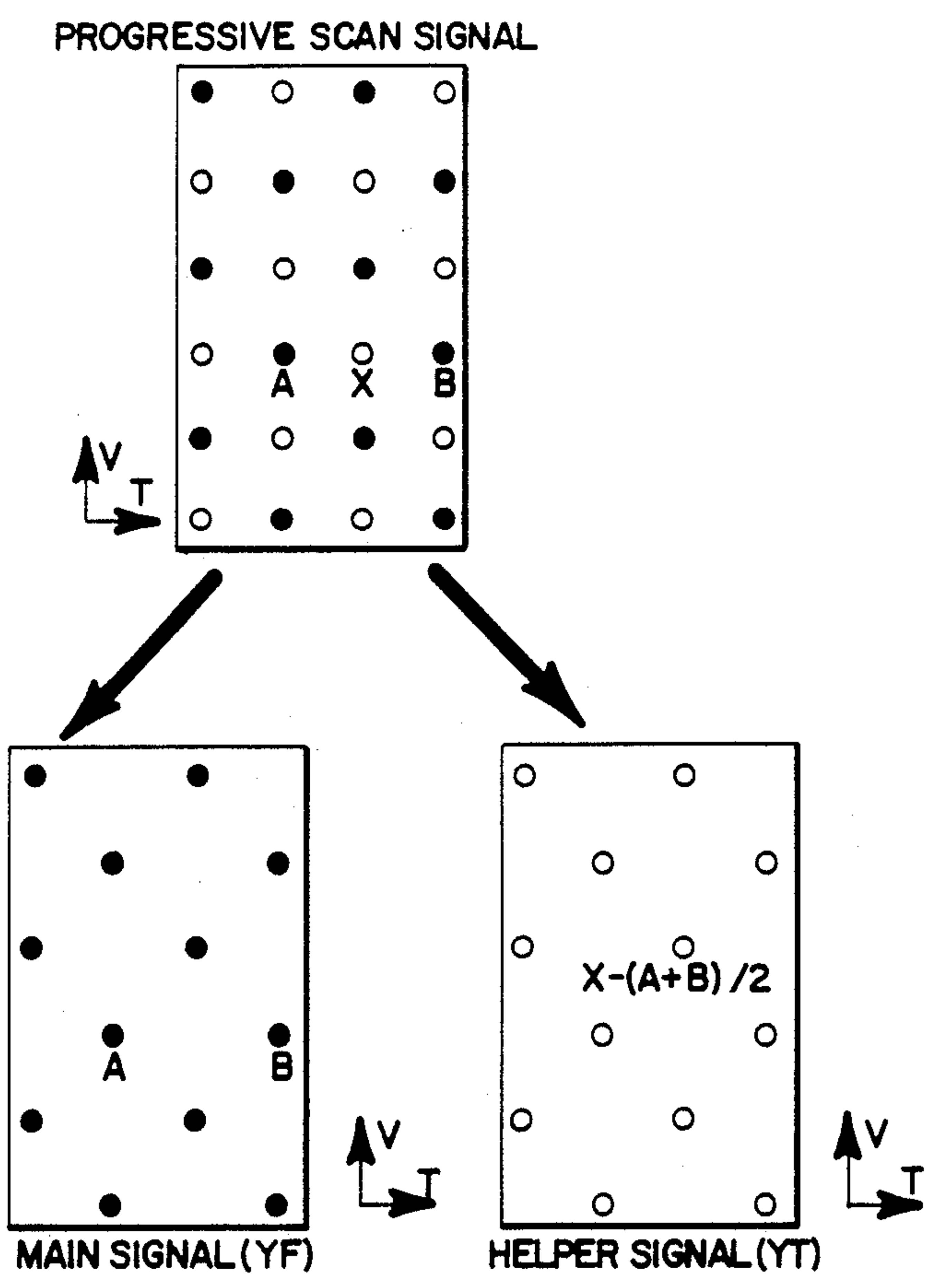
PROGRESSIVE SCAN TO 2:1 INTERLACE CONVERSION
