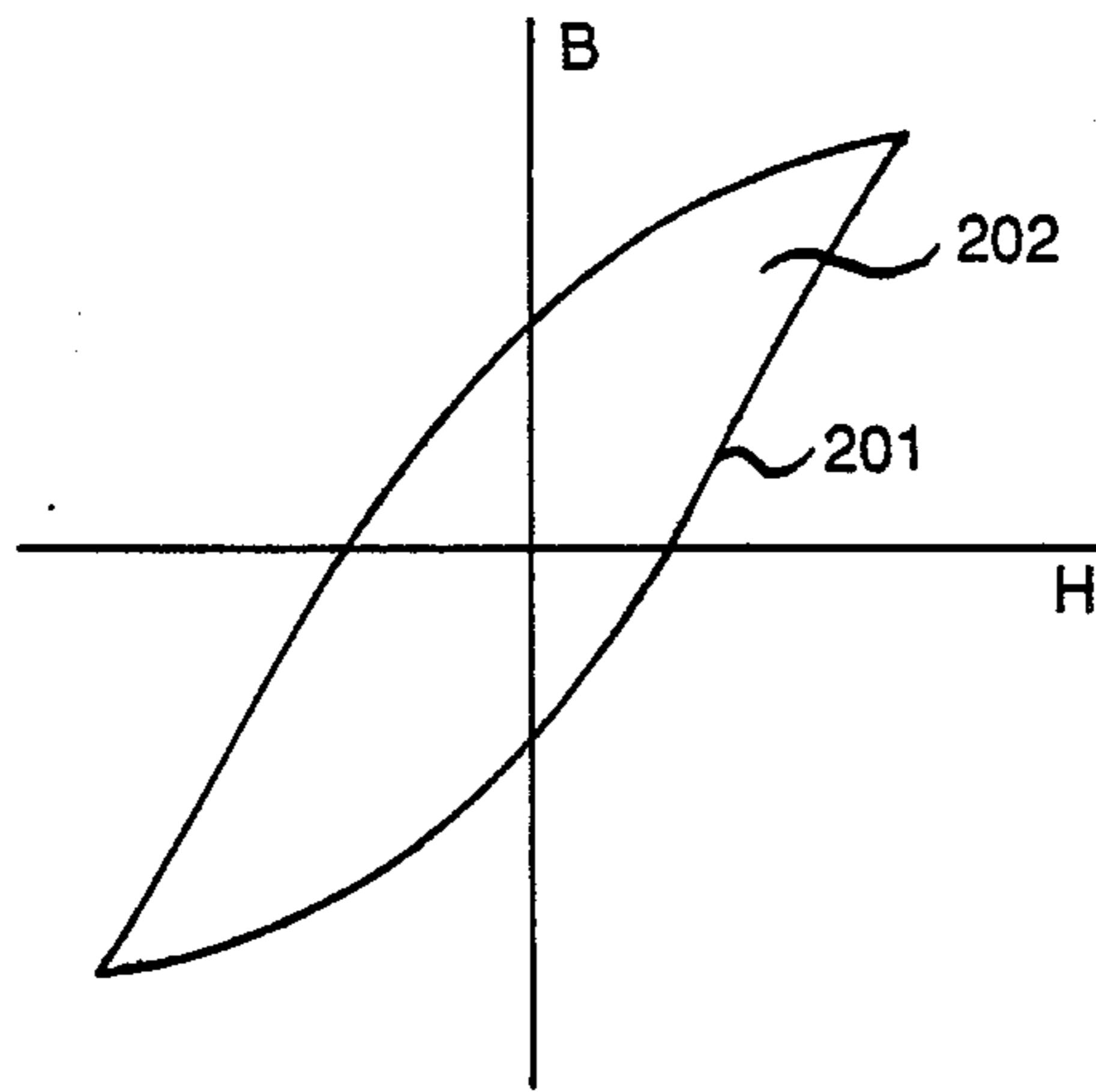
FIG. 2 (PRIOR ART)
