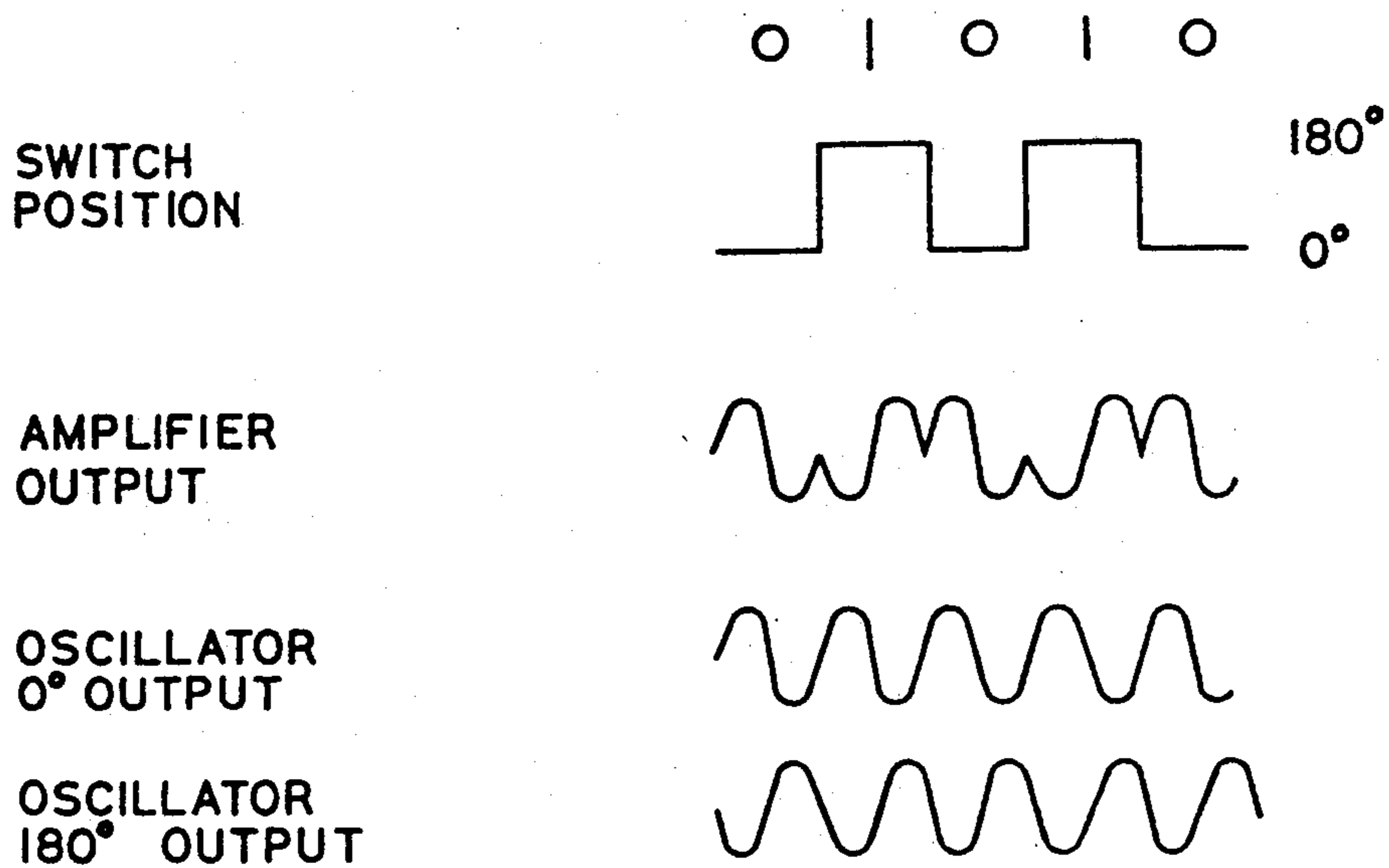
TRANSMITTER WAVEFORMS
