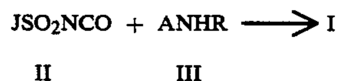
Equation I
