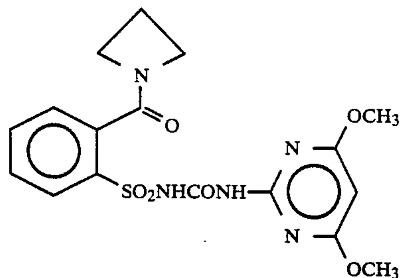
Compound 26
