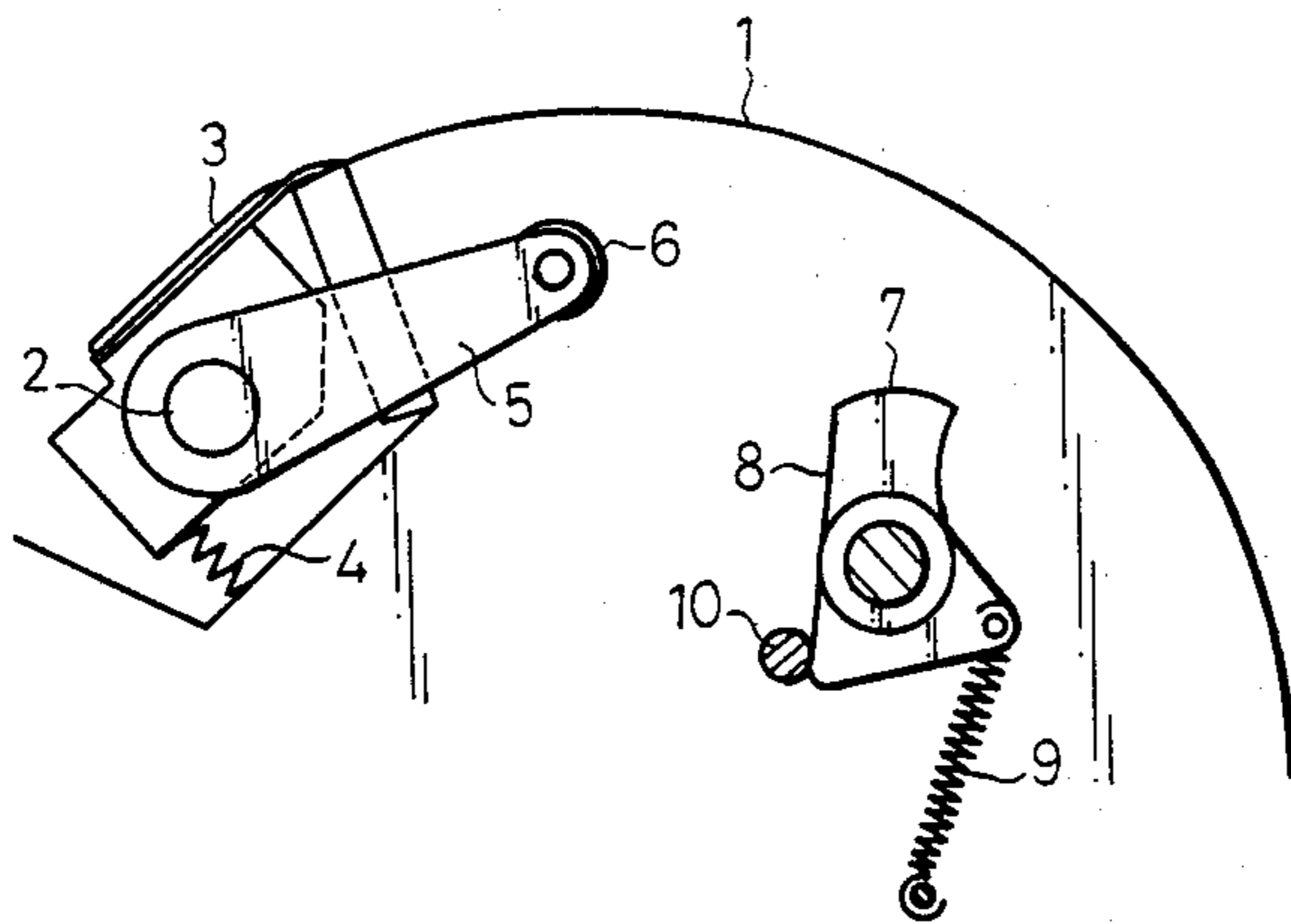
FIG. 9 (PRIOR ART)
