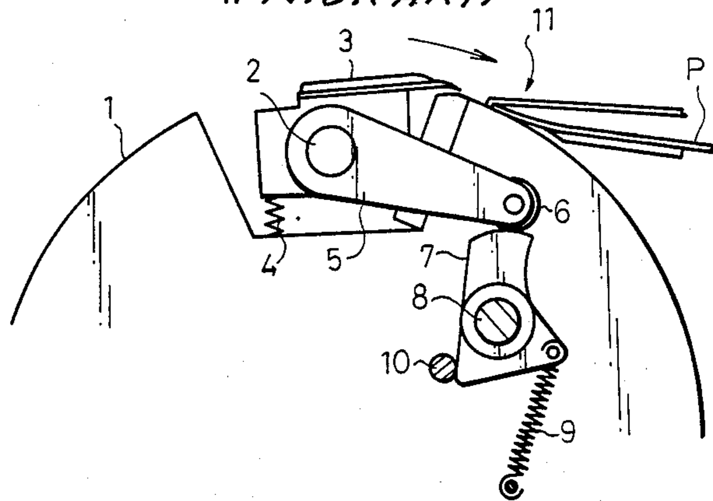
FIG. 10 (PRIOR ART)
