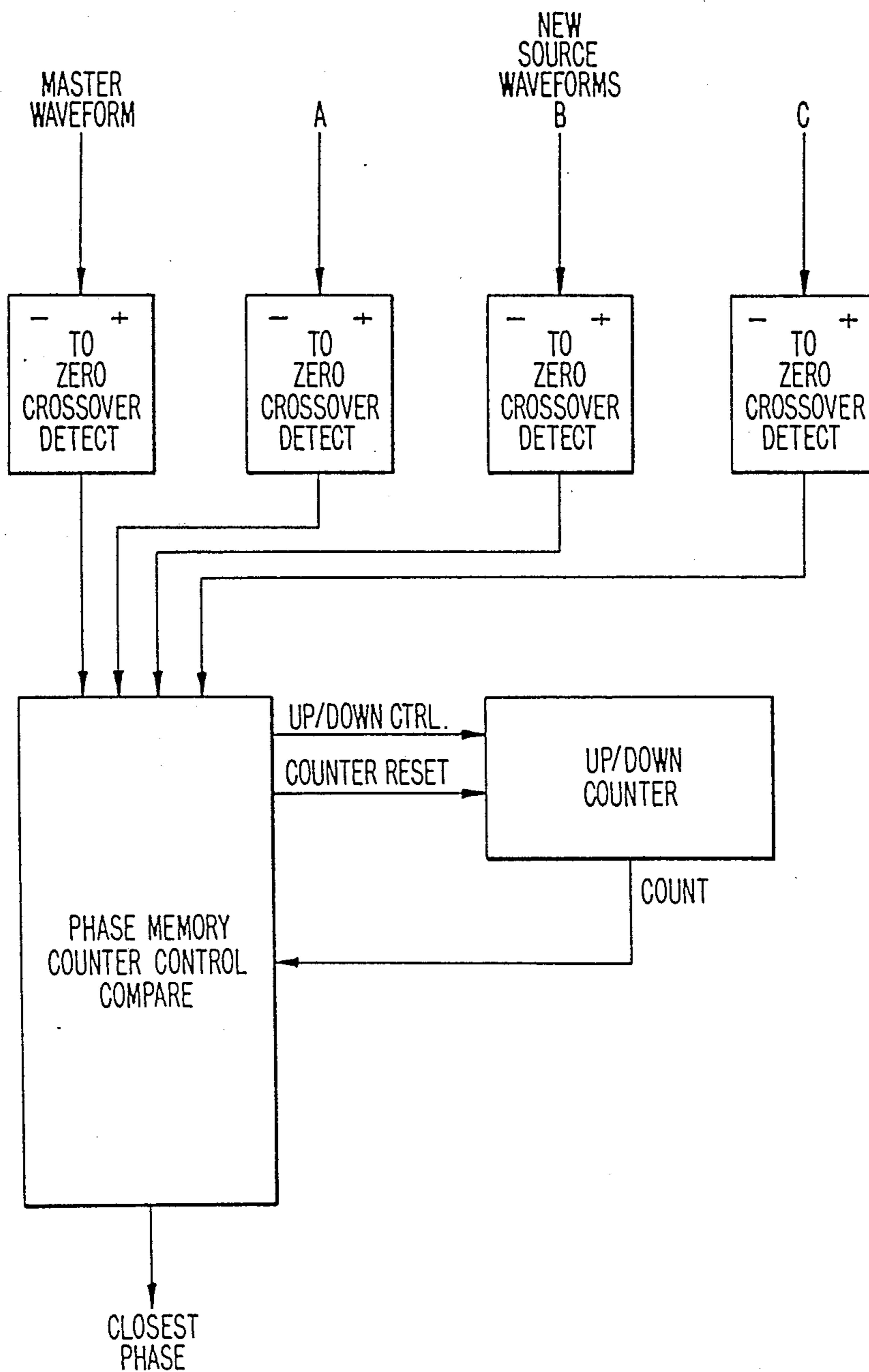
WAVEFORM COINCIDENCE DETECTOR CIRCUIT
