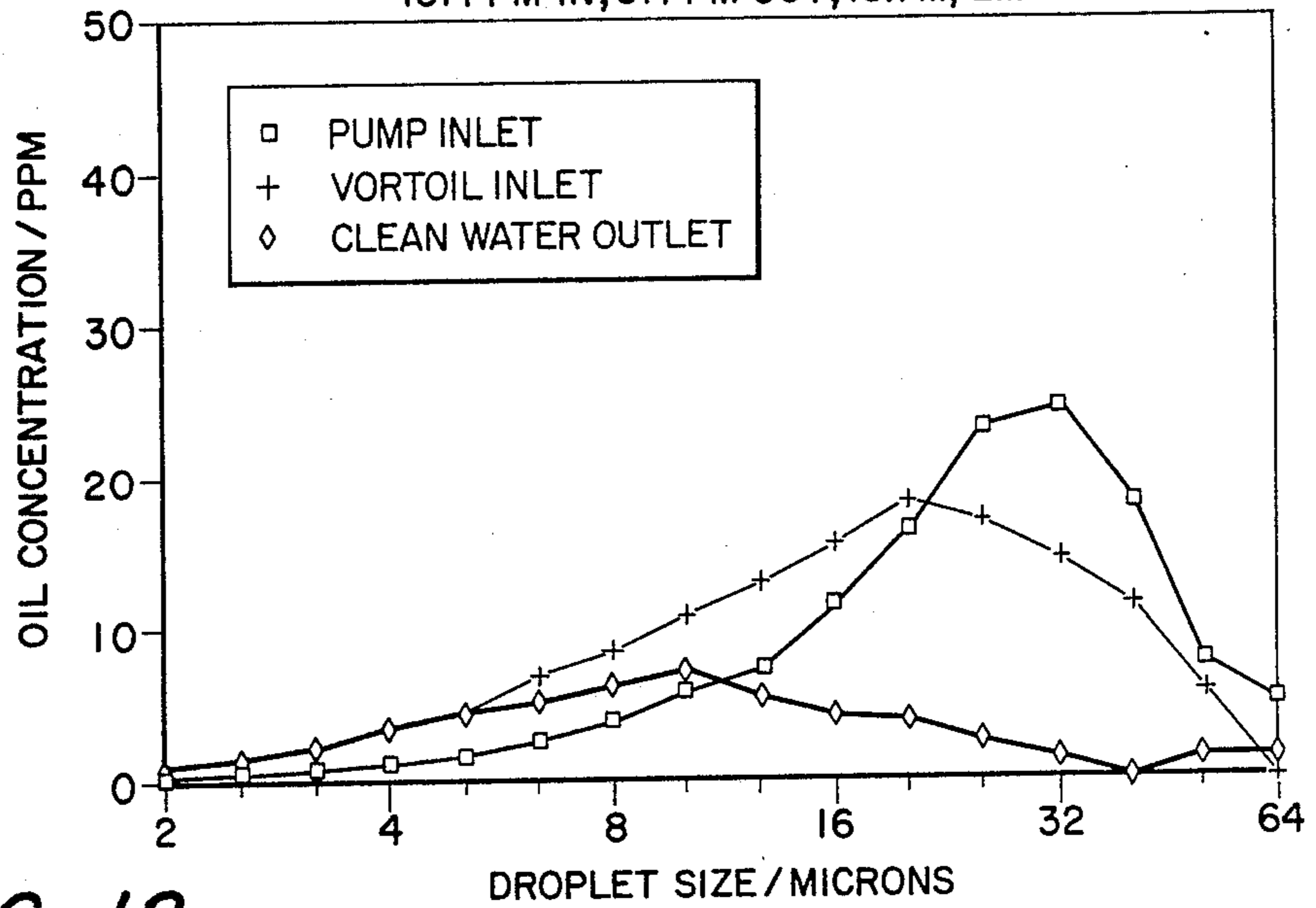
35 MM VORTOIL ® PERFORMANCE BY DROP SIZE 131 PPM IN, 51 PPM OUT, 15.1 M, LM
